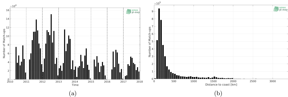
Figure 1: Number of match-ups between TSG (SAMOS) and SMOS SSS L3 v2 - Monthly - 0.25 Deg (CATDS-CECOS-IFREMER) SSS as a function of time (a) and as function of the distance to coast (b) over the Atlantic Ocean Pi-MEP region and for the full satellite product period.
