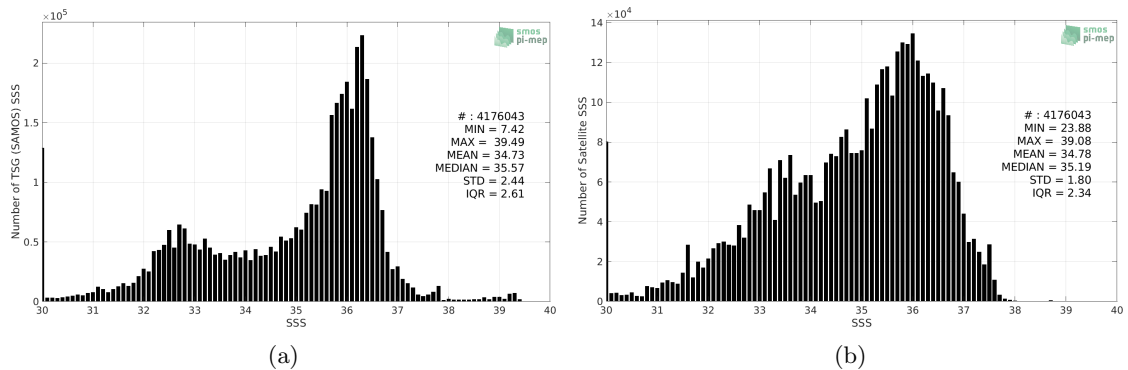
Figure 2: Histograms of SSS from TSG (SAMOS) (a) and SMOS SSS L3 v2 - Monthly - 0.25 Deg (CATDS-CECOS-IFREMER) (b) considering all match-up pairs per bins of 0.1 over the Atlantic Ocean Pi-MEP region and for the full satellite product period.
