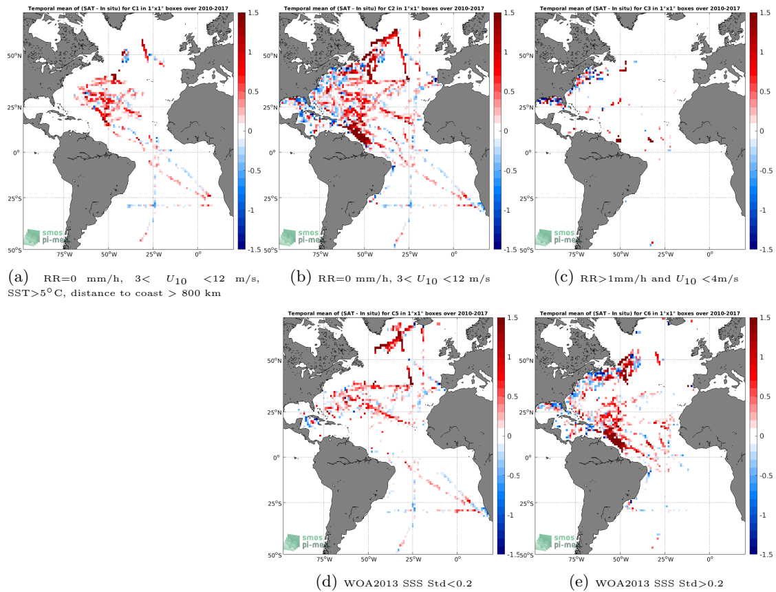
Figure 12: Temporal mean gridded over spatial boxes of size 1^\circ \times 1^\circ of \Delta SSS (SMOS SSS L3 v2 - Monthly - 0.25 Deg (CATDS-CECOS-IFREMER) - TSG (SAMOS)) for 5 different subdatasets corresponding to:RR=0 mm/h, 3 < U_{10} < 12 m/s, SST >5^\circ\text{C} , distance to coast > 800 km (a), RR=0 mm/h, 3 < U_{10} < 12 m/s (b), RR >1 mm/h and U_{10} < 4 m/s (c), WOA2013 SSS Std <0.2 (d), WOA2013 SSS Std >0.2 (e).
