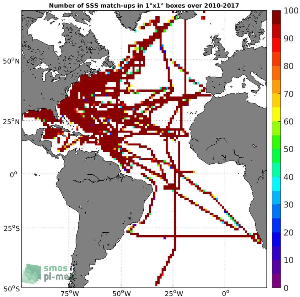
Figure 4: Number of SSS match-ups between TSG (SAMOS) SSS and the SMOS SSS L3 v2 - Monthly - 0.25 Deg (CATDS-CECOS-IFREMER) SSS product for the Atlantic Ocean Pi-MEP region over 1°x1° boxes and for the full satellite product period.
