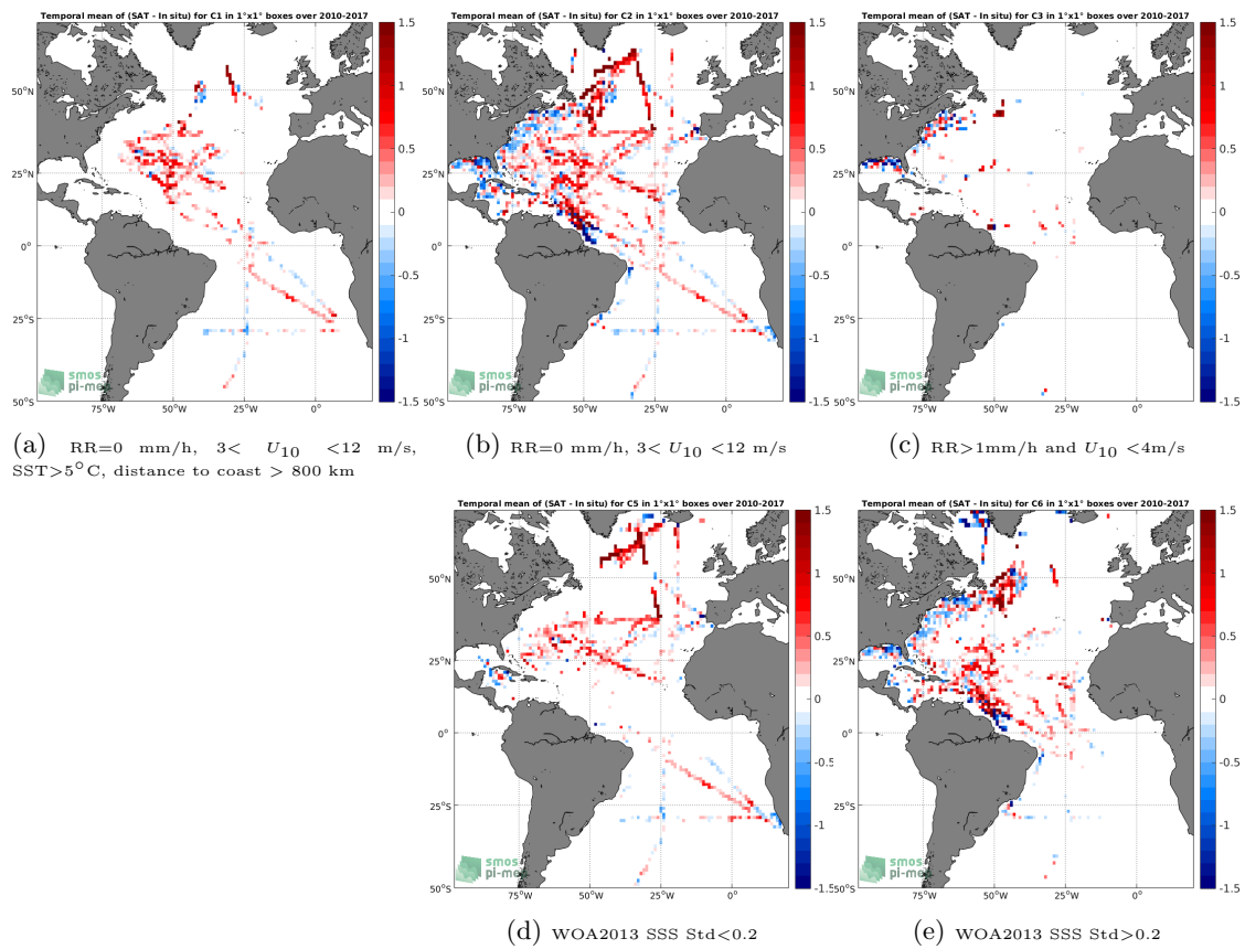
Figure 12: Temporal mean gridded over spatial boxes of size 1^\circ \times 1^\circ of \Delta\text{SSS} (SMOS SSS L3 v2 - Monthly - 0.25 Deg (CATDS-CECOS-IFREMER) - TSG (SAMOS)) for 5 different subdatasets corresponding to:RR=0 mm/h, 3 < U_{10} < 12 m/s, SST >5^\circ\text{C} , distance to coast > 800 km (a), RR=0 mm/h, 3 < U_{10} < 12 m/s (b), RR >1 mm/h and U_{10} < 4 m/s (c), WOA2013 SSS Std <0.2 (d), WOA2013 SSS Std >0.2 (e).
