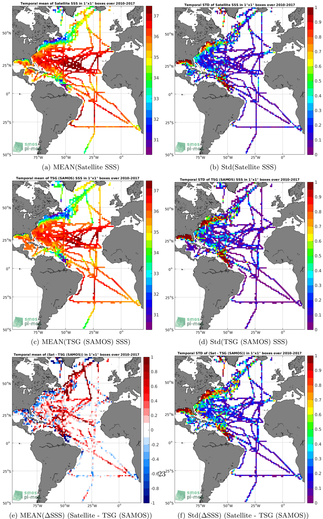
(e) MEAN( \Delta SSS) (Satellite - TSG (SAMOS)) (f) Std( \Delta SSS) (Satellite - TSG (SAMOS)) Figure 6: Temporal mean (left) and Std (right) of SSS from SMOS SSS L3 v2 - Monthly - 0.25 Deg (CATDS-CECOS-IFREMER) (top), TSG (SAMOS) (middle), and of \Delta SSS (Satellite - TSG (SAMOS)). Only match-up pairs are used to generate these maps.
