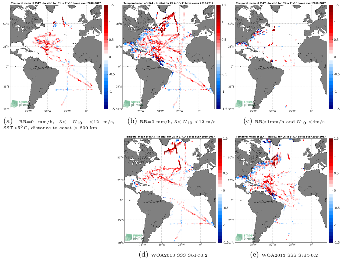
Figure 12: Temporal mean gridded over spatial boxes of size 1^\circ \times 1^\circ of \Delta SSS (SMOS L3 v2 - Monthly - 0.25 Deg (CATDS-CECOS-IFREMER) - TSG-SAMOS) for 5 different subdatasets corresponding to:RR=0 mm/h, 3 < U_{10} < 12 m/s, SST >5^\circ\text{C} , distance to coast > 800 km (a), RR=0 mm/h, 3 < U_{10} < 12 m/s (b), RR >1 mm/h and U_{10} < 4 m/s (c), WOA2013 SSS Std <0.2 (d), WOA2013 SSS Std >0.2 (e).
