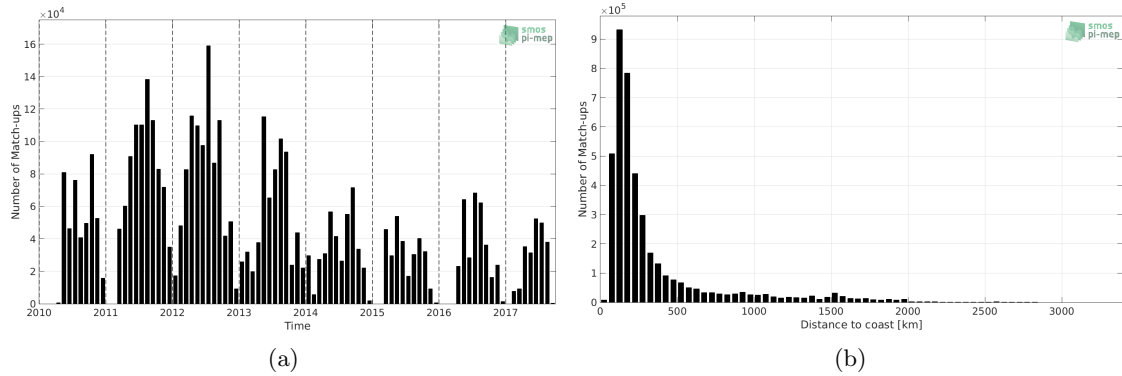
Figure 1: Number of match-ups between TSG-SAMOS and SMOS L3 v2 - Monthly - 0.25 Deg (CATDS-CECOS-IFREMER) SSS as a function of time (a) and as function of the distance to coast (b) over the Atlantic Ocean Pi-MEP region and for the full satellite product period.
