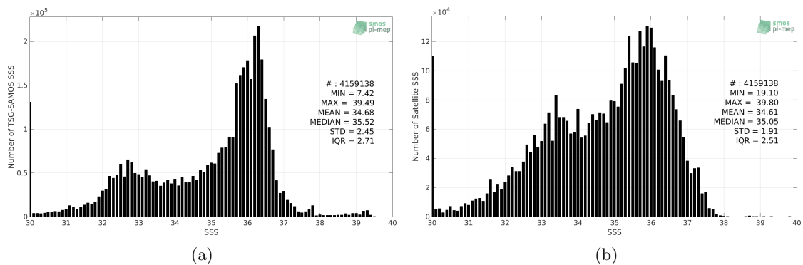
Figure 2: Histograms of SSS from TSG-SAMOS (a) and SMOS L3 v2 - Monthly - 0.25 Deg (CATDS-CECOS-IFREMER) (b) considering all match-up pairs per bins of 0.1 over the Atlantic Ocean Pi-MEP region and for the full satellite product period.
