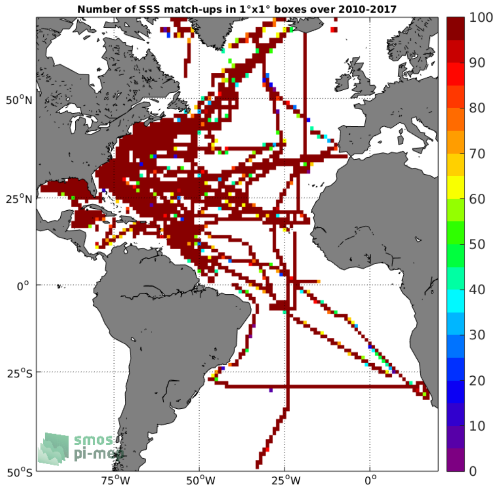
Figure 4: Number of SSS match-ups between TSG-SAMOS SSS and the SMOS L3 v2 - Monthly - 0.25 Deg (CATDS-CECOS-IFREMER) SSS product for the Atlantic Ocean Pi-MEP region over 1°x1° boxes and for the full satellite product period.
