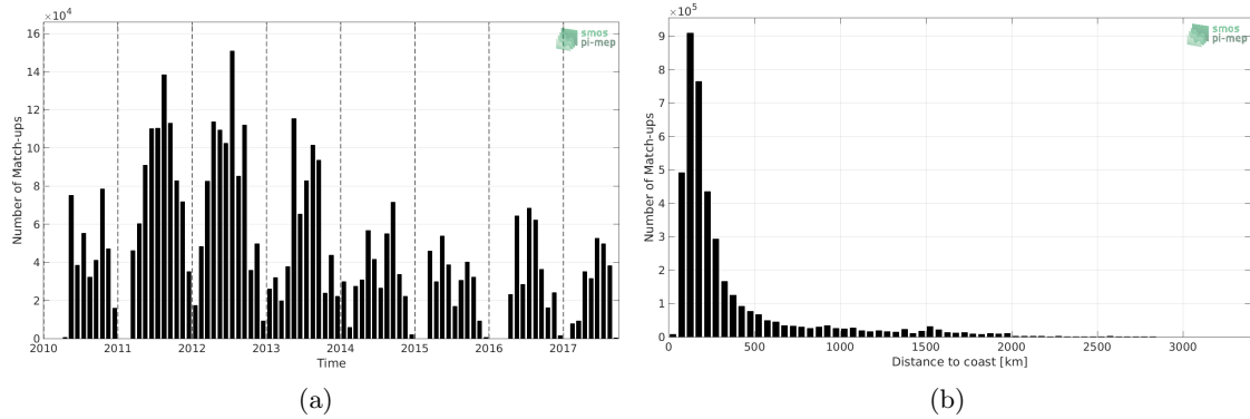
Figure 1: Number of match-ups between TSG-SAMOS and SMOS-L3-CATDS-IFREMER-CECOS-V2-MONTHLY-0.25DEG SSS as a function of time (a) and as function of the distance to coast (b) over the Atlantic Ocean Pi-MEP region and for the full satellite product period.
