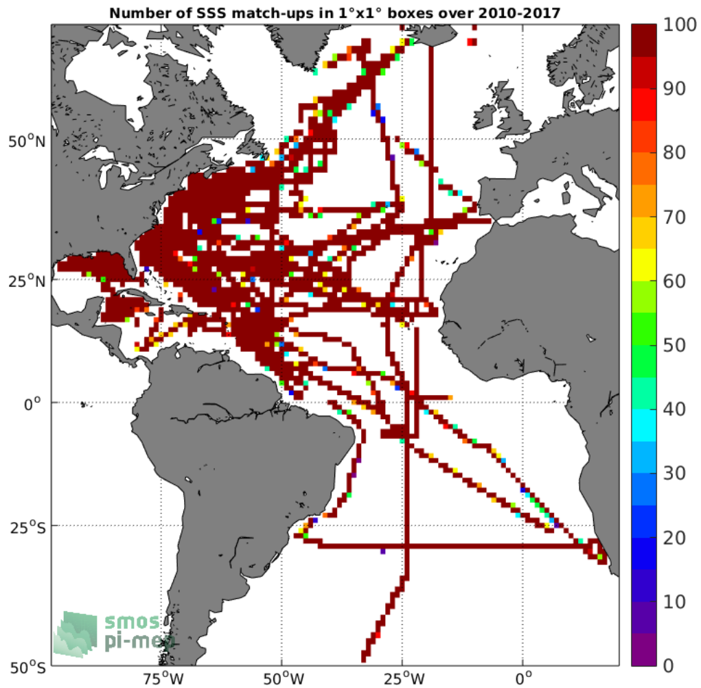
Figure 4: Number of SSS match-ups between TSG-SAMOS SSS and the SMOS-L3-CATDS-IFREMER-CECOS-V2-MONTHLY-0.25DEG SSS product for the Atlantic Ocean Pi-MEP region over 1°x1° boxes and for the full satellite product period.
