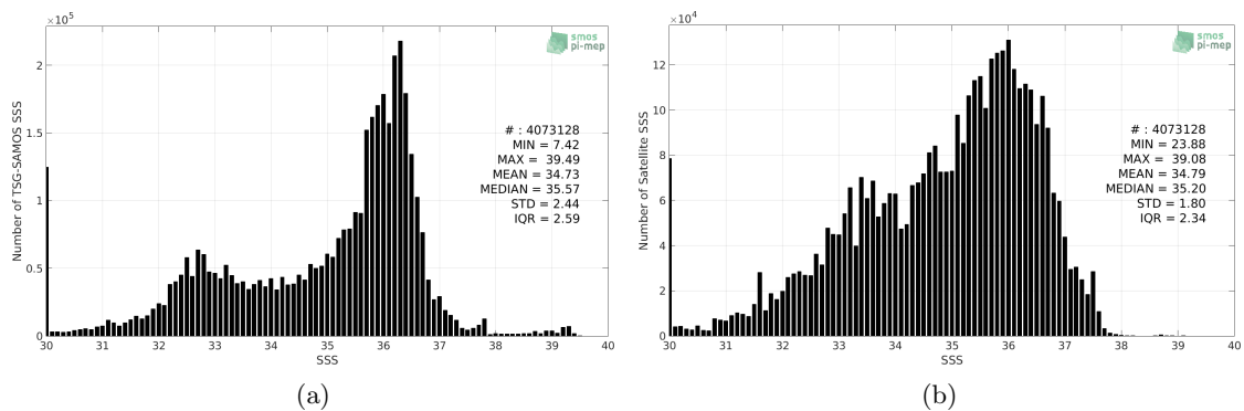
Figure 2: Histograms of SSS from TSG-SAMOS (a) and SMOS-L3-CATDS-IFREMER-CECOS-V2-MONTHLY-0.25DEG (b) considering all match-up pairs per bins of 0.1 over the Atlantic Ocean Pi-MEP region and for the full satellite product period.
