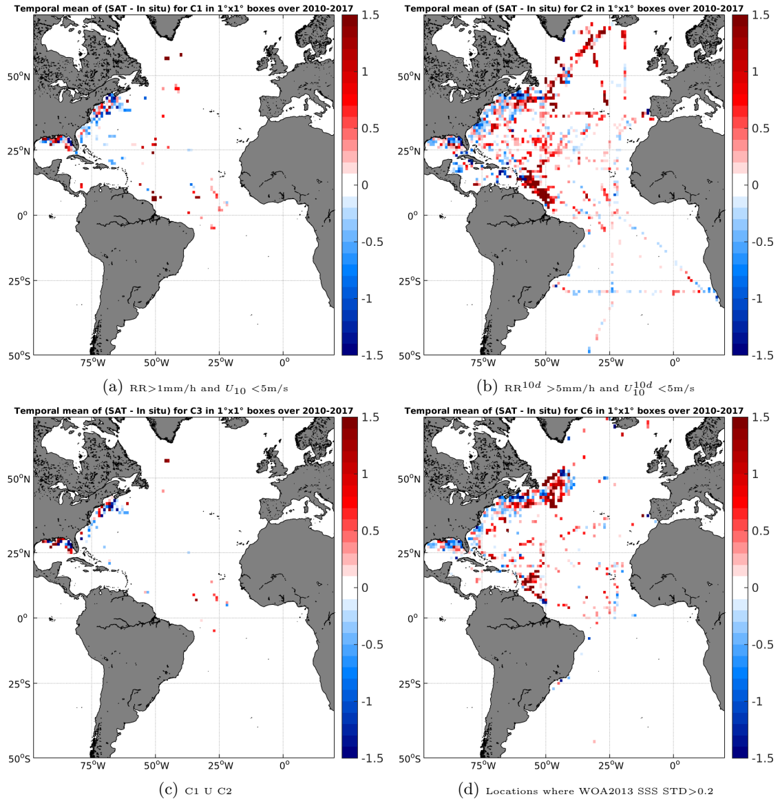
Figure 12: Temporal mean gridded over spatial boxes of size 1^\circ \times 1^\circ of \Delta SSS (SMOS-L3-CATDS-IFREMER-CECOS-V2-MONTHLY-0.25DEG - TSG-SAMOS) for 4 different subdatasets corresponding to:RR >1 mm/h and U_{10} < 5 m/s (a), RR 10d > 5 mm/h and U_{10}^{10d} < 5 m/s (b), C1 U C2 (c),Locations where WOA2013 SSS STD >0.2 (d).
