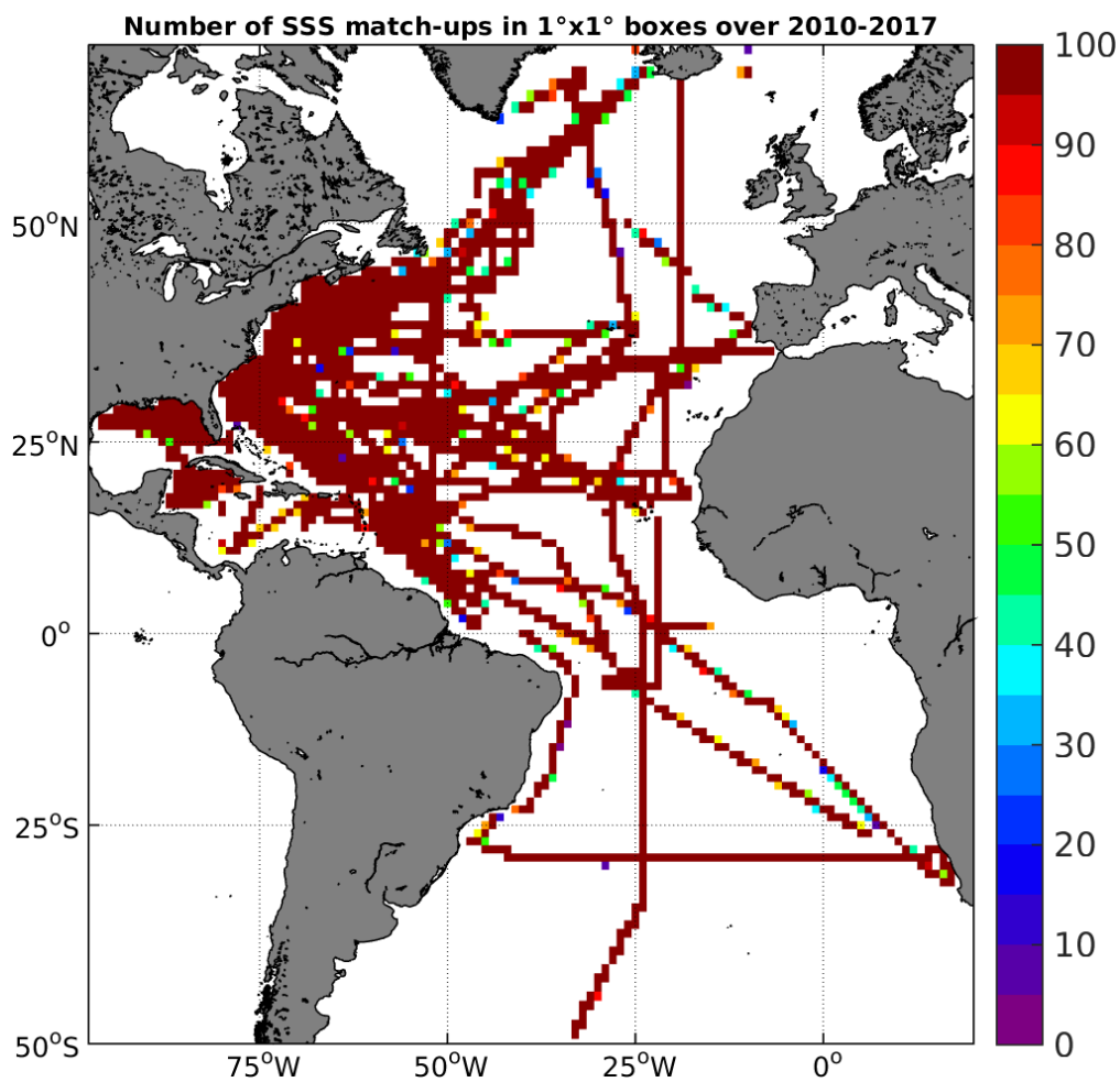
Figure 4: Number of SSS match-ups between TSG-SAMOS SSS and the SMOS-L3-CATDS-IFREMER-CECOS-V2-MONTHLY-0.25DEG SSS product for the Atlantic Ocean Pi-MEP region over 1°x1° boxes and for the full satellite product period.
