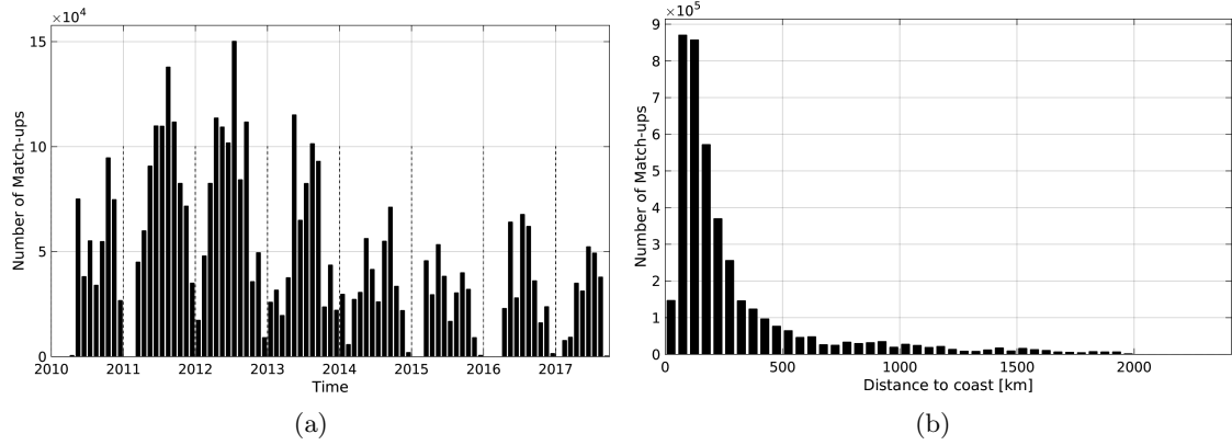
Figure 1: Number of match-ups between TSG-SAMOS and SMOS-L3-CATDS-IFREMER-CECOS-V2-MONTHLY-0.25DEG SSS as a function of time (a) and as function of the distance to coast (b) over the Atlantic Ocean Pi-MEP region and for the full satellite product period.
