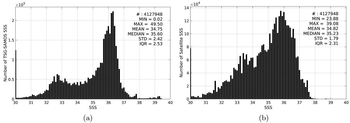
Figure 2: Histograms of SSS from TSG-SAMOS (a) and SMOS-L3-CATDS-IFREMER-CECOS-V2-MONTHLY-0.25DEG (b) considering all match-up pairs per bins of 0.1 over the Atlantic Ocean Pi-MEP region and for the full satellite product period.
