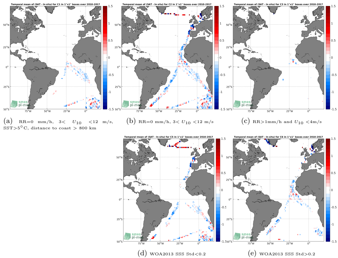
Figure 12: Temporal mean gridded over spatial boxes of size 1^\circ \times 1^\circ of \Delta\text{SSS} (SMOS SSS L3 v2 - Monthly - 0.25 Deg (CATDS-CECOS-IFREMER) - TSG (Polarstern)) for 5 different subdatasets corresponding to:RR=0 mm/h, 3 < U_{10} < 12 m/s, SST >5^\circ\text{C} , distance to coast > 800 km (a), RR=0 mm/h, 3 < U_{10} < 12 m/s (b), RR >1 mm/h and U_{10} < 4 m/s (c), WOA2013 SSS Std <0.2 (d), WOA2013 SSS Std >0.2 (e).
