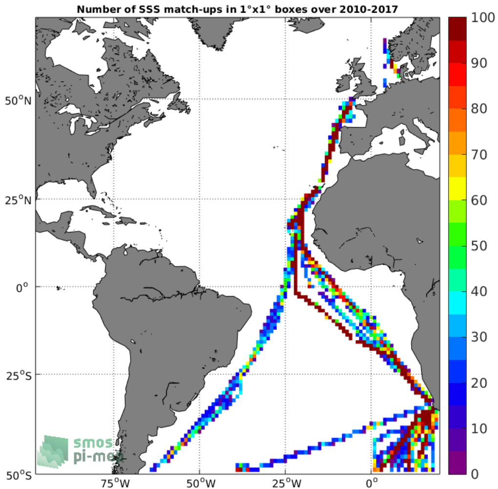
Figure 4: Number of SSS match-ups between TSG-POLARSTERN SSS and the SMOS-L3-CATDS-IFREMER-CECOS-V2-MONTHLY-0.25DEG SSS product for the Atlantic Ocean Pi-MEP region over 1°x1° boxes and for the full satellite product period.
