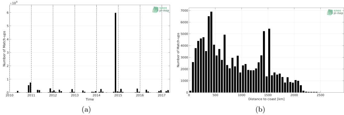
Figure 1: Number of match-ups between TSG-POLARSTERN and SMOS-L3-CATDS-IFREMER-CECOS-V2-MONTHLY-0.25DEG SSS as a function of time (a) and as function of the distance to coast (b) over the Atlantic Ocean Pi-MEP region and for the full satellite product period.
