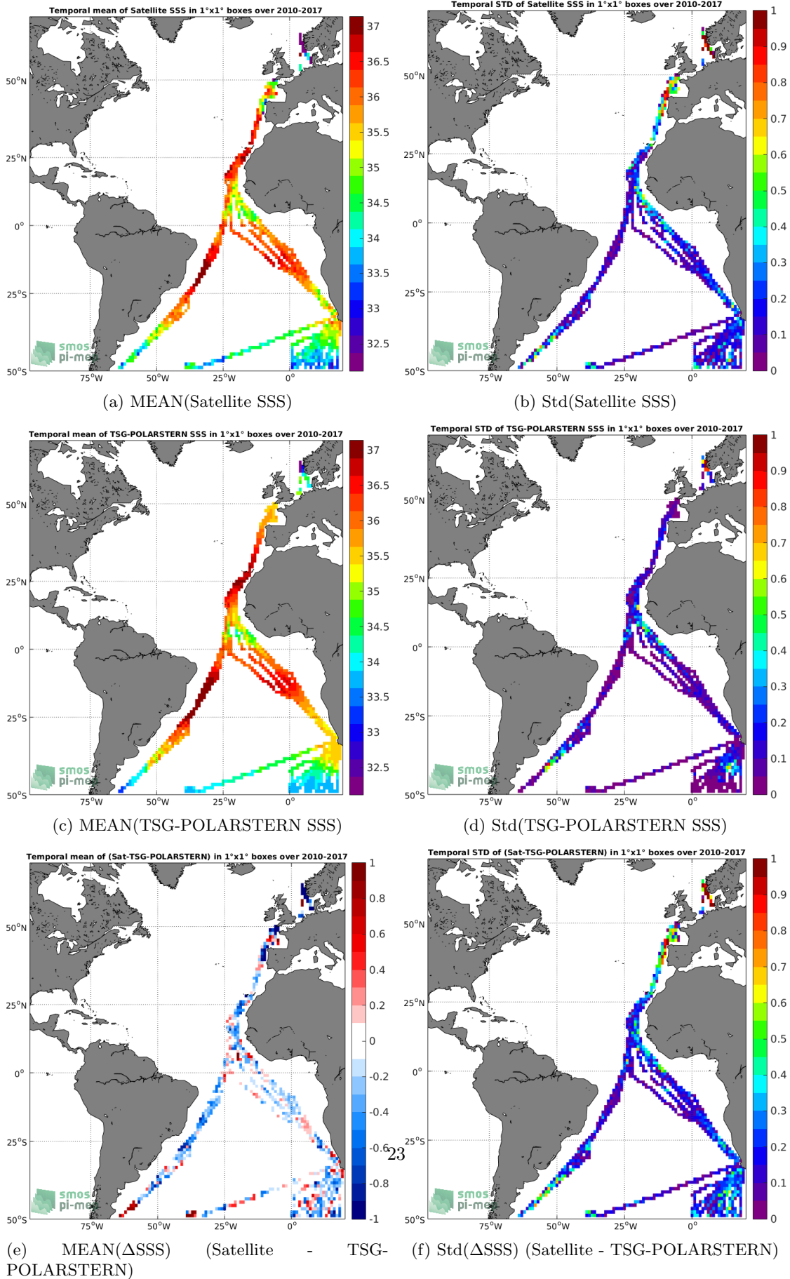
Figure 6: Temporal mean (left) and Std (right) of SSS from SMOS-L3-CATDS-IFREMER-CECOS-V2-MONTHLY-0.25DEG (top), TSG-POLARSTERN (middle), and of \Delta SSS (Satellite - TSG-POLARSTERN). Only match-up pairs are used to generate these maps.
