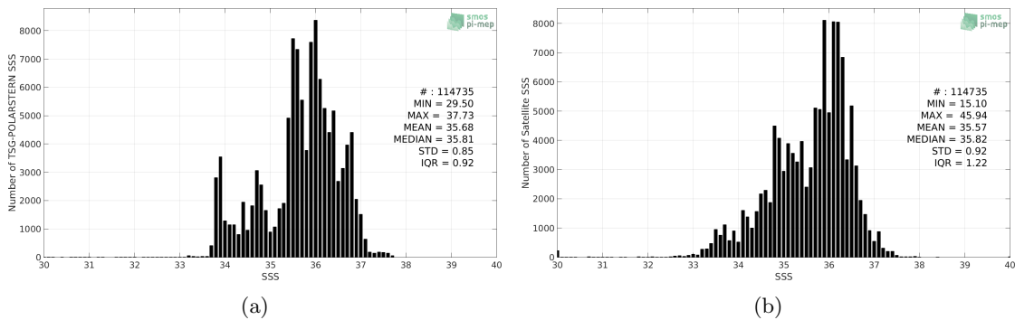
Figure 2: Histograms of SSS from TSG-POLARSTERN (a) and SMOS-L3-CATDS-IFREMER-CECOS-V2-MONTHLY-0.25DEG (b) considering all match-up pairs per bins of 0.1 over the Atlantic Ocean Pi-MEP region and for the full satellite product period.
