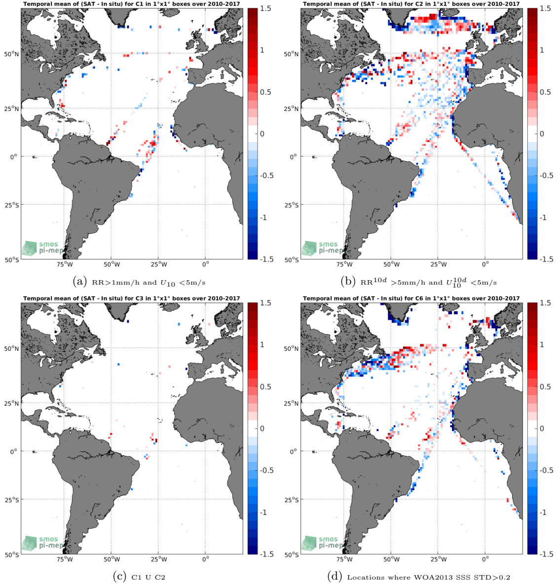
Figure 12: Temporal mean gridded over spatial boxes of size 1^\circ \times 1^\circ of \Delta SSS (SMOS-L3-CATDS-IFREMER-CECOS-V2-MONTHLY-0.25DEG - TSG-LEGOS-DM) for 4 different subdatasets corresponding to: RR > 1mm/h and U_{10} < 5\text{m/s} (a), RR^{10d} > 5\text{mm/h} and U_{10}^{10d} < 5\text{m/s} (b), C1 U C2 (c), Locations where WOA2013 SSS STD > 0.2 (d).
