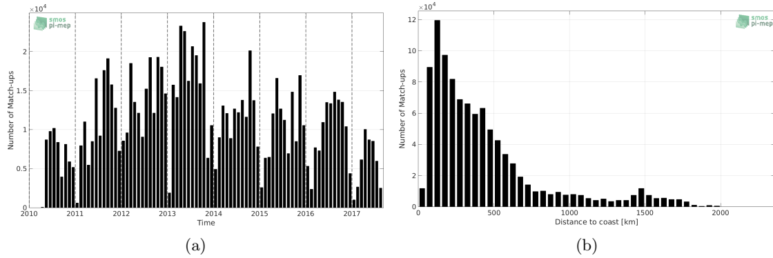
Figure 1: Number of match-ups between TSG-LEGOS-DM and SMOS-L3-CATDS-IFREMER-CECOS-V2-MONTHLY-0.25DEG SSS as a function of time (a) and as function of the distance to coast (b) over the Atlantic Ocean Pi-MEP region and for the full satellite product period.
