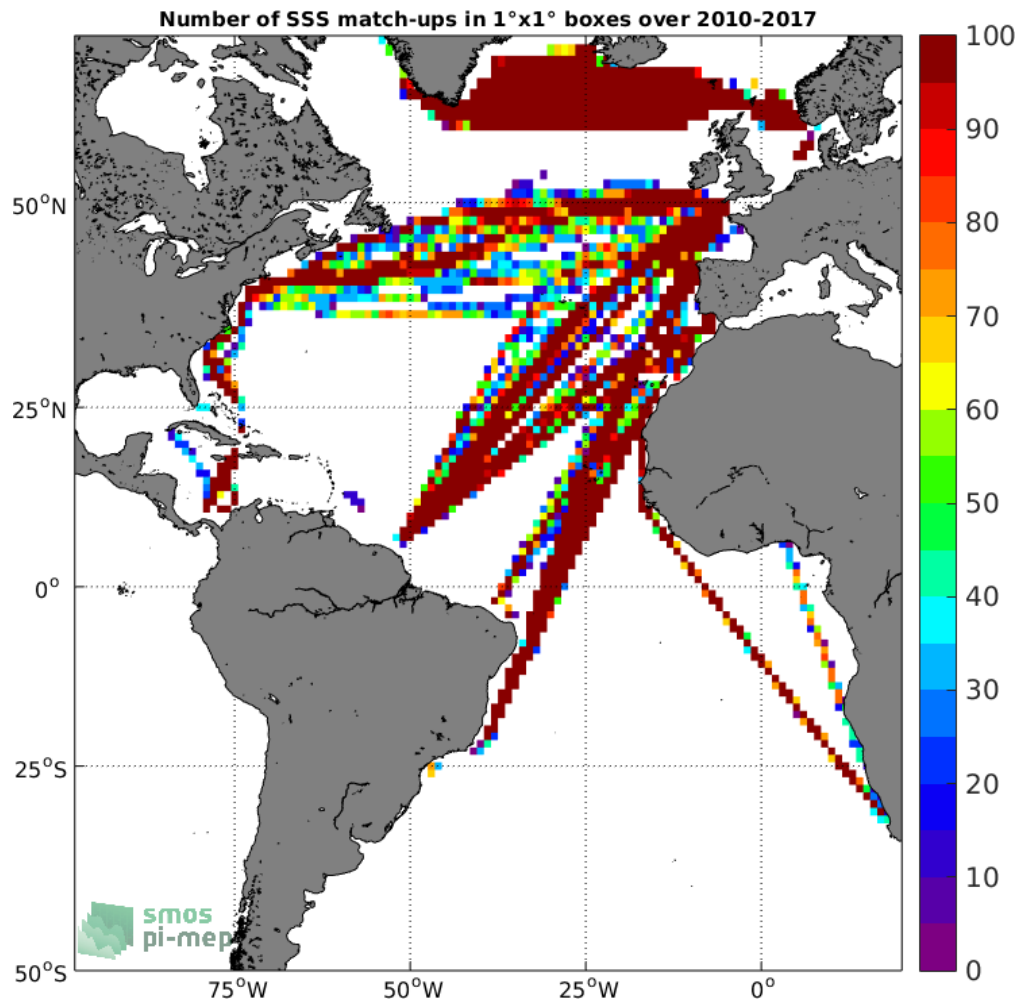
Figure 4: Number of SSS match-ups between TSG-LEGOS-DM SSS and the SMOS-L3-CATDS-IFREMER-CECOS-V2-MONTHLY-0.25DEG SSS product for the Atlantic Ocean Pi-MEP region over 1°x1° boxes and for the full satellite product period.
