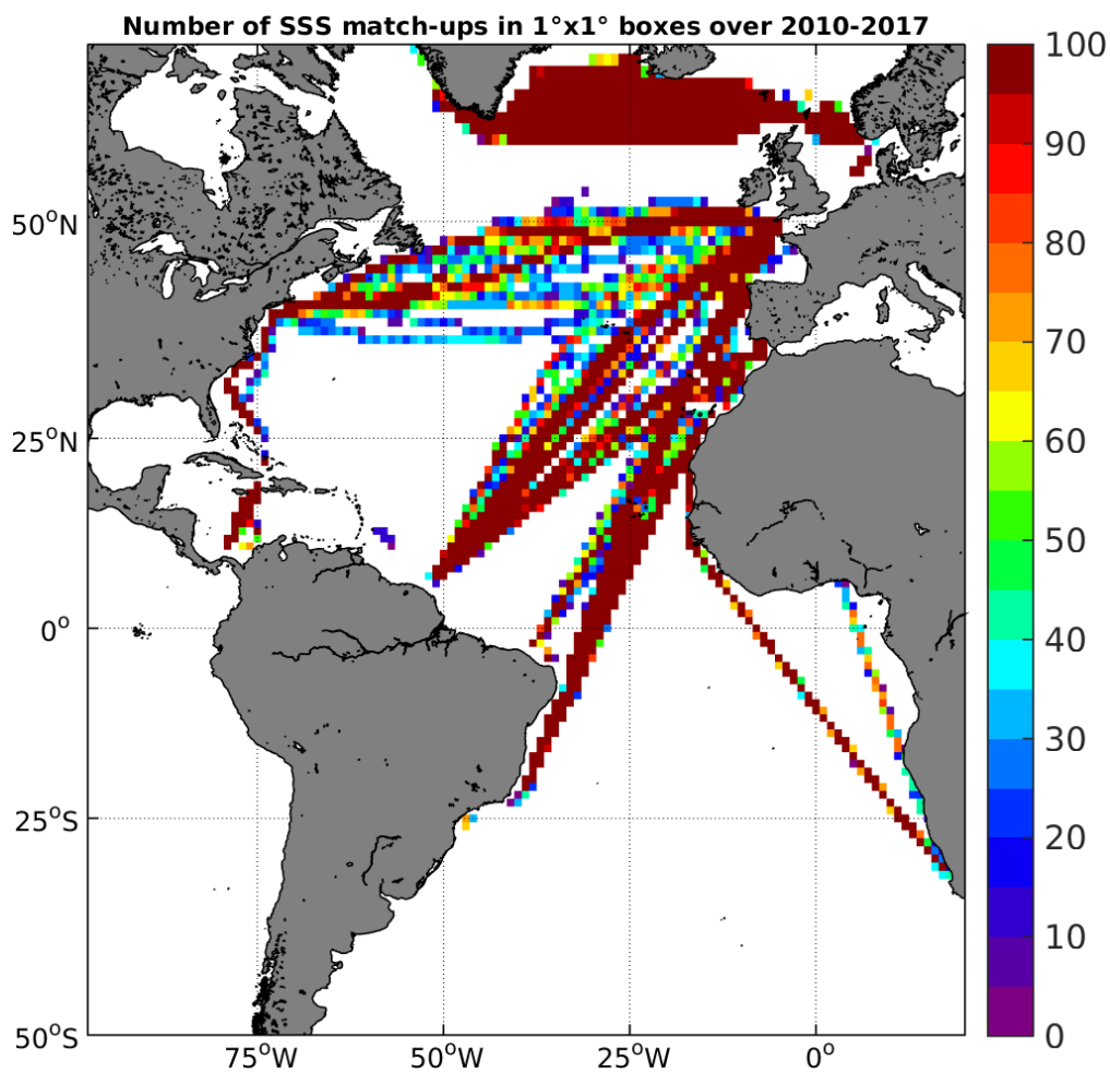
Figure 4: Number of SSS match-ups between TSG-LEGOS-DM SSS and the SMOS-L3-CATDS-IFREMER-CECOS-V2-MONTHLY-0.25DEG SSS product for the Atlantic Ocean Pi-MEP region over 1°x1° boxes and for the full satellite product period.
