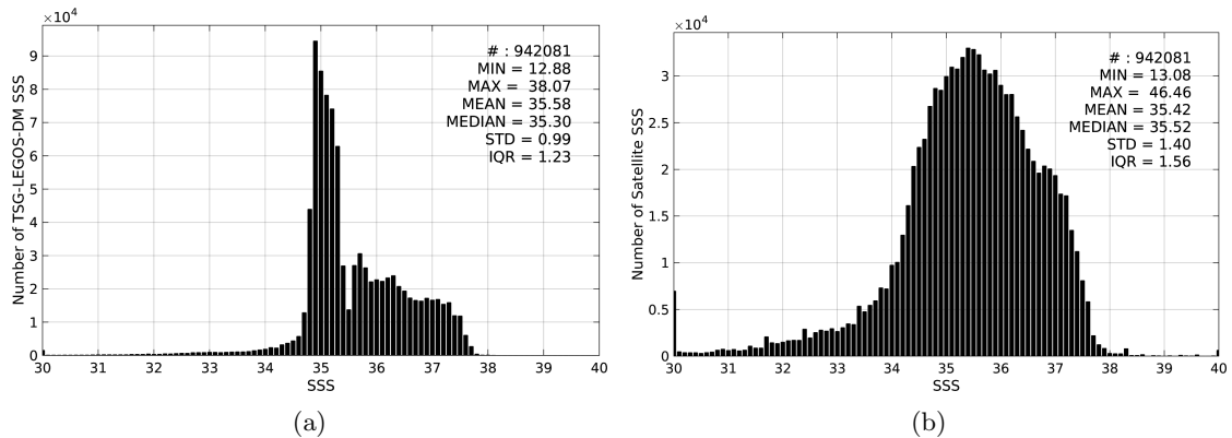
Figure 2: Histograms of SSS from TSG-LEGOS-DM (a) and SMOS-L3-CATDS-IFREMER-CECOS-V2-MONTHLY-0.25DEG (b) considering all match-up pairs per bins of 0.1 over the Atlantic Ocean Pi-MEP region and for the full satellite product period.
