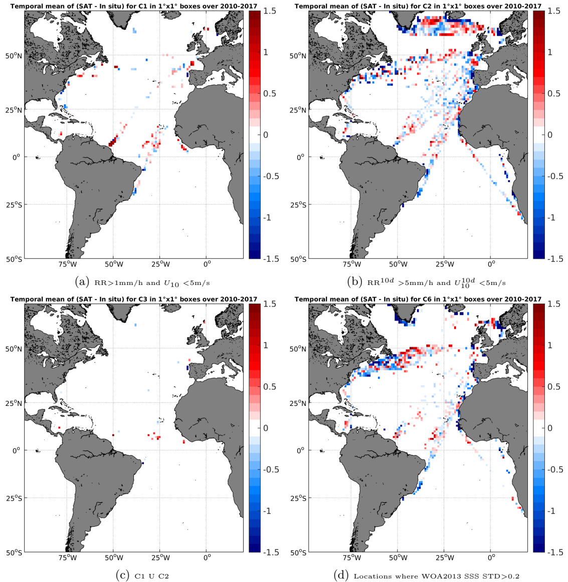
Figure 12: Temporal mean gridded over spatial boxes of size 1^\circ \times 1^\circ of \Delta SSS (SMOS-L3-CATDS-IFREMER-CECOS-V2-MONTHLY-0.25DEG - TSG-LEGOS-DM) for 4 different subdatasets corresponding to: RR > 1mm/h and U_{10} < 5 m/s (a), RR^{10d} > 5 mm/h and U_{10}^{10d} < 5 m/s (b), C1 U C2 (c), Locations where WOA2013 SSS STD > 0.2 (d).
