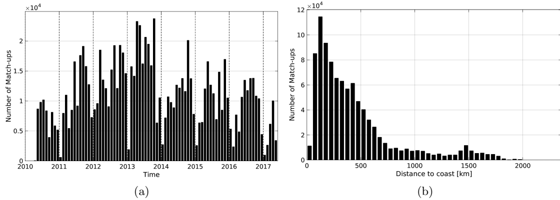
Figure 1: Number of match-ups between TSG-LEGOS-DM and SMOS-L3-CATDS-IFREMER-CECOS-V2-MONTHLY-0.25DEG SSS as a function of time (a) and as function of the distance to coast (b) over the Atlantic Ocean Pi-MEP region and for the full satellite product period.
