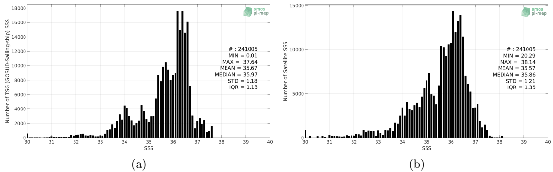
Figure 2: Histograms of SSS from TSG (GOSUD-Sailing-ship) (a) and SMOS SSS L3 v2 - Monthly - 0.25 Deg (CATDS-CECOS-IFREMER) (b) considering all match-up pairs per bins of 0.1 over the Atlantic Ocean Pi-MEP region and for the full satellite product period.
