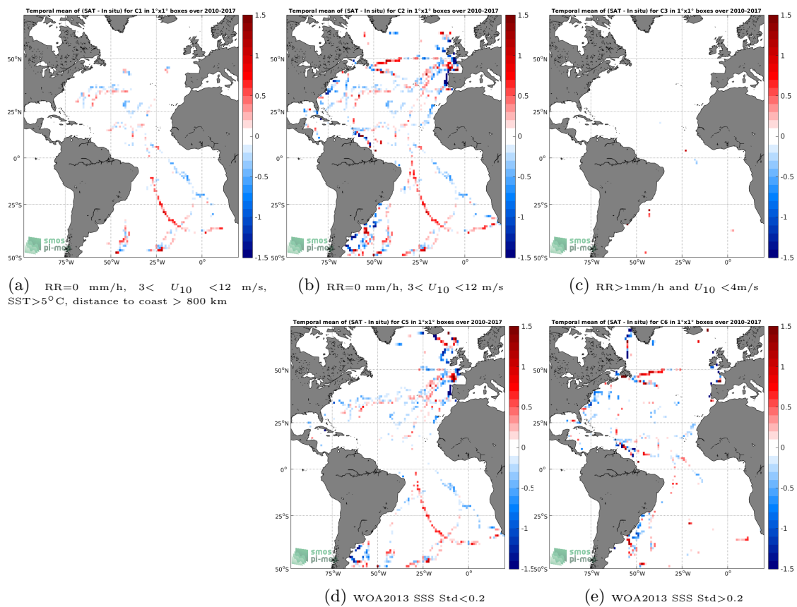
Figure 12: Temporal mean gridded over spatial boxes of size 1^\circ \times 1^\circ of \Delta\text{SSS} (SMOS SSS L3 v2 - Monthly - 0.25 Deg (CATDS-CECOS-IFREMER) - TSG (GOSUD-Sailing-ship)) for 5 different subdatasets corresponding to:RR=0 mm/h, 3 < U_{10} < 12 m/s, SST>5°C, distance to coast > 800 km (a), RR=0 mm/h, 3 < U_{10} < 12 m/s (b), RR>1mm/h and U_{10} < 4 m/s (c), WOA2013 SSS Std<0.2 (d), WOA2013 SSS Std>0.2 (e).
