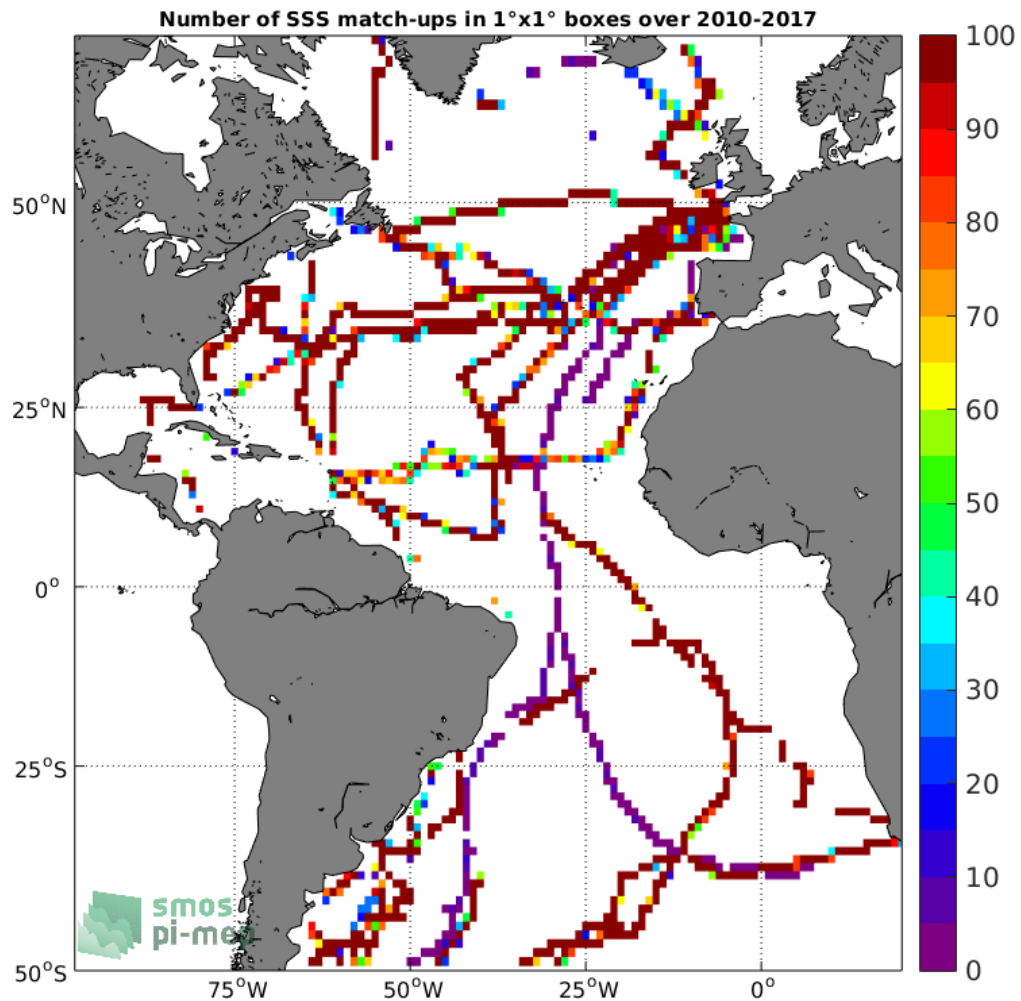
Figure 4: Number of SSS match-ups between TSG-GOSUD-Sailing-ship SSS and the SMOS L3 v2 - Monthly - 0.25 Deg (CATDS-CECOS-IFREMER) SSS product for the Atlantic Ocean Pi-MEP region over 1°x1° boxes and for the full satellite product period.
