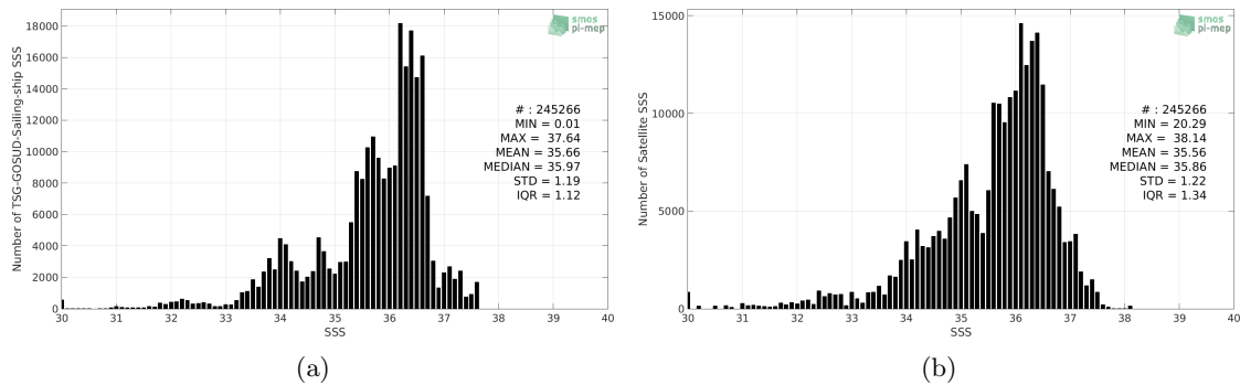
Figure 2: Histograms of SSS from TSG-GOSUD-Sailing-ship (a) and SMOS L3 v2 - Monthly - 0.25 Deg (CATDS-CECOS-IFREMER) (b) considering all match-up pairs per bins of 0.1 over the Atlantic Ocean Pi-MEP region and for the full satellite product period.
