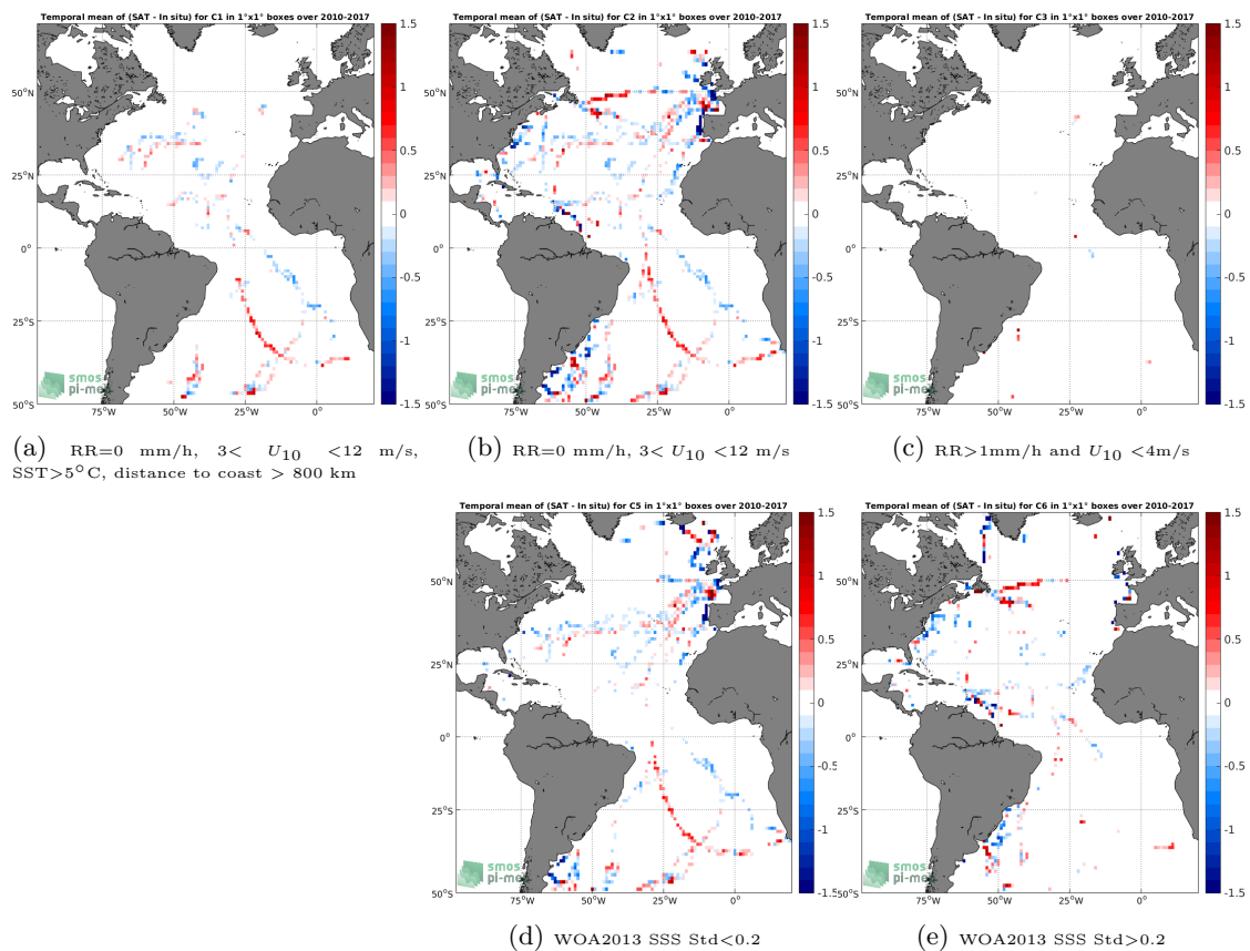
Figure 12: Temporal mean gridded over spatial boxes of size 1^\circ \times 1^\circ of \Delta\text{SSS} (SMOS L3 v2 - Monthly - 0.25 Deg (CATDS-CECOS-IFREMER) - TSG-GOSUD-Sailing-ship) for 5 different subdatasets corresponding to:RR=0 mm/h, 3 < U_{10} < 12 m/s, SST>5°C, distance to coast > 800 km (a), RR=0 mm/h, 3 < U_{10} < 12 m/s (b), RR>1mm/h and U_{10} < 4 m/s (c), WOA2013 SSS Std<0.2 (d), WOA2013 SSS Std>0.2 (e).
