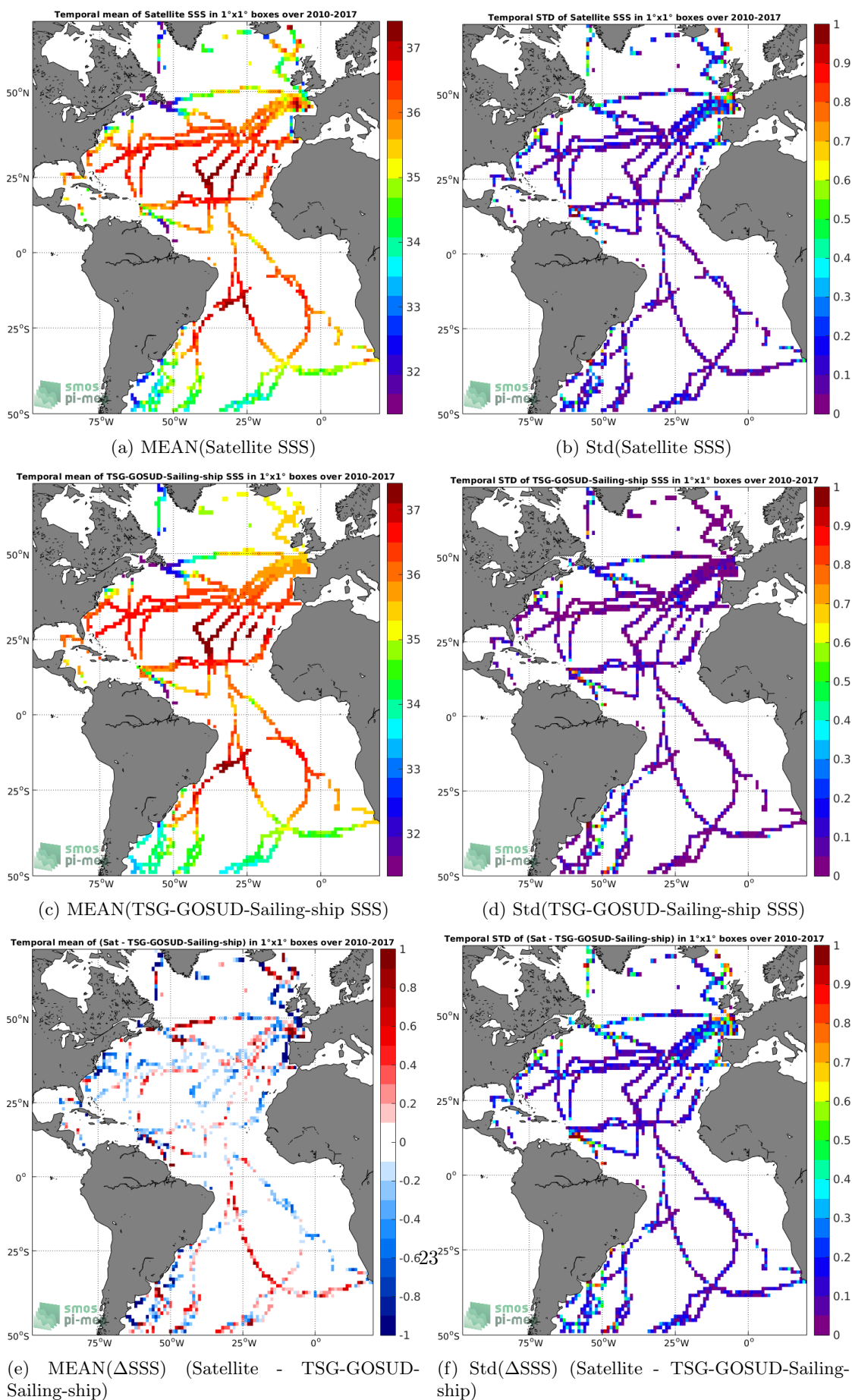
Figure 6: Temporal mean (left) and Std (right) of SSS from SMOS L3 v2 - Monthly - 0.25 Deg (CATDS-CECOS-IFREMER) (top), TSG-GOSUD-Sailing-ship (middle), and of \Delta SSS (Satellite - TSG-GOSUD-Sailing-ship). Only match-up pairs are used to generate these maps.
