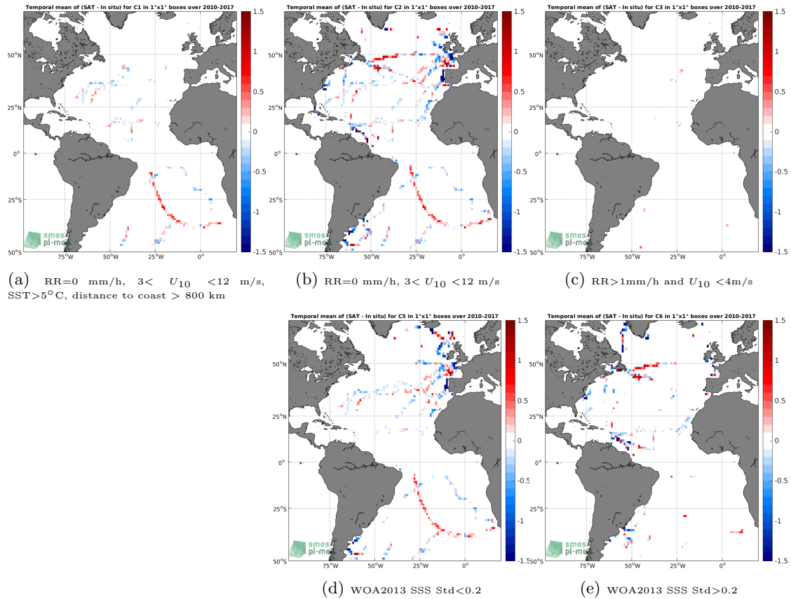
Figure 12: Temporal mean gridded over spatial boxes of size 1^\circ \times 1^\circ of \Delta SSS (SMOS-L3-CATDS-IFREMER-CECOS-V2-MONTHLY-0.25DEG - TSG-GOSUD-Sailing-ship) for 5 different sub-datasets corresponding to:RR=0 mm/h, 3 < U_{10} < 12 m/s, SST >5^\circ C, distance to coast > 800 km (a), RR=0 mm/h, 3 < U_{10} < 12 m/s (b), RR >1 mm/h and U_{10} < 4 m/s (c), WOA2013 SSS Std <0.2 (d), WOA2013 SSS Std >0.2 (e).
