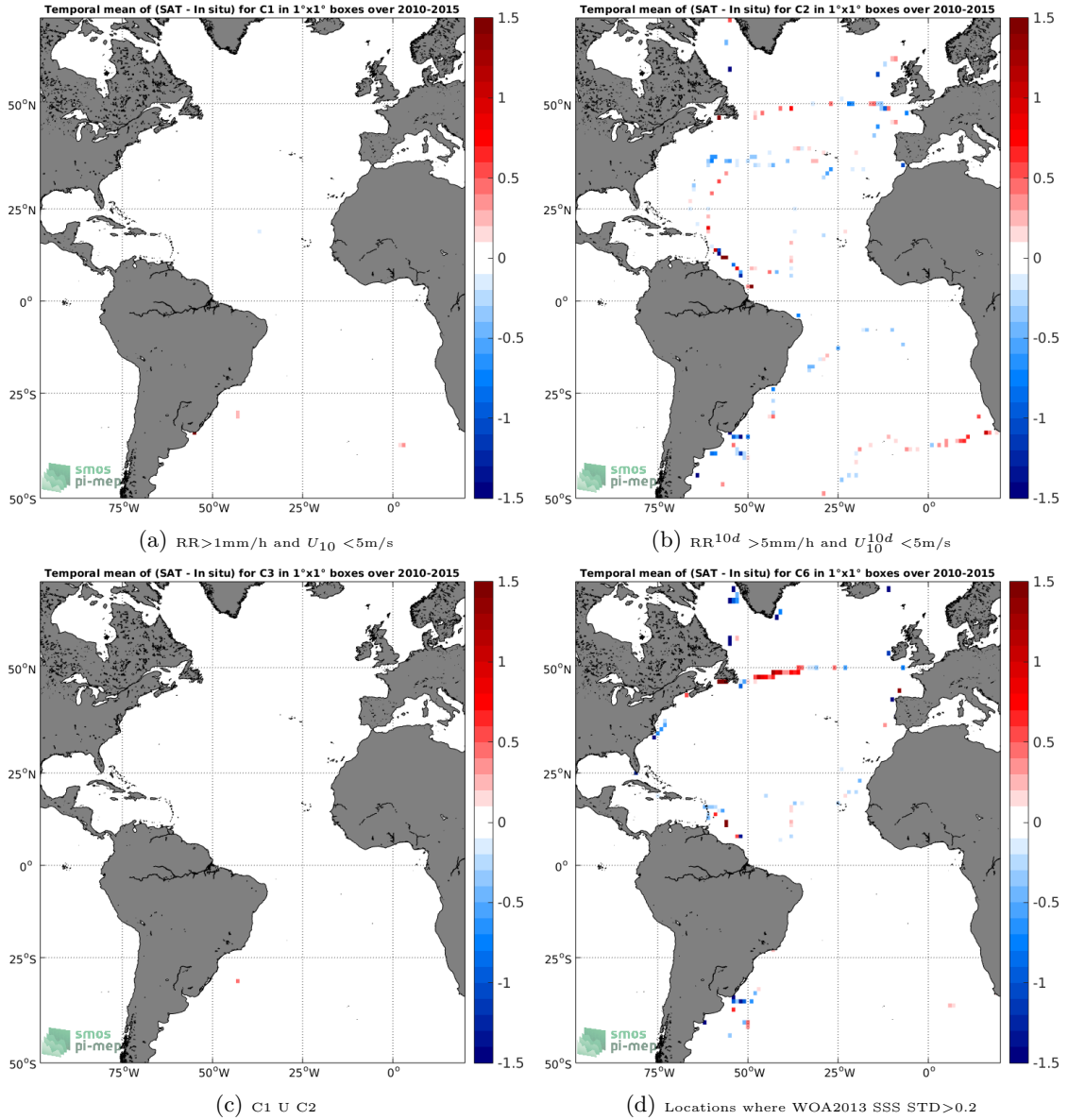
Figure 12: Temporal mean gridded over spatial boxes of size 1^\circ \times 1^\circ of \Delta SSS (SMOS-L3-CATDS-IFREMER-CECOS-V2-MONTHLY-0.25DEG - TSG-GOSUD-Sailing-ship) for 4 different sub-datasets corresponding to:RR >1\text{mm/h} and U_{10} < 5\text{m/s} (a), RR 10d > 5\text{mm/h} and U_{10}^{10d} < 5\text{m/s} (b), C1 U C2 (c),Locations where WOA2013 SSS STD >0.2 (d).
