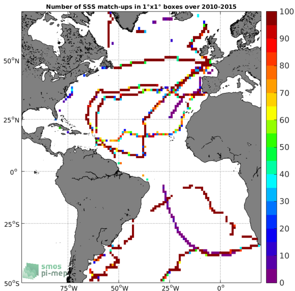
Figure 4: Number of SSS match-ups between TSG-GOSUD-Sailing-ship SSS and the SMOS-L3-CATDS-IFREMER-CECOS-V2-MONTHLY-0.25DEG SSS product for the Atlantic Ocean Pi-MEP region over 1°x1° boxes and for the full satellite product period.
