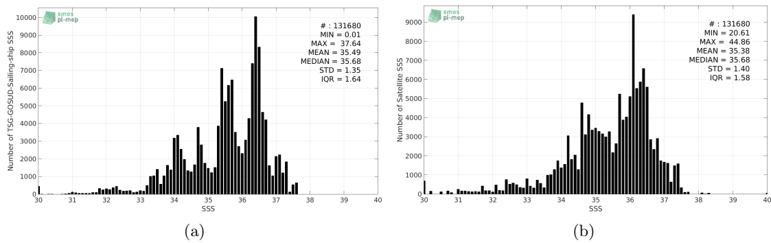
Figure 2: Histograms of SSS from TSG-GOSUD-Sailing-ship (a) and SMOS-L3-CATDS-IFREMER-CECOS-V2-MONTHLY-0.25DEG (b) considering all match-up pairs per bins of 0.1 over the Atlantic Ocean Pi-MEP region and for the full satellite product period.
