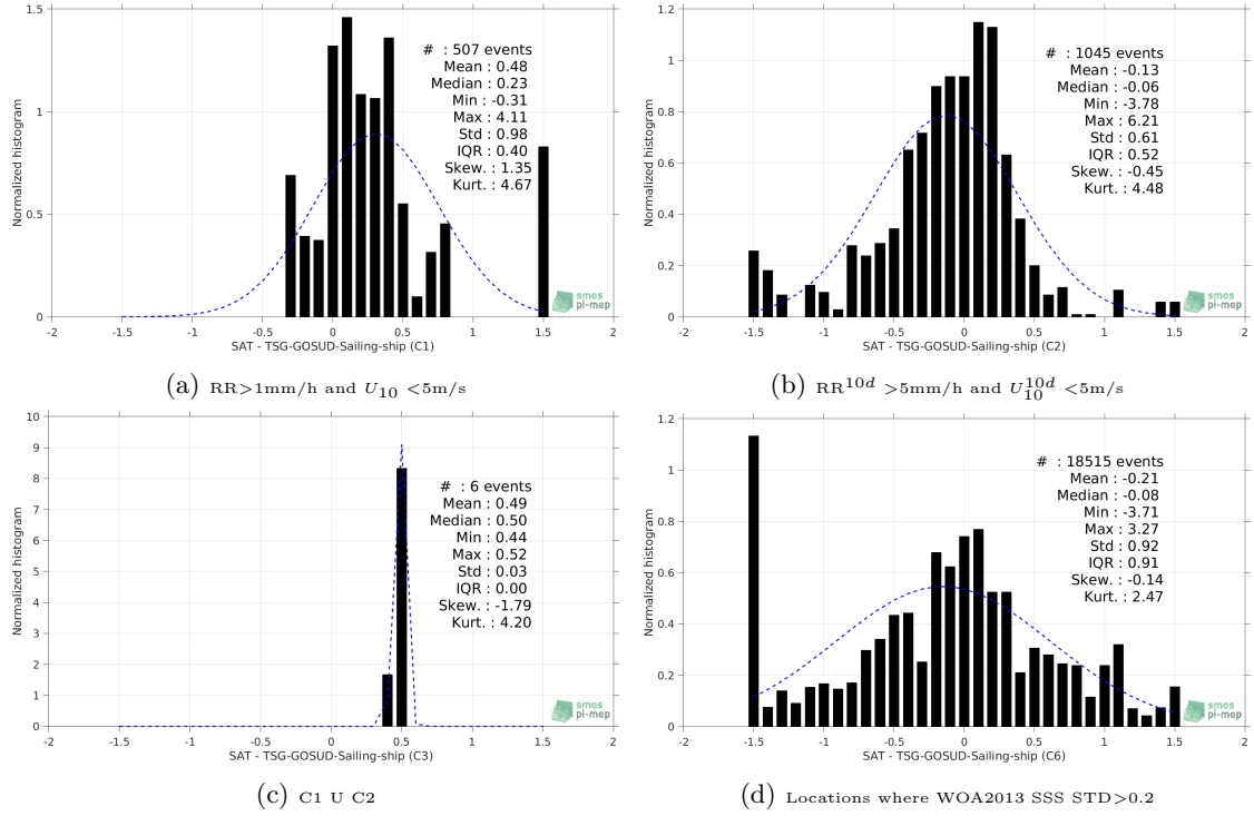
Figure 13: Normalized histogram of \Delta SSS (SMOS-L3-CATDS-IFREMER-CECOS-V2-MONTHLY-0.25DEG - TSG-GOSUD-Sailing-ship) for 6 different subdatasets corresponding to: RR > 1mm/h and U_{10} < 5 m/s (a), RR^{10d} > 5 mm/h and U_{10}^{10d} < 5 m/s (b), C1 U C2 (c), Locations where WOA2013 SSS STD > 0.2 (d).
