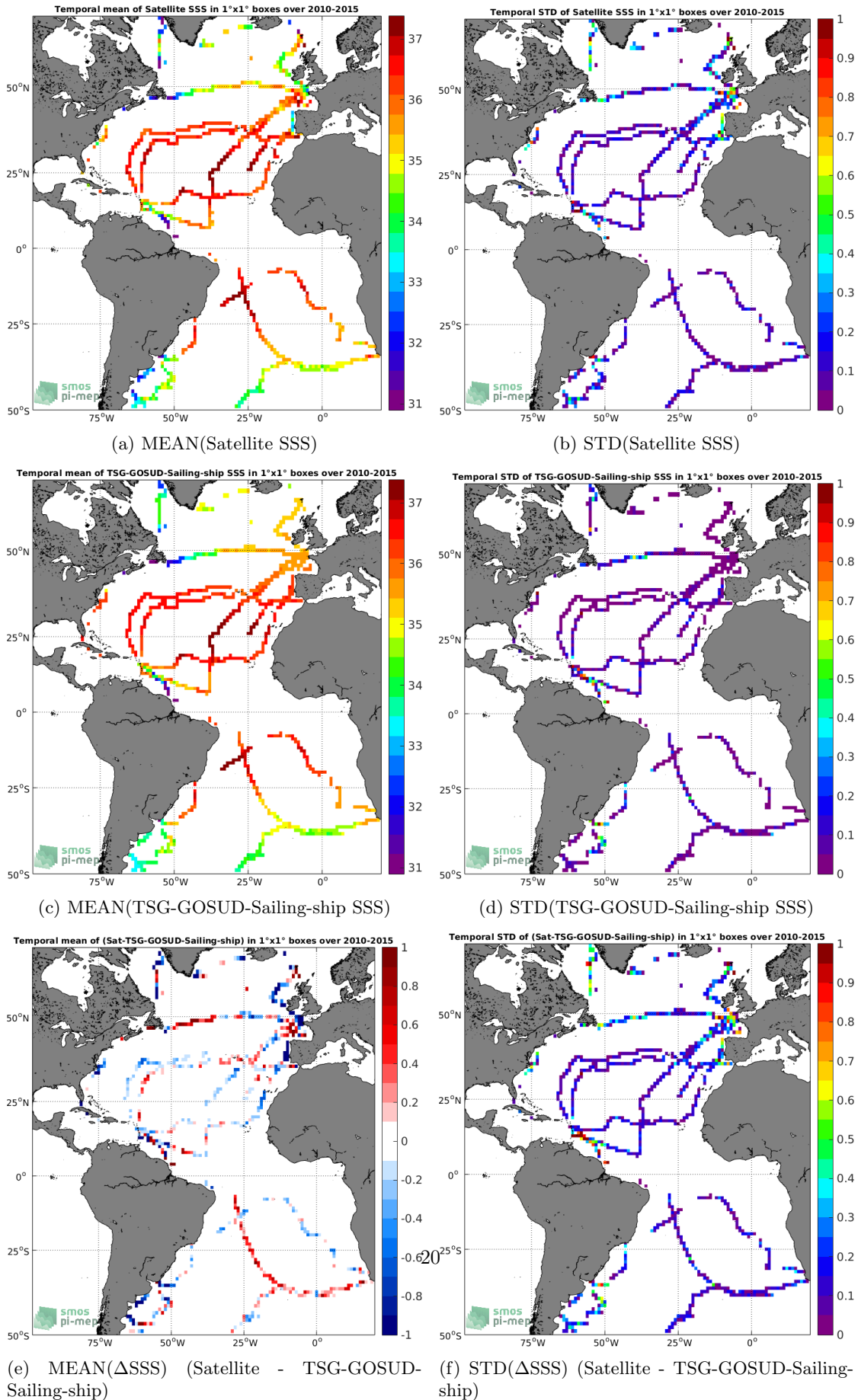
Figure 6: Temporal mean (left) and STD (right) of SSS from SMOS-L3-CATDS-IFREMER-CECOS-V2-MONTHLY-0.25DEG (top), TSG-GOSUD-Sailing-ship (middle), and of \Delta SSS (Satellite - TSG-GOSUD-Sailing-ship). Only match-up pairs are used to generate these maps.
