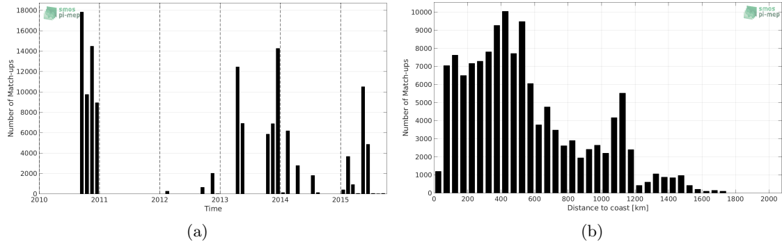
Figure 1: Number of match-ups between TSG-GOSUD-Sailing-ship and SMOS-L3-CATDS-IFREMER-CECOS-V2-MONTHLY-0.25DEG SSS as a function of time (a) and as function of the distance to coast (b) over the Atlantic Ocean Pi-MEP region and for the full satellite product period.
