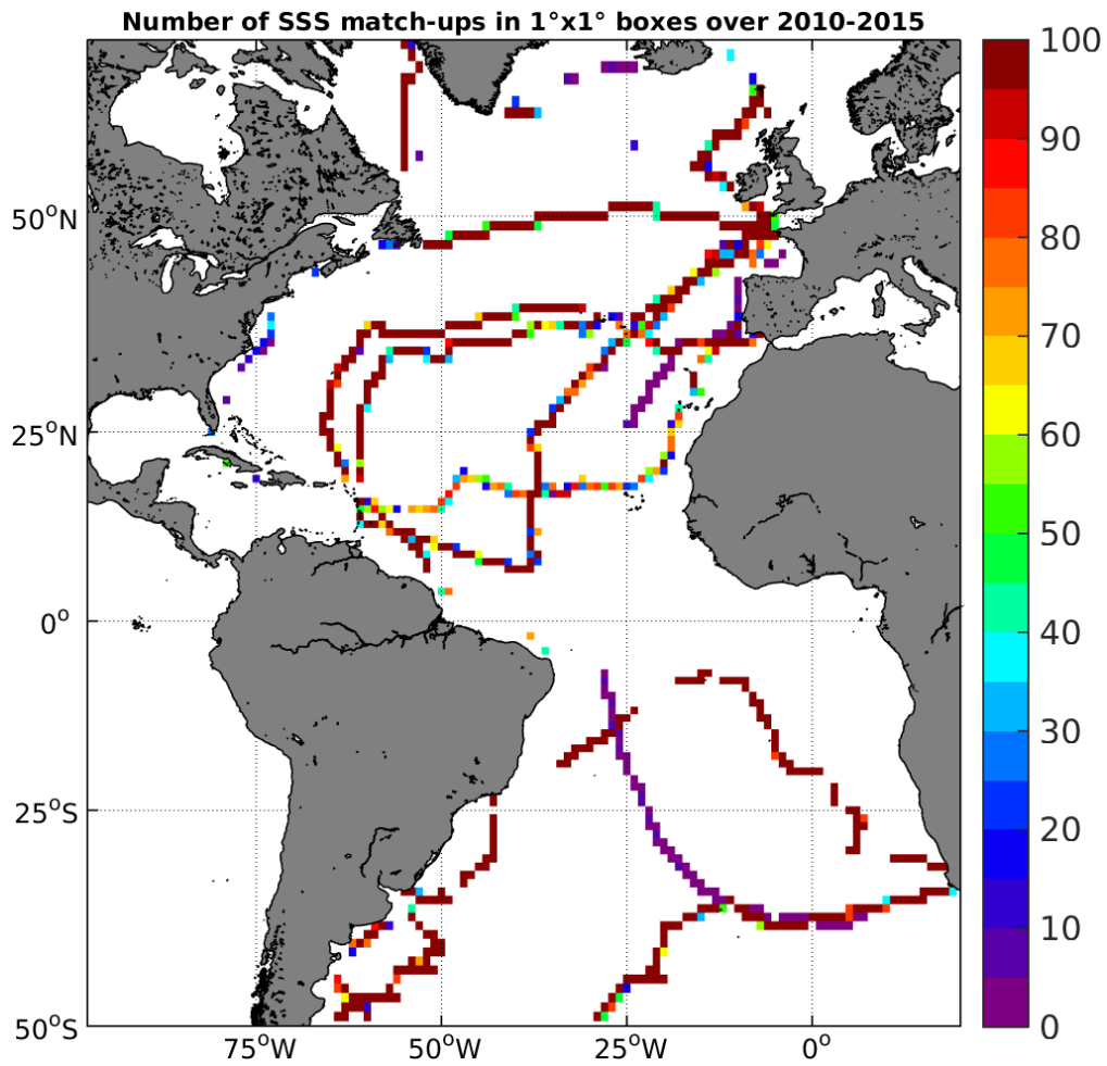
Figure 4: Number of SSS match-ups between TSG-GOSUD-Sailing-ship SSS and the SMOS-L3-CATDS-IFREMER-CECOS-V2-MONTHLY-0.25DEG SSS product for the Atlantic Ocean Pi-MEP region over 1°x1° boxes and for the full satellite product period.
