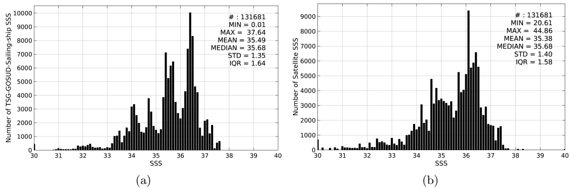
Figure 2: Histograms of SSS from TSG-GOSUD-Sailing-ship (a) and SMOS-L3-CATDS-IFREMER-CECOS-V2-MONTHLY-0.25DEG (b) considering all match-up pairs per bins of 0.1 over the Atlantic Ocean Pi-MEP region and for the full satellite product period.
