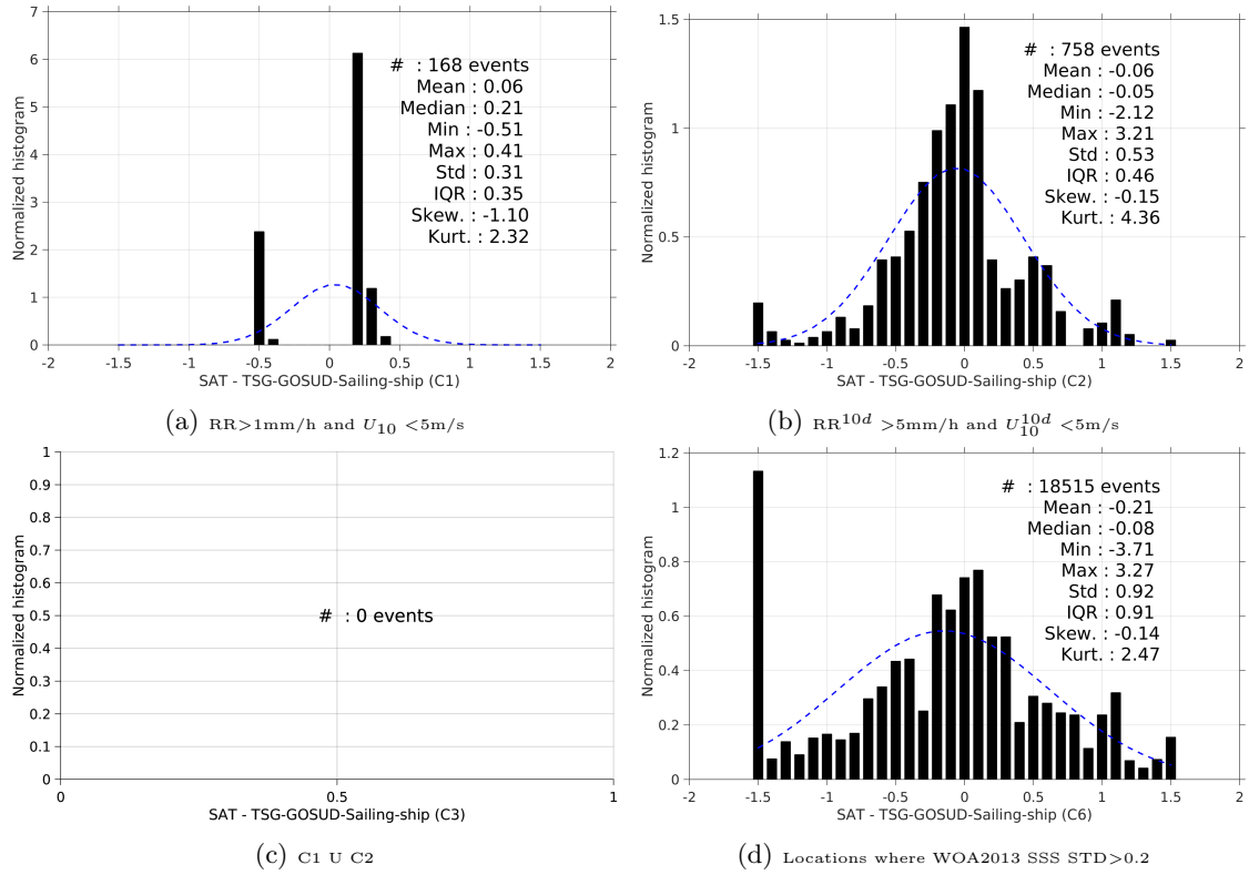
Figure 13: Normalized histogram of \Delta\text{SSS} (SMOS-L3-CATDS-IFREMER-CECOS-V2-MONTHLY-0.25DEG - TSG-GOSUD-Sailing-ship) for 6 different subdatasets corresponding to: RR > 1mm/h and U_{10} < 5\text{m/s} (a), RR^{10d} > 5\text{mm/h} and U_{10}^{10d} < 5\text{m/s} (b), C1 U C2 (c), Locations where WOA2013 SSS STD > 0.2 (d).
