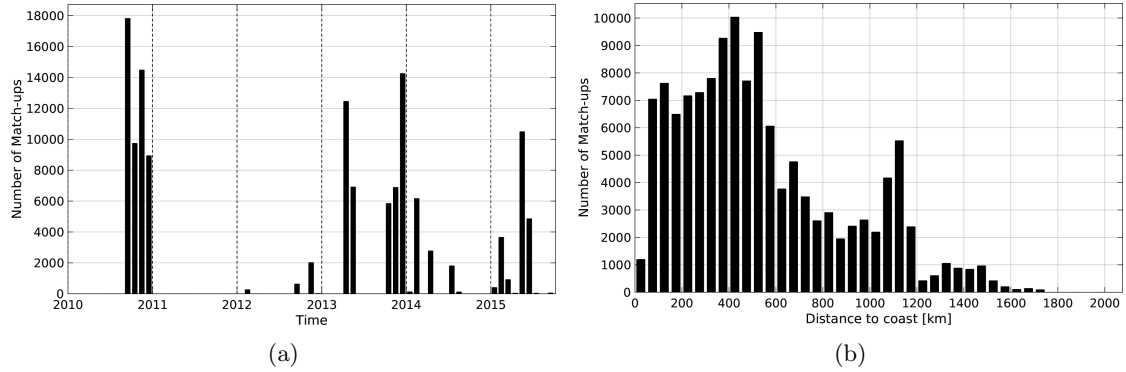
Figure 1: Number of match-ups between TSG-GOSUD-Sailing-ship and SMOS-L3-CATDS-IFREMER-CECOS-V2-MONTHLY-0.25DEG SSS as a function of time (a) and as function of the distance to coast (b) over the Atlantic Ocean Pi-MEP region and for the full satellite product period.
