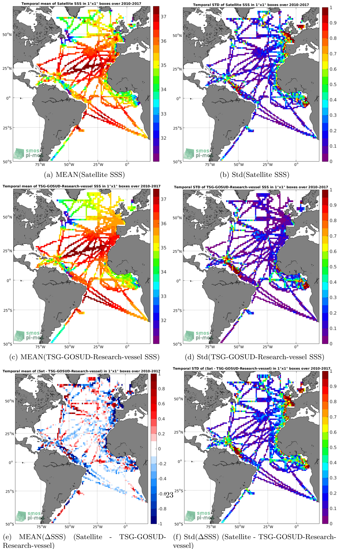
Figure 6: Temporal mean (left) and Std (right) of SSS from SMOS L3 v2 - Monthly - 0.25 Deg (CATDS-CECOS-IFREMER) (top), TSG-GOSUD-Research-vessel (middle), and of \Delta SSS (Satellite - TSG-GOSUD-Research-vessel). Only match-up pairs are used to generate these maps.
