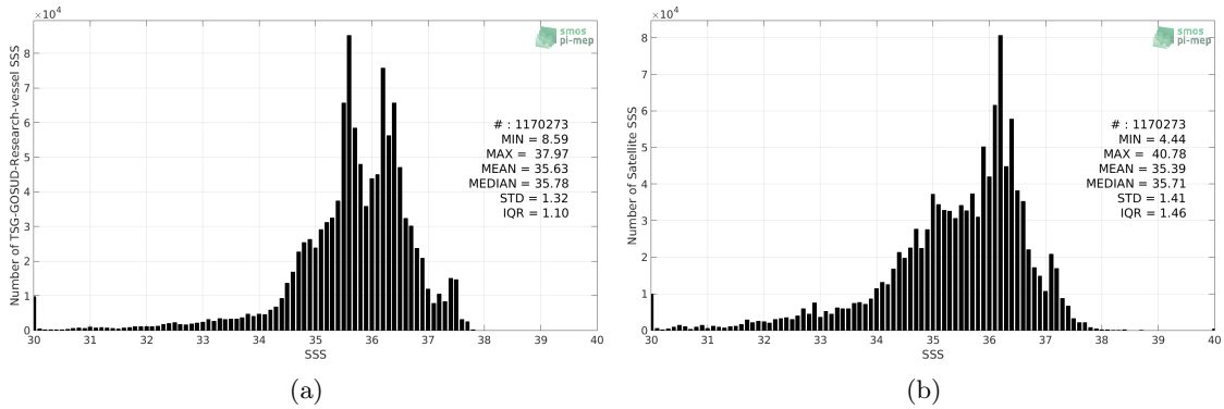
Figure 2: Histograms of SSS from TSG-GOSUD-Research-vessel (a) and SMOS L3 v2 - Monthly - 0.25 Deg (CATDS-CECOS-IFREMER) (b) considering all match-up pairs per bins of 0.1 over the Atlantic Ocean Pi-MEP region and for the full satellite product period.
