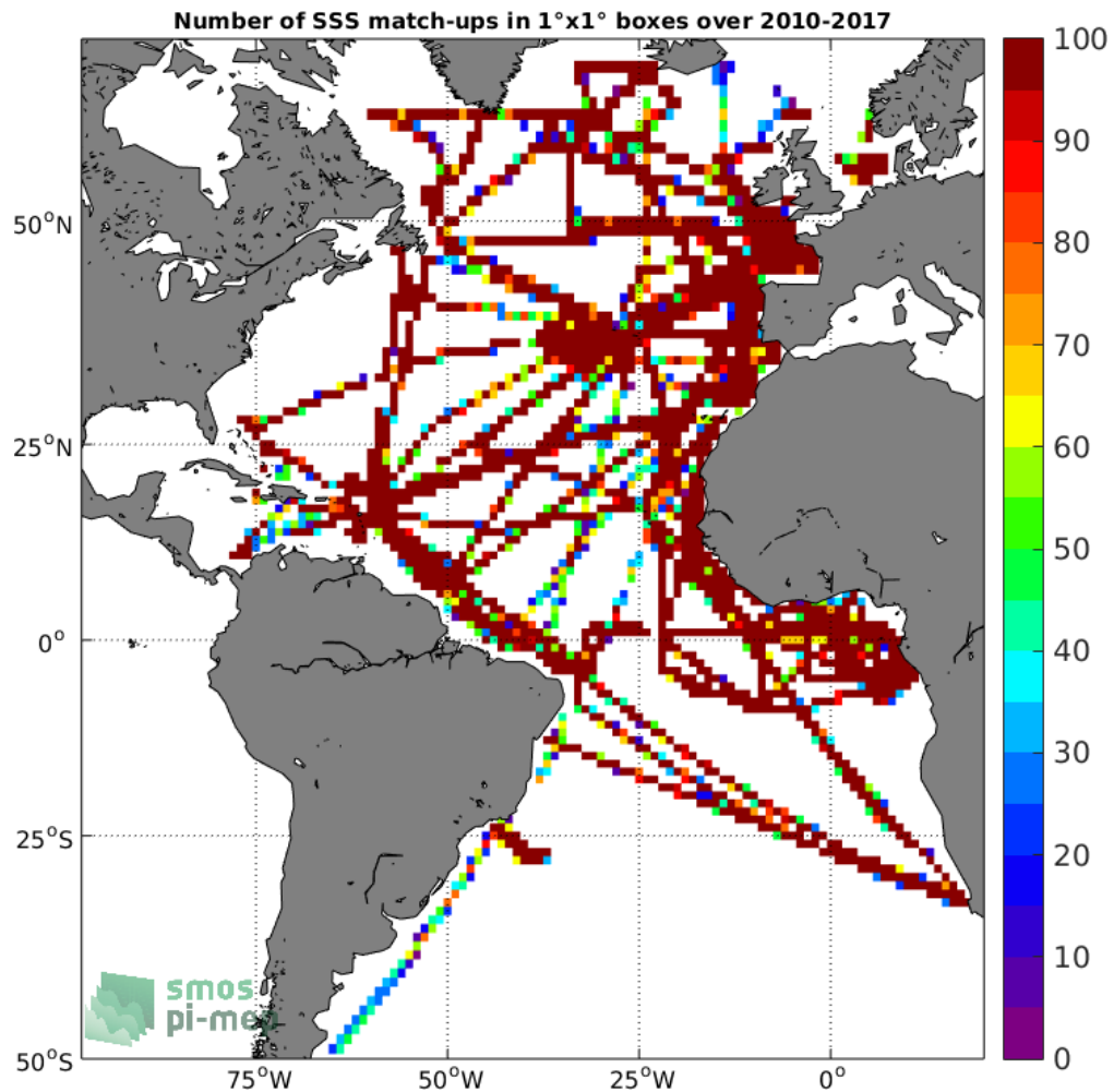
Figure 4: Number of SSS match-ups between TSG-GOSUD-Research-vessel SSS and the SMOS L3 v2 - Monthly - 0.25 Deg (CATDS-CECOS-IFREMER) SSS product for the Atlantic Ocean Pi-MEP region over 1°x1° boxes and for the full satellite product period.
