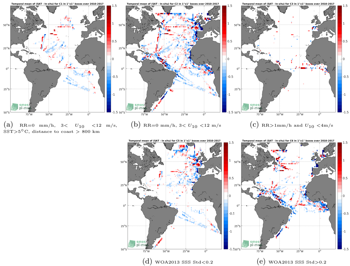
Figure 12: Temporal mean gridded over spatial boxes of size 1^\circ \times 1^\circ of \Delta SSS (SMOS-L3-CATDS-IFREMER-CECOS-V2-MONTHLY-0.25DEG - TSG-GOSUD-Research-vessel) for 5 different subdatasets corresponding to:RR=0 mm/h, 3 < U_{10} < 12 m/s, SST >5^\circ C, distance to coast > 800 km (a), RR=0 mm/h, 3 < U_{10} < 12 m/s (b), RR >1 mm/h and U_{10} < 4 m/s (c), WOA2013 SSS Std <0.2 (d), WOA2013 SSS Std >0.2 (e).
