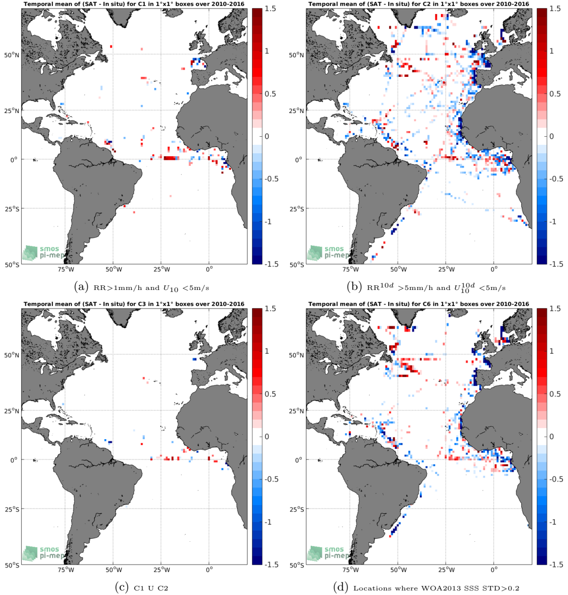
Figure 12: Temporal mean gridded over spatial boxes of size 1^\circ \times 1^\circ of \Delta SSS (SMOS-L3-CATDS-IFREMER-CECOS-V2-MONTHLY-0.25DEG - TSG-GOSUD-Research-vessel) for 4 different subdatasets corresponding to:RR>1mm/h and U_{10} < 5\text{m/s} (a), RR^{10d} > 5\text{mm/h} and U_{10}^{10d} < 5\text{m/s} (b), C1 U C2 (c),Locations where WOA2013 SSS STD>0.2 (d).
