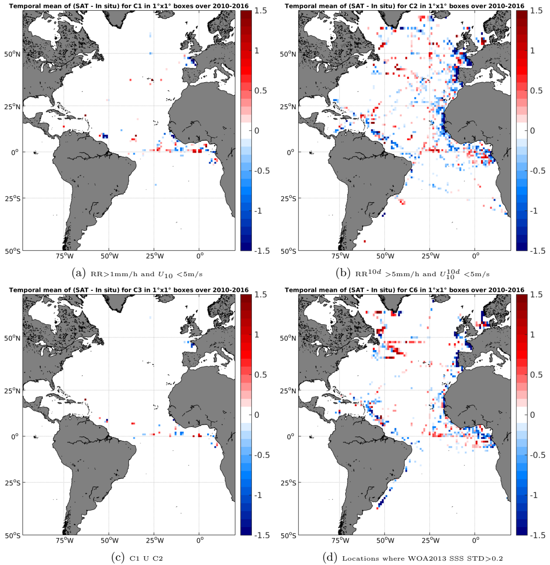
Figure 12: Temporal mean gridded over spatial boxes of size 1^\circ \times 1^\circ of \Delta\text{SSS} (SMOS-L3-CATDS-IFREMER-CECOS-V2-MONTHLY-0.25DEG - TSG-GOSUD-Research-vessel) for 4 different subdatasets corresponding to: RR > 1\text{mm/h} and U_{10} < 5\text{m/s} (a), RR^{10d} > 5\text{mm/h} and U_{10}^{10d} < 5\text{m/s} (b), C1 U C2 (c), Locations where WOA2013 SSS STD > 0.2 (d).
