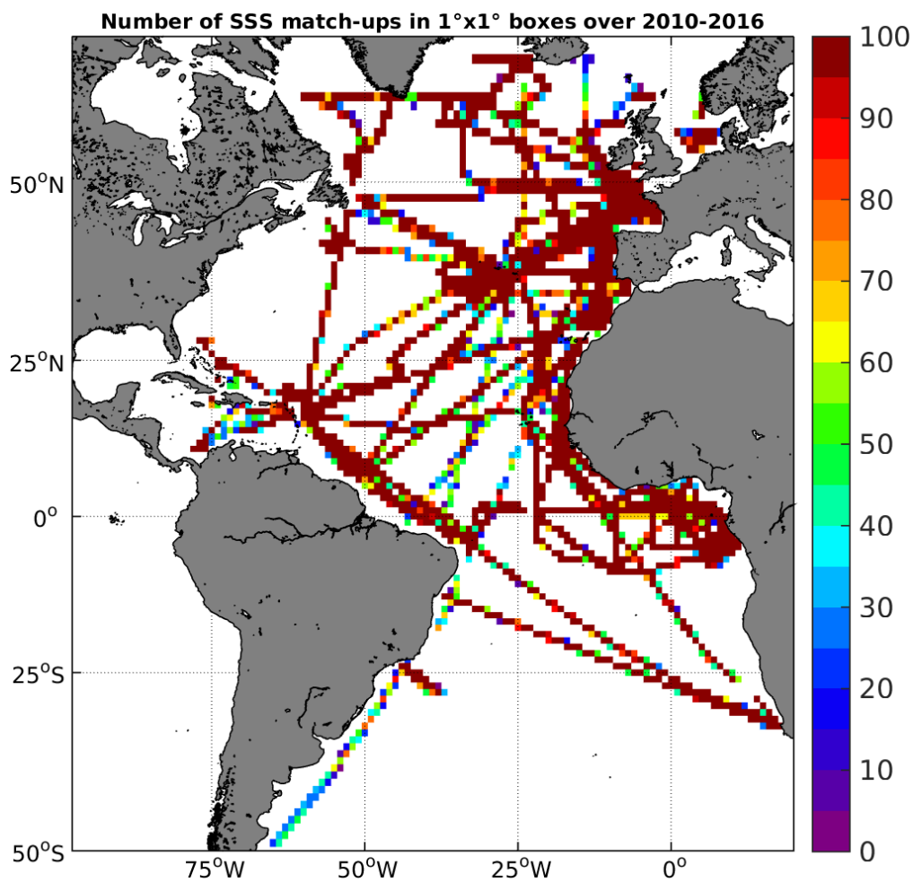
Figure 4: Number of SSS match-ups between TSG-GOSUD-Research-vessel SSS and the SMOS-L3-CATDS-IFREMER-CECOS-V2-MONTHLY-0.25DEG SSS product for the Atlantic Ocean Pi-MEP region over 1°x1° boxes and for the full satellite product period.
