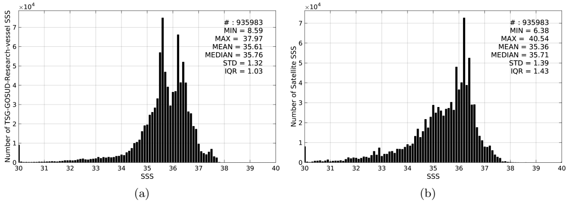
Figure 2: Histograms of SSS from TSG-GOSUD-Research-vessel (a) and SMOS-L3-CATDS-IFREMER-CECOS-V2-MONTHLY-0.25DEG (b) considering all match-up pairs per bins of 0.1 over the Atlantic Ocean Pi-MEP region and for the full satellite product period.
