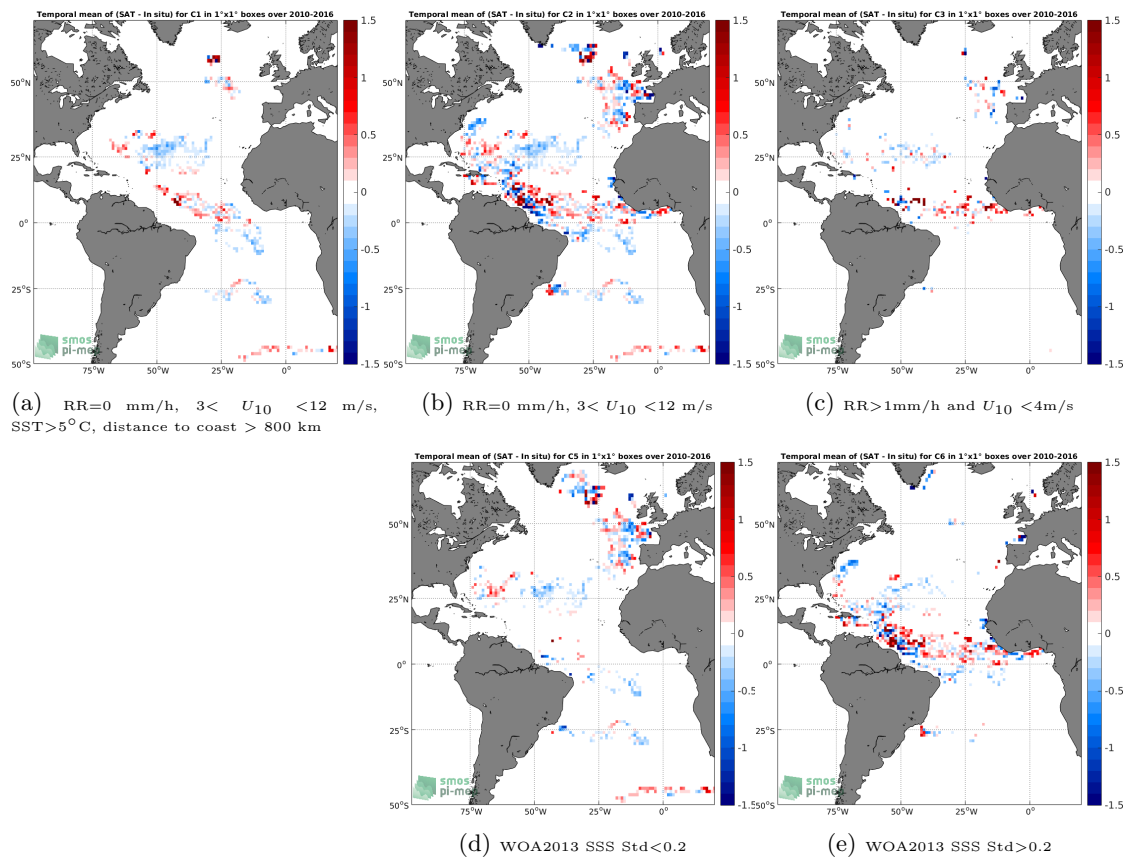
Figure 11: Temporal mean gridded over spatial boxes of size 1^\circ \times 1^\circ of \Delta SSS (SMOS SSS L3 v2 - Monthly - 0.25 Deg (CATDS-CECOS-IFREMER) - Surface drifters) for 5 different subdatasets corresponding to:RR=0 mm/h, 3 < U_{10} < 12 m/s, SST >5^\circ C, distance to coast > 800 km (a), RR=0 mm/h, 3 < U_{10} < 12 m/s (b), RR >1 mm/h and U_{10} < 4 m/s (c), WOA2013 SSS Std <0.2 (d), WOA2013 SSS Std >0.2 (e).
