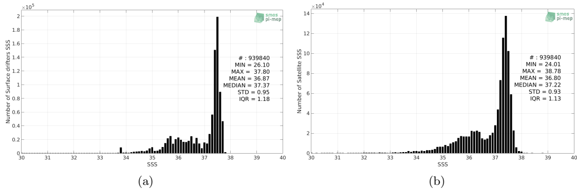
Figure 2: Histograms of SSS from Surface drifters (a) and SMOS SSS L3 v2 - Monthly - 0.25 Deg (CATDS-CECOS-IFREMER) (b) considering all match-up pairs per bins of 0.1 over the Atlantic Ocean Pi-MEP region and for the full satellite product period.
