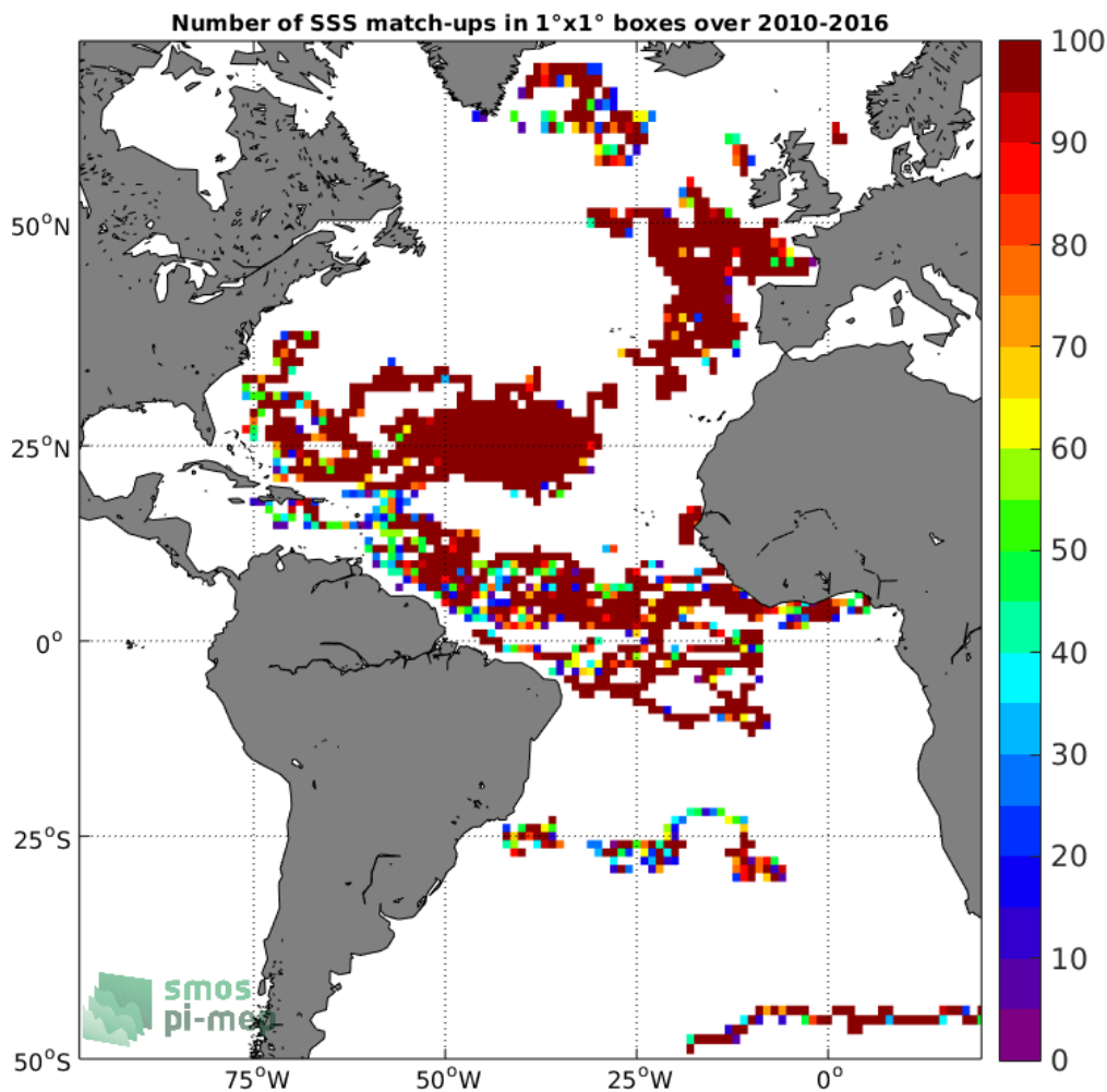
Figure 3: Number of SSS match-ups between Surface drifters SSS and the SMOS SSS L3 v2 - Monthly - 0.25 Deg (CATDS-CECOS-IFREMER) SSS product for the Atlantic Ocean Pi-MEP region over 1°x1° boxes and for the full satellite product period.
