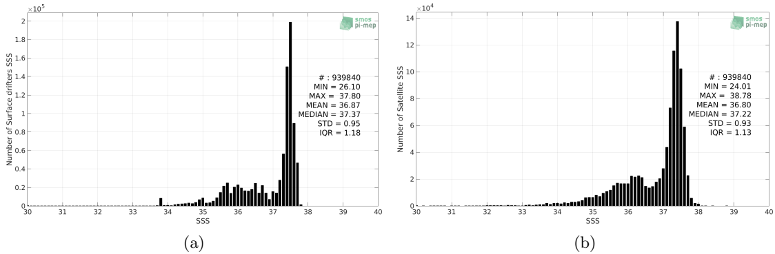
Figure 2: Histograms of SSS from Surface drifters (a) and SMOS L3 v2 - Monthly - 0.25 Deg (CATDS-CECOS-IFREMER) (b) considering all match-up pairs per bins of 0.1 over the Atlantic Ocean Pi-MEP region and for the full satellite product period.
