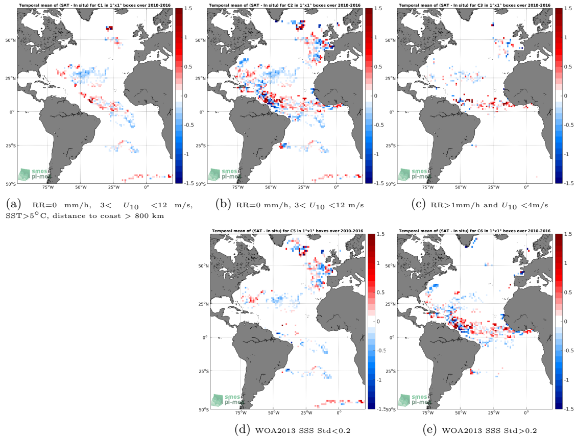
Figure 11: Temporal mean gridded over spatial boxes of size 1^\circ \times 1^\circ of \Delta SSS (SMOS L3 v2 - Monthly - 0.25 Deg (CATDS-CECOS-IFREMER) - Surface drifters) for 5 different subdatasets corresponding to:RR=0 mm/h, 3 < U_{10} < 12 m/s, SST >5^\circ C, distance to coast > 800 km (a), RR=0 mm/h, 3 < U_{10} < 12 m/s (b), RR >1 mm/h and U_{10} < 4 m/s (c), WOA2013 SSS Std <0.2 (d), WOA2013 SSS Std >0.2 (e).
