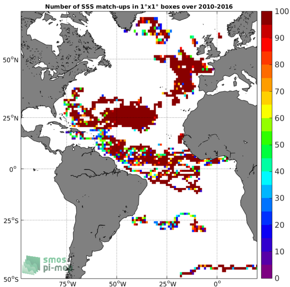
Figure 3: Number of SSS match-ups between Surface drifters SSS and the SMOS L3 v2 - Monthly - 0.25 Deg (CATDS-CECOS-IFREMER) SSS product for the Atlantic Ocean Pi-MEP region over 1°x1° boxes and for the full satellite product period.
