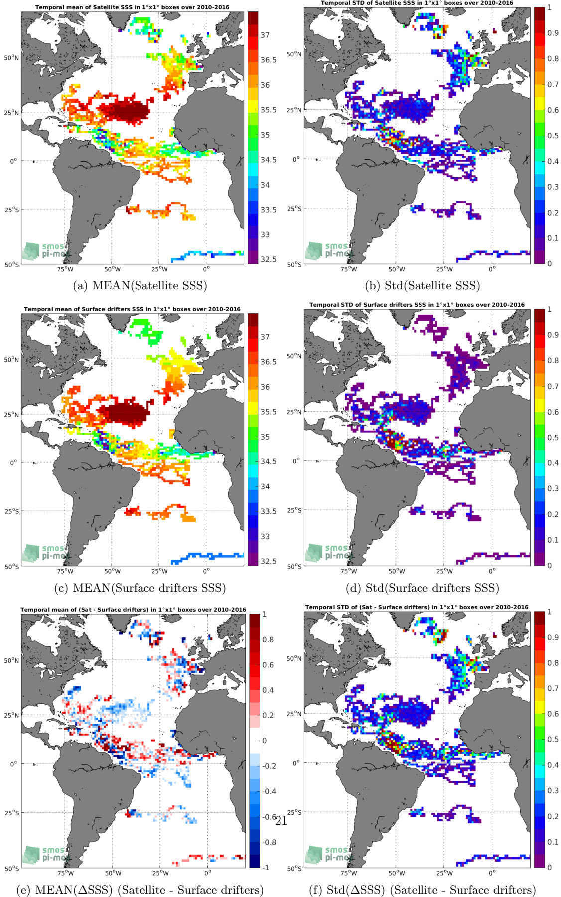
Figure 5: Temporal mean (left) and Std (right) of SSS from SMOS L3 v2 - Monthly - 0.25 Deg (CATDS-CECOS-IFREMER) (top), Surface drifters (middle), and of \Delta SSS (Satellite - Surface drifters). Only match-up pairs are used to generate these maps.
