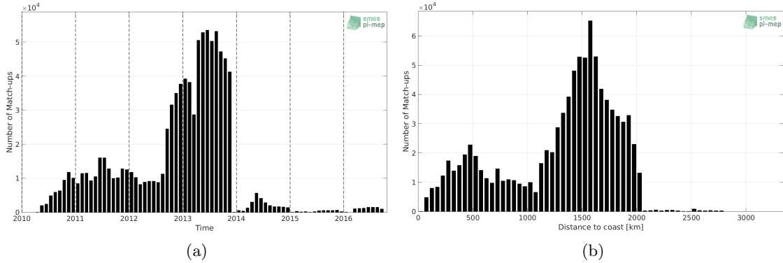
Figure 1: Number of match-ups between Surface drifters and SMOS L3 v2 - Monthly - 0.25 Deg (CATDS-CECOS-IFREMER) SSS as a function of time (a) and as function of the distance to coast (b) over the Atlantic Ocean Pi-MEP region and for the full satellite product period.
