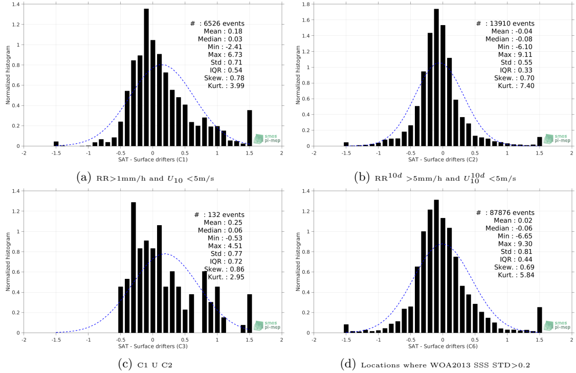
Figure 12: Normalized histogram of \Delta SSS (SMOS-L3-CATDS-IFREMER-CECOS-V2-MONTHLY-0.25DEG - Surface drifters) for 6 different subdatasets corresponding to: RR > 1mm/h and U_{10} < 5 m/s (a), RR^{10d} > 5 mm/h and U_{10}^{10d} < 5 m/s (b), C1 U C2 (c), Locations where WOA2013 SSS STD > 0.2 (d).
