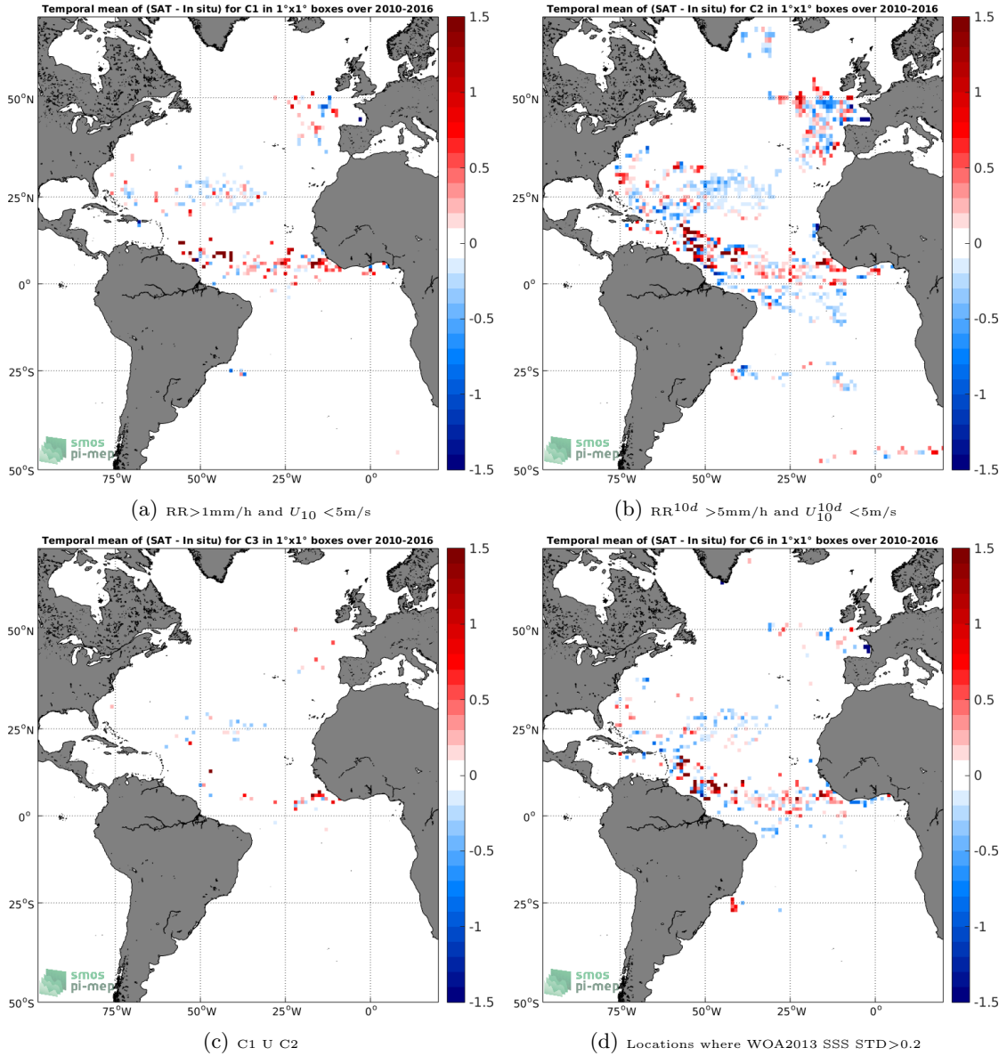
Figure 11: Temporal mean gridded over spatial boxes of size 1^\circ \times 1^\circ of \Delta SSS (SMOS-L3-CATDS-IFREMER-CECOS-V2-MONTHLY-0.25DEG - Surface drifters) for 4 different subdatasets corresponding to: RR > 1\text{mm/h} and U_{10} < 5\text{m/s} (a), RR 10d > 5\text{mm/h} and U_{10}^{10d} < 5\text{m/s} (b), C1 U C2 (c), Locations where WOA2013 SSS STD > 0.2 (d).
