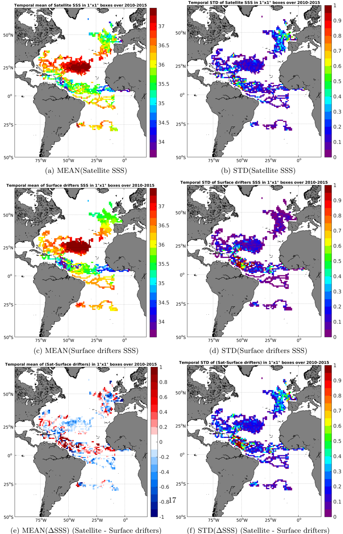
Figure 5: Temporal mean (left) and STD (right) of SSS from SMOS-L3-CATDS-IFREMER-CECOS-V2-MONTHLY-0.25DEG (top), Surface drifters (middle), and of \Delta SSS (Satellite - Surface drifters). Only match-up pairs are used to generate these maps.
