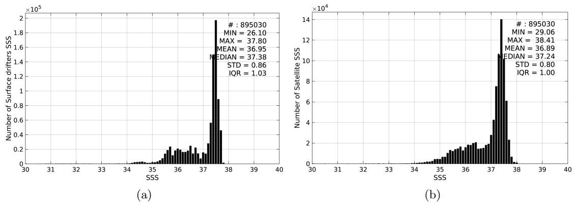
Figure 2: Histograms of SSS from Surface drifters (a) and SMOS-L3-CATDS-IFREMER-CECOS-V2-MONTHLY-0.25DEG (b) considering all match-up pairs per bins of 0.1 over the Atlantic Ocean Pi-MEP region and for the full satellite product period.
