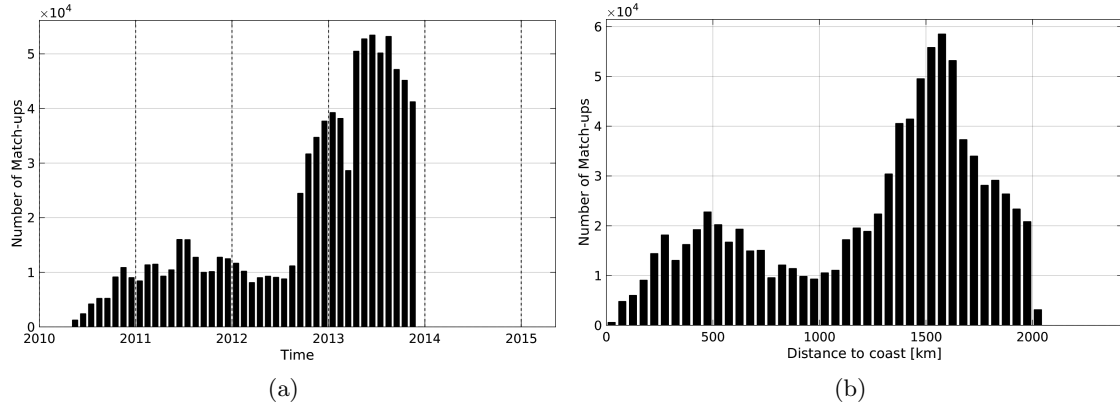
Figure 1: Number of match-ups between Surface drifters and SMOS-L3-CATDS-IFREMER-CECOS-V2-MONTHLY-0.25DEG SSS as a function of time (a) and as function of the distance to coast (b) over the Atlantic Ocean Pi-MEP region and for the full satellite product period.
