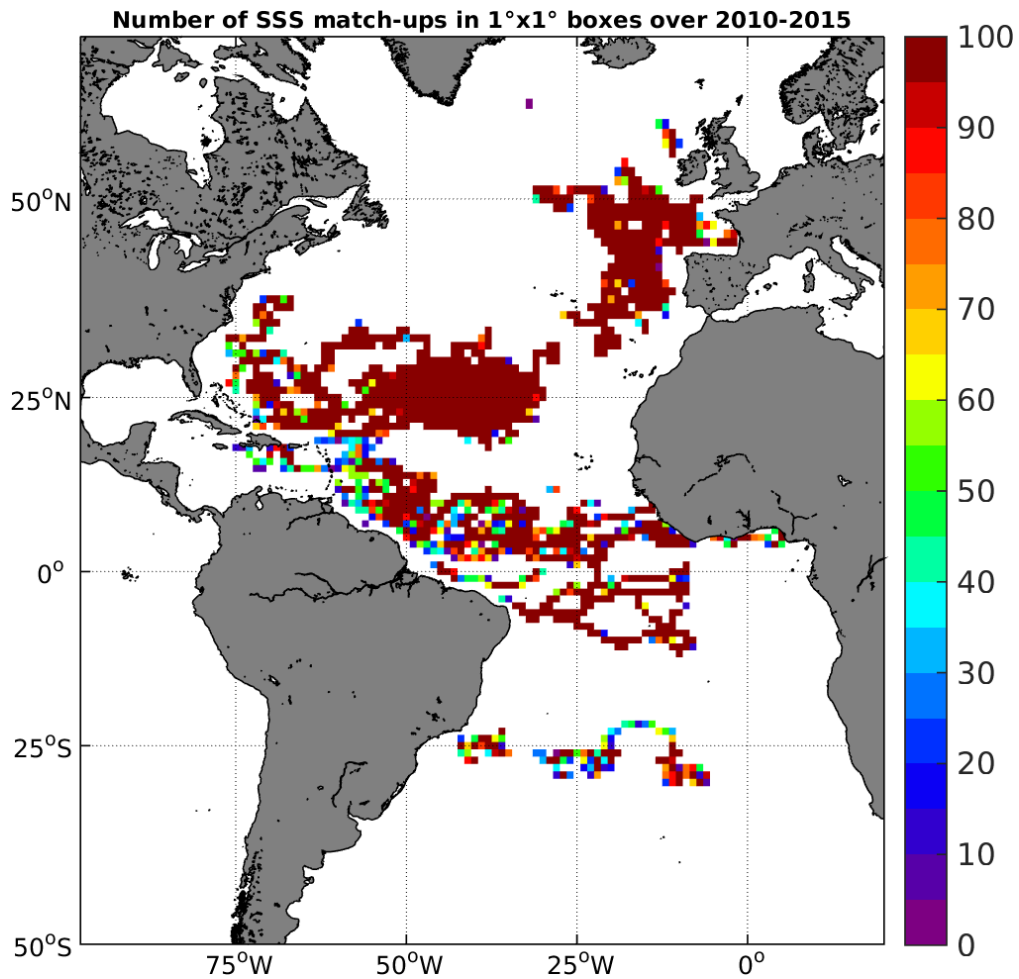
Figure 3: Number of SSS match-ups between Surface drifters SSS and the SMOS-L3-CATDS-IFREMER-CECOS-V2-MONTHLY-0.25DEG SSS product for the Atlantic Ocean Pi-MEP region over 1°x1° boxes and for the full satellite product period.
