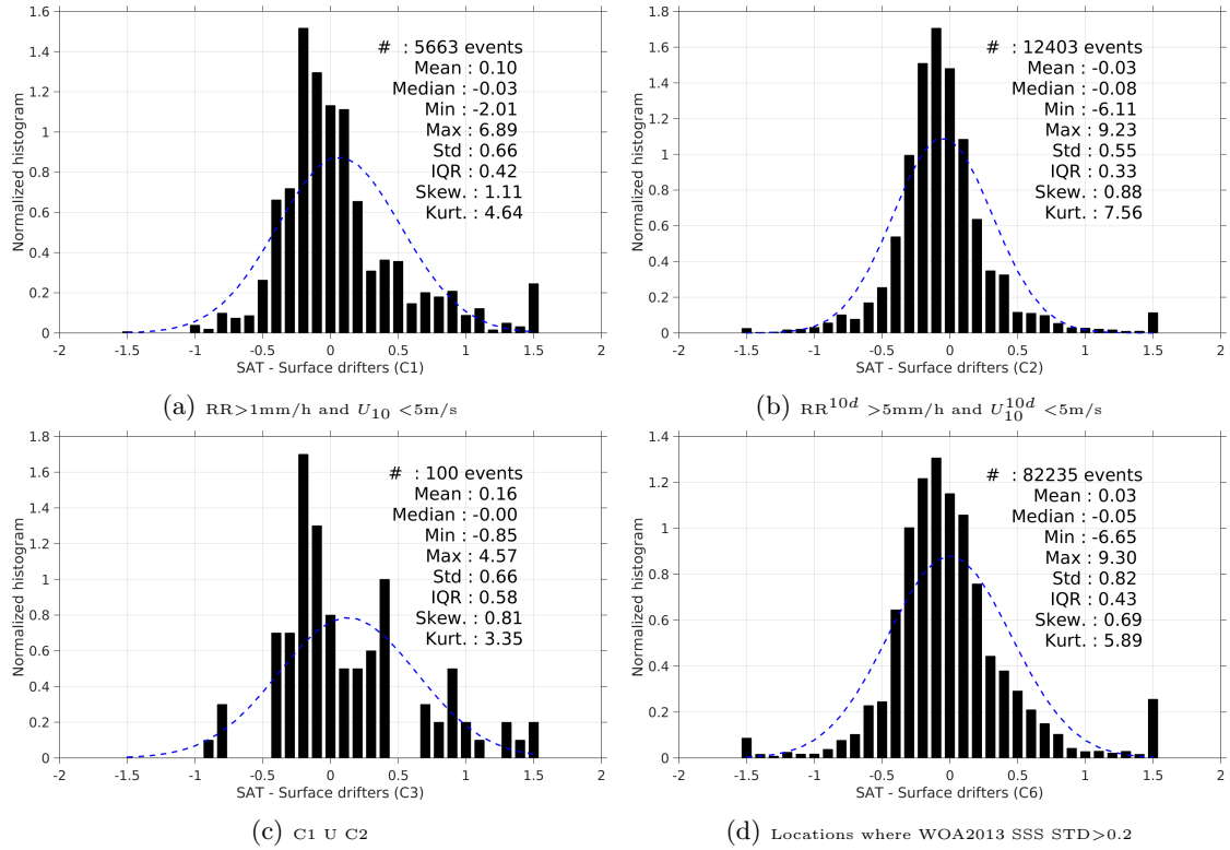
Figure 12: Normalized histogram of \Delta SSS (SMOS-L3-CATDS-IFREMER-CECOS-V2-MONTHLY-0.25DEG - Surface drifters) for 6 different subdatasets corresponding to: RR > 1\text{mm/h} and U_{10} < 5\text{m/s} (a), RR^{10d} > 5\text{mm/h} and U_{10}^{10d} < 5\text{m/s} (b), C1 U C2 (c), Locations where WOA2013 SSS STD > 0.2 (d).
