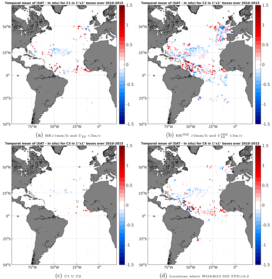
Figure 11: Temporal mean gridded over spatial boxes of size 1^\circ \times 1^\circ of \Delta SSS (SMOS-L3-CATDS-IFREMER-CECOS-V2-MONTHLY-0.25DEG - Surface drifters) for 4 different subdatasets corresponding to: RR > 1\text{mm/h} and U_{10} < 5\text{m/s} (a), RR^{10d} > 5\text{mm/h} and U_{10}^{10d} < 5\text{m/s} (b), C1 U C2 (c), Locations where WOA2013 SSS STD > 0.2 (d).
