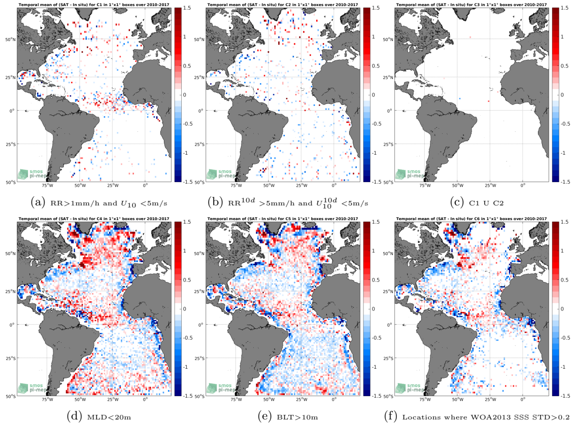
Figure 12: Temporal mean gridded over spatial boxes of size 1^\circ \times 1^\circ of \Delta\text{SSS} (SMOS-L3-CATDS-IFREMER-CECOS-V2-MONTHLY-0.25DEG - Argo) for 6 different subdatasets corresponding to: \text{RR} > 1\text{mm/h} and U_{10} < 5\text{m/s} (a), \text{RR}^{10d} > 5\text{mm/h} and U_{10}^{10d} < 5\text{m/s} (b), C1 U C2 (c), \text{MLD} < 20\text{m} (d), \text{BLT} > 10\text{m} (e), Locations where WOA2013 SSS STD > 0.2 (f).
