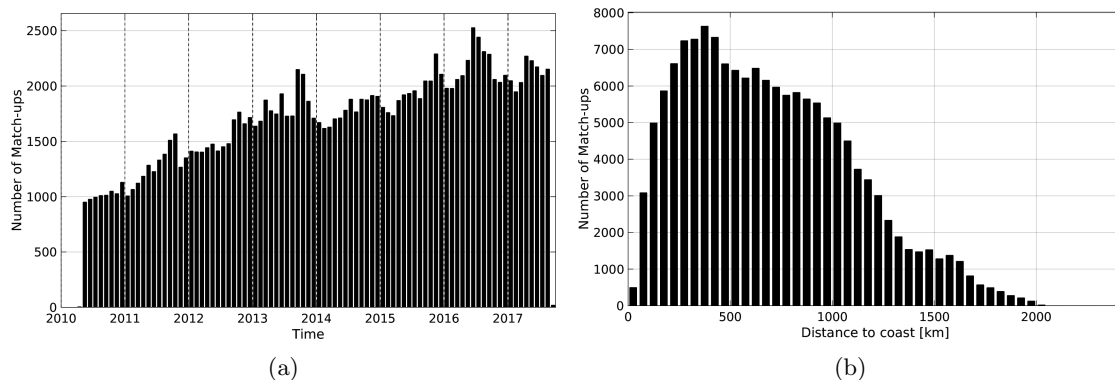
Figure 1: Number of match-ups between Argo and SMOS-L3-CATDS-IFREMER-CECOS-V2-MONTHLY-0.25DEG SSS as a function of time (a) and as function of the distance to coast (b) over the Atlantic Ocean Pi-MEP region and for the full satellite product period.
