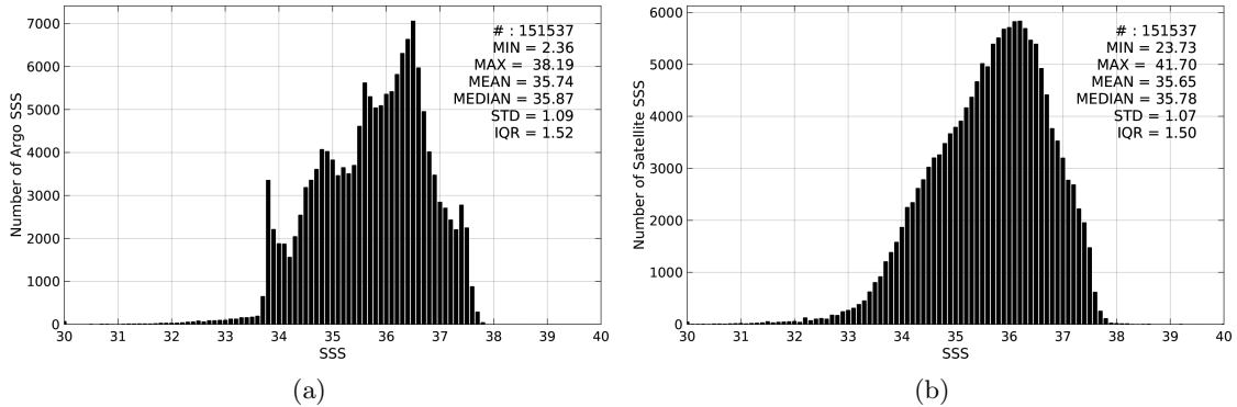
Figure 2: Histograms of SSS from Argo (a) and SMOS-L3-CATDS-IFREMER-CECOS-V2-MONTHLY-0.25DEG (b) considering all match-up pairs per bins of 0.1 over the Atlantic Ocean Pi-MEP region and for the full satellite product period.
