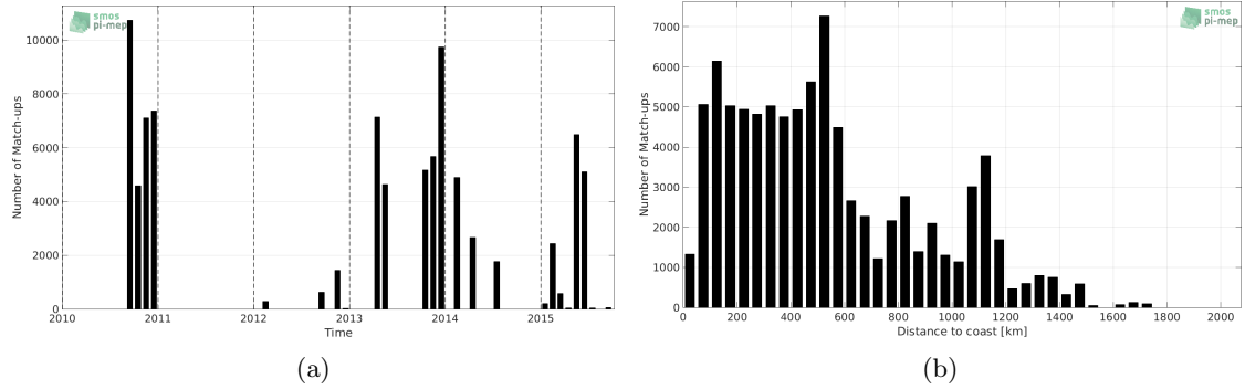
Figure 1: Number of match-ups between TSG-GOSUD-Sailing-ship and SMOS-L3-CATDS-CECOS-IFREMER-V2-1DAY-0.5DEG SSS as a function of time (a) and as function of the distance to coast (b) over the Atlantic Ocean Pi-MEP region and for the full satellite product period.
