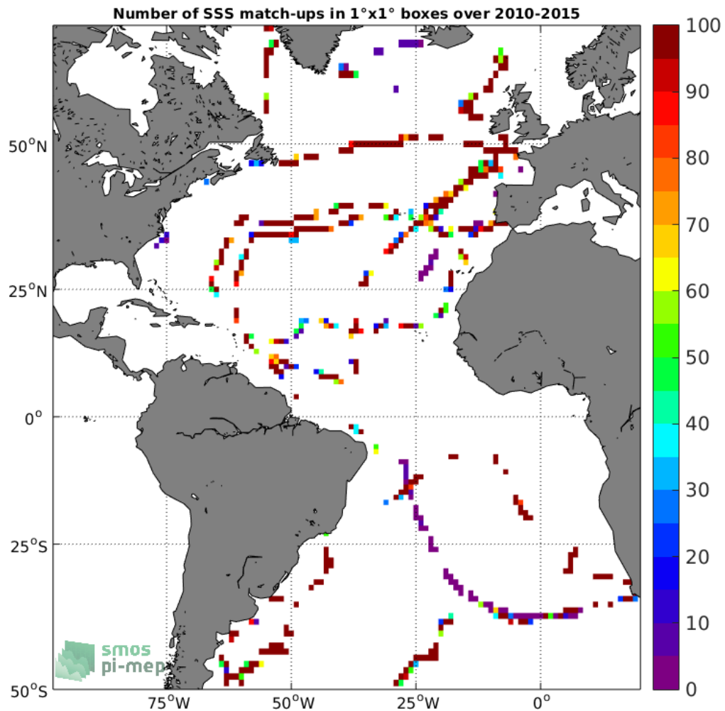
Figure 4: Number of SSS match-ups between TSG-GOSUD-Sailing-ship SSS and the SMOS-L3-CATDS-CECOS-IFREMER-V2-1DAY-0.5DEG SSS product for the Atlantic Ocean Pi-MEP region over 1°x1° boxes and for the full satellite product period.
