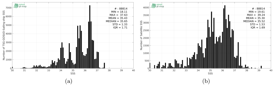
Figure 2: Histograms of SSS from TSG-GOSUD-Sailing-ship (a) and SMOS-L3-CATDS-CECOS-IFREMER-V2-1DAY-0.5DEG (b) considering all match-up pairs per bins of 0.1 over the Atlantic Ocean Pi-MEP region and for the full satellite product period.
