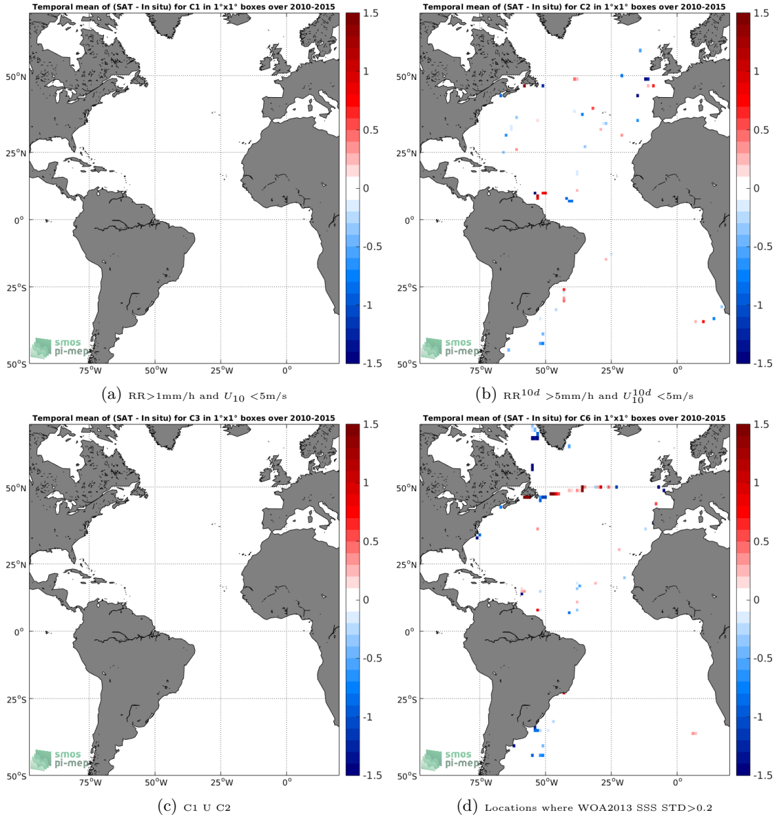
Figure 12: Temporal mean gridded over spatial boxes of size 1^\circ \times 1^\circ of \Delta SSS (SMOS-L3-CATDS-CECOS-IFREMER-V2-1DAY-0.5DEG - TSG-GOSUD-Sailing-ship) for 4 different subdatasets corresponding to: RR > 1mm/h and U_{10} < 5\text{m/s} (a), RR^{10d} > 5\text{mm/h} and U_{10}^{10d} < 5\text{m/s} (b), C1 U C2 (c), Locations where WOA2013 SSS STD > 0.2 (d).
