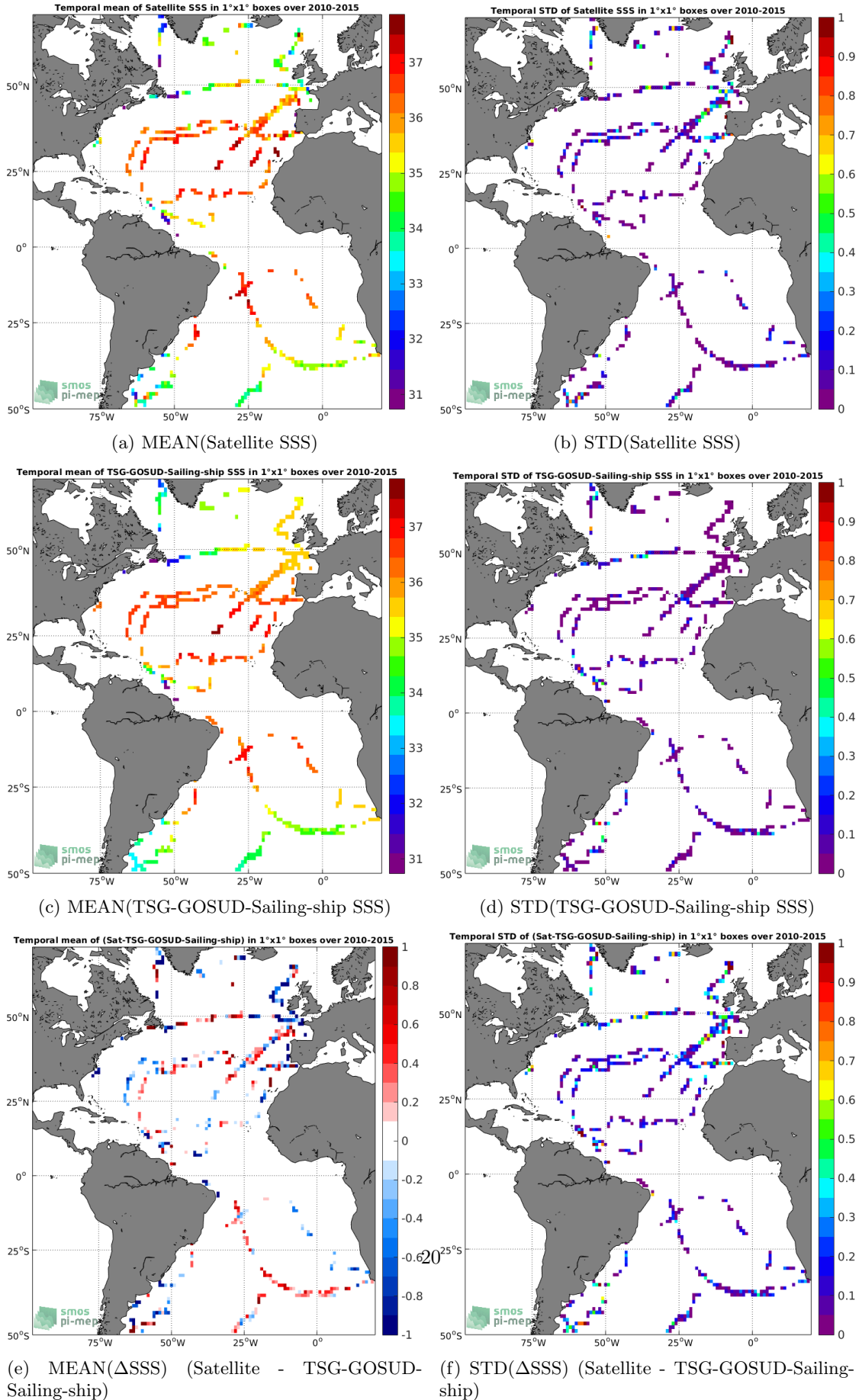
Figure 6: Temporal mean (left) and STD (right) of SSS from SMOS-L3-CATDS-CECOS-IFREMER-V2-1DAY-0.5DEG (top), TSG-GOSUD-Sailing-ship (middle), and of \Delta SSS (Satellite - TSG-GOSUD-Sailing-ship). Only match-up pairs are used to generate these maps.
