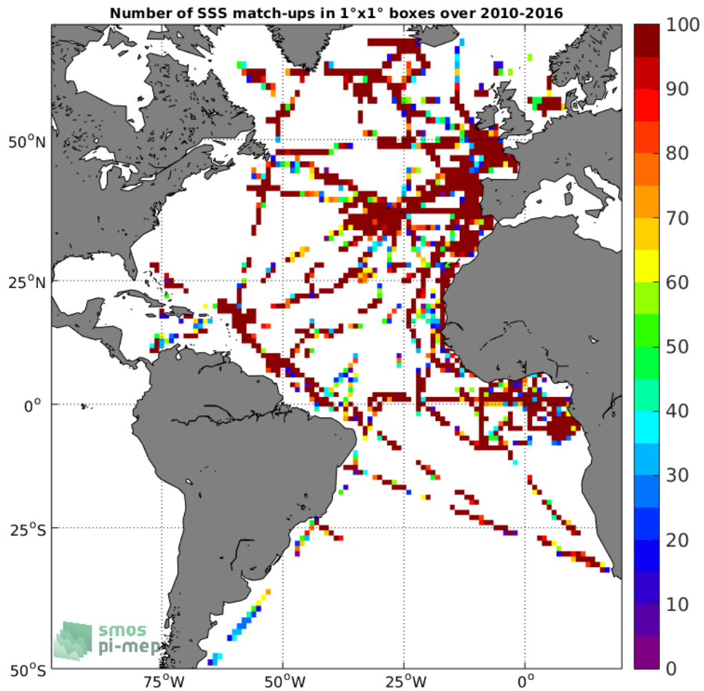
Figure 4: Number of SSS match-ups between TSG-GOSUD-Research-vessel SSS and the SMOS-L3-CATDS-CECOS-IFREMER-V2-1DAY-0.5DEG SSS product for the Atlantic Ocean Pi-MEP region over 1°x1° boxes and for the full satellite product period.
