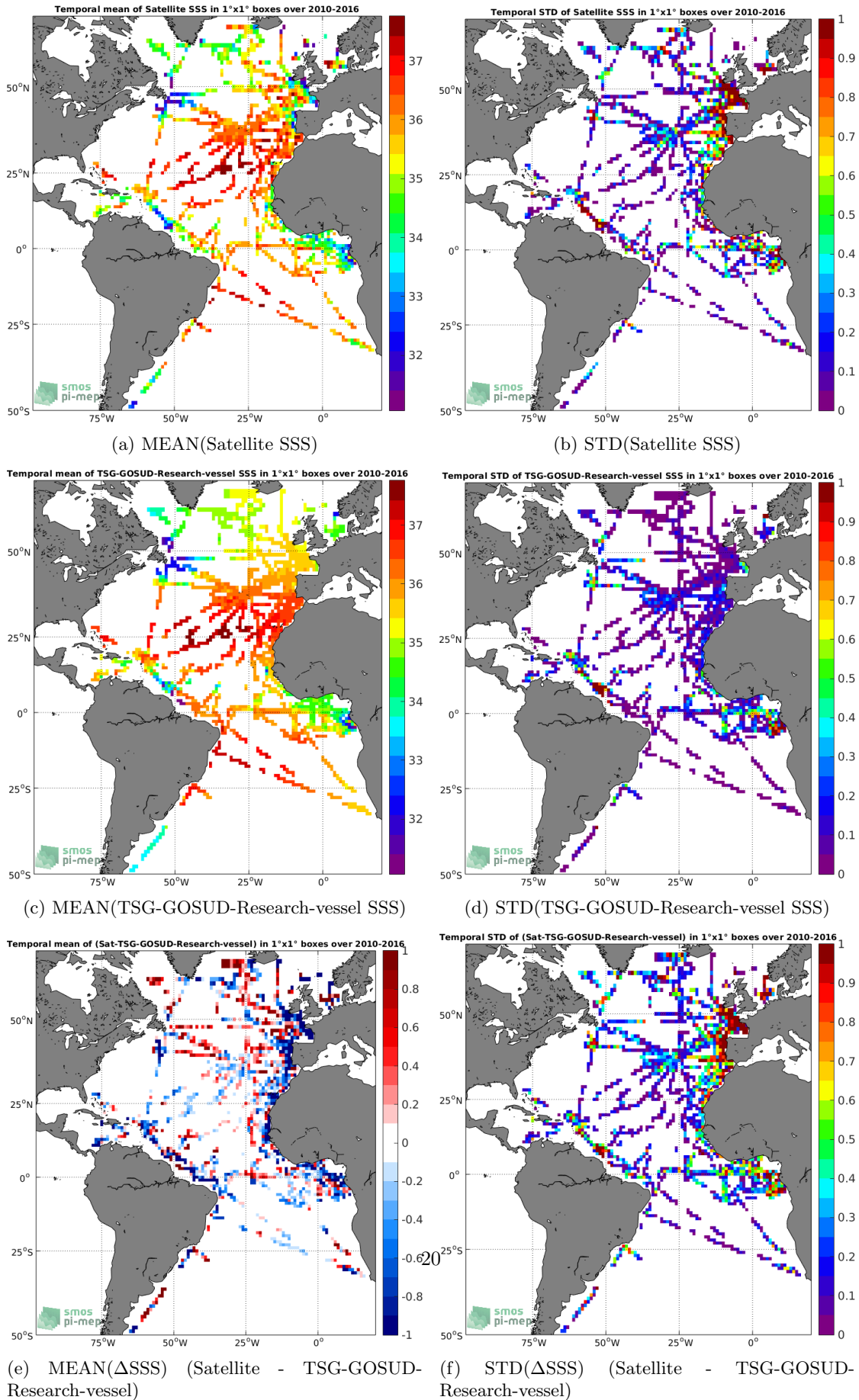
Figure 6: Temporal mean (left) and STD (right) of SSS from SMOS-L3-CATDS-CECOS-IFREMER-V2-1DAY-0.5DEG (top), TSG-GOSUD-Research-vessel (middle), and of \Delta SSS (Satellite - TSG-GOSUD-Research-vessel). Only match-up pairs are used to generate these maps.
