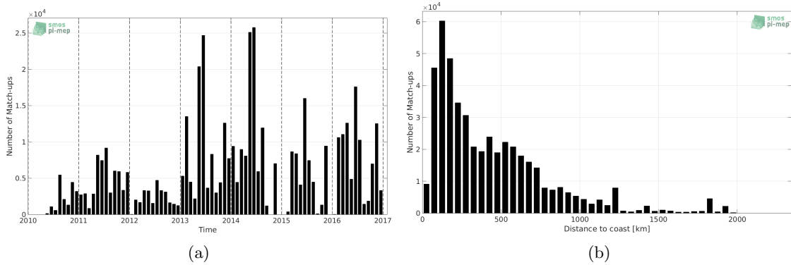
Figure 1: Number of match-ups between TSG-GOSUD-Research-vessel and SMOS-L3-CATDS-CECOS-IFREMER-V2-1DAY-0.5DEG SSS as a function of time (a) and as function of the distance to coast (b) over the Atlantic Ocean Pi-MEP region and for the full satellite product period.
