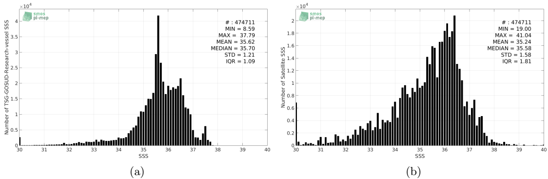
Figure 2: Histograms of SSS from TSG-GOSUD-Research-vessel (a) and SMOS-L3-CATDS-CECOS-IFREMER-V2-1DAY-0.5DEG (b) considering all match-up pairs per bins of 0.1 over the Atlantic Ocean Pi-MEP region and for the full satellite product period.
