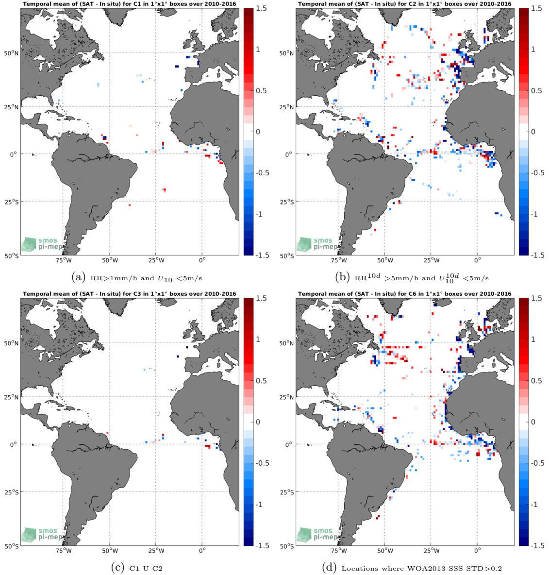
Figure 12: Temporal mean gridded over spatial boxes of size 1^\circ \times 1^\circ of \Delta SSS (SMOS-L3-CATDS-CECOS-IFREMER-V2-1DAY-0.5DEG - TSG-GOSUD-Research-vessel) for 4 different subdatasets corresponding to: RR > 1mm/h and U_{10} < 5m/s (a), RR^{10d} > 5mm/h and U_{10}^{10d} < 5m/s (b), C1 U C2 (c), Locations where WOA2013 SSS STD > 0.2 (d).
