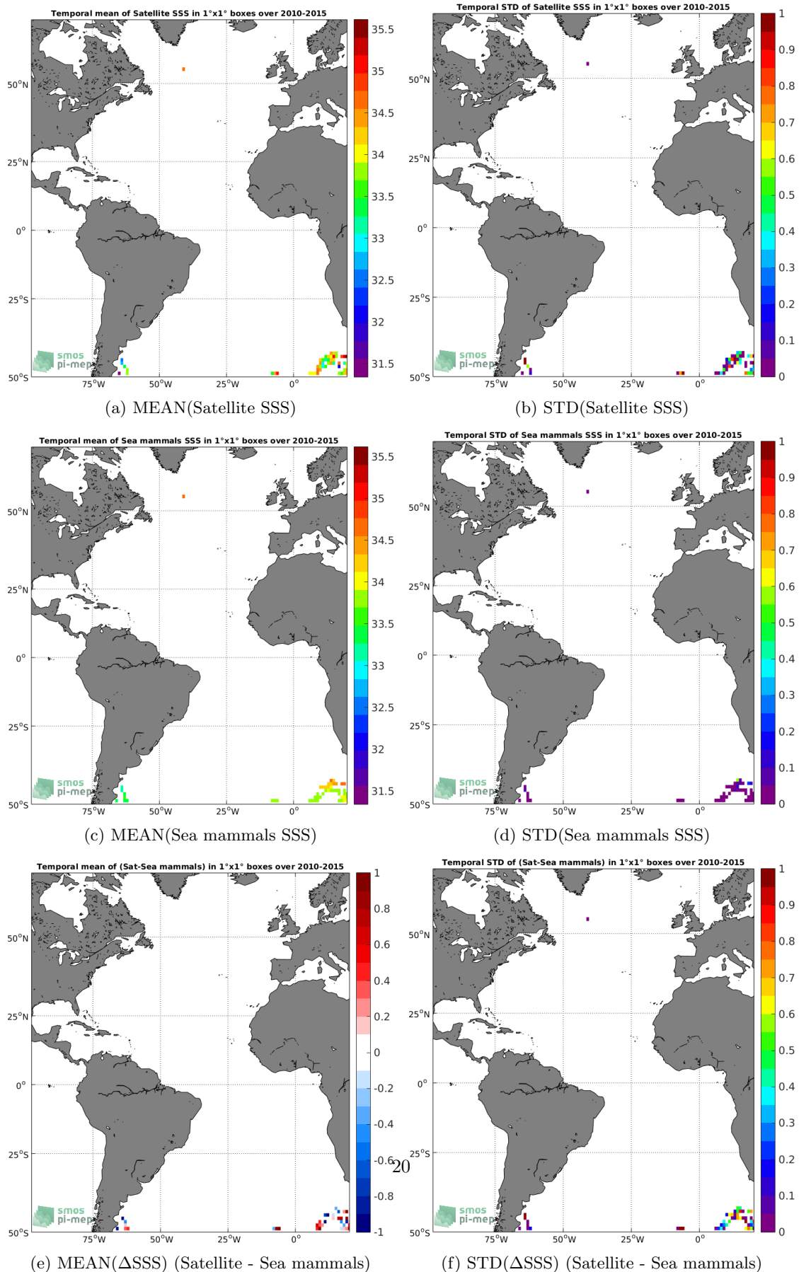
Figure 6: Temporal mean (left) and STD (right) of SSS from SMOS-L3-CATDS-CECOS-IFREMER-V2-1DAY-0.5DEG (top), Sea mammals (middle), and of \Delta SSS (Satellite - Sea mammals). Only match-up pairs are used to generate these maps.
