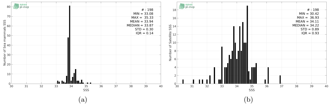
Figure 2: Histograms of SSS from Sea mammals (a) and SMOS-L3-CATDS-CECOS-IFREMER-V2-1DAY-0.5DEG (b) considering all match-up pairs per bins of 0.1 over the Atlantic Ocean Pi-MEP region and for the full satellite product period.
