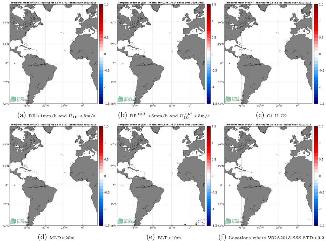
Figure 12: Temporal mean gridded over spatial boxes of size 1^\circ \times 1^\circ of \Delta\text{SSS} (SMOS-L3-CATDS-CECOS-IFREMER-V2-1DAY-0.5DEG - Sea mammals) for 6 different subdatasets corresponding to: RR > 1\text{mm/h} and U_{10} < 5\text{m/s} (a), RR^{10d} > 5\text{mm/h} and U_{10}^{10d} < 5\text{m/s} (b), C1 U C2 (c), MLD < 20\text{m} (d), BLT > 10\text{m} (e), Locations where WOA2013 SSS STD > 0.2 (f).
