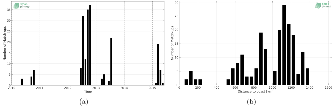
Figure 1: Number of match-ups between Sea mammals and SMOS-L3-CATDS-CECOS-IFREMER-V2-1DAY-0.5DEG SSS as a function of time (a) and as function of the distance to coast (b) over the Atlantic Ocean Pi-MEP region and for the full satellite product period.
