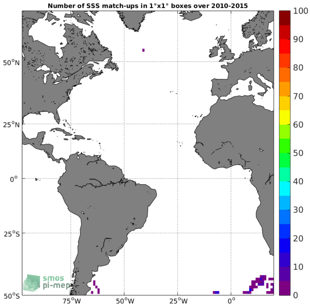
Figure 4: Number of SSS match-ups between Sea mammals SSS and the SMOS-L3-CATDS-CECOS-IFREMER-V2-1DAY-0.5DEG SSS product for the Atlantic Ocean Pi-MEP region over 1°x1° boxes and for the full satellite product period.
