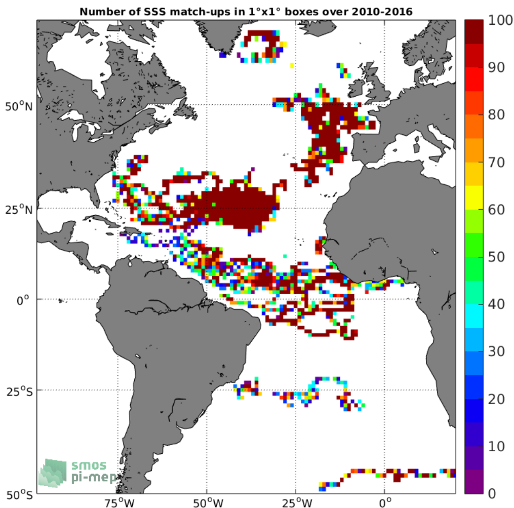
Figure 3: Number of SSS match-ups between Surface drifters SSS and the SMOS-L3-CATDS-CECOS-IFREMER-V2-1DAY-0.5DEG SSS product for the Atlantic Ocean Pi-MEP region over 1°x1° boxes and for the full satellite product period.
