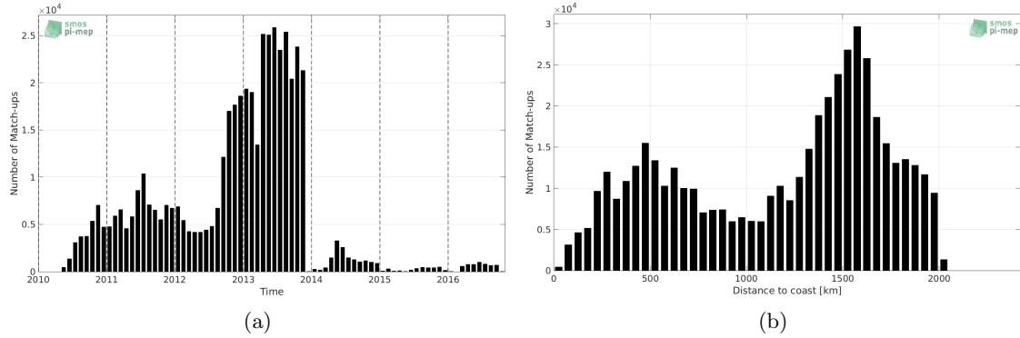
Figure 1: Number of match-ups between Surface drifters and SMOS-L3-CATDS-CECOS-IFREMER-V2-1DAY-0.5DEG SSS as a function of time (a) and as function of the distance to coast (b) over the Atlantic Ocean Pi-MEP region and for the full satellite product period.
