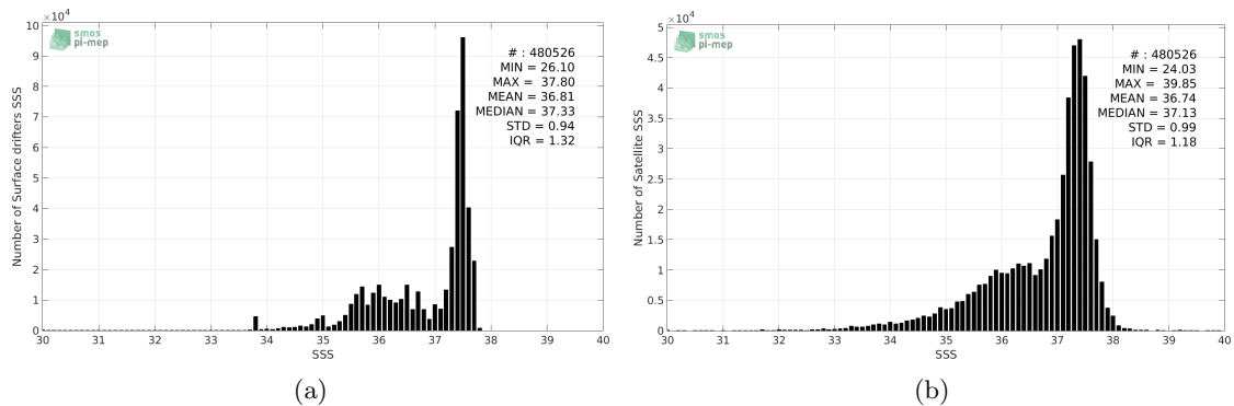
Figure 2: Histograms of SSS from Surface drifters (a) and SMOS-L3-CATDS-CECOS-IFREMER-V2-1DAY-0.5DEG (b) considering all match-up pairs per bins of 0.1 over the Atlantic Ocean Pi-MEP region and for the full satellite product period.
