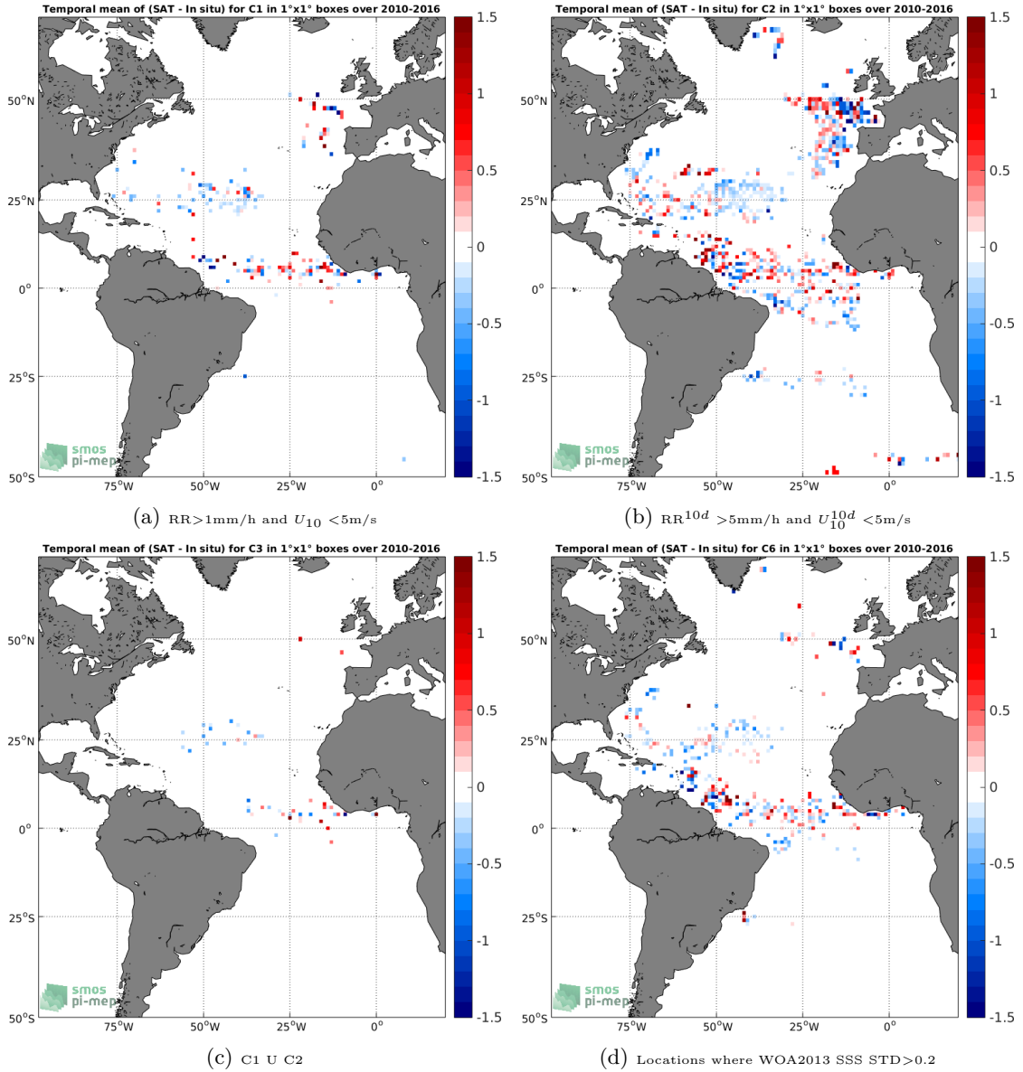
Figure 11: Temporal mean gridded over spatial boxes of size 1^\circ \times 1^\circ of \Delta SSS (SMOS-L3-CATDS-CECOS-IFREMER-V2-1DAY-0.5DEG - Surface drifters) for 4 different subdatasets corresponding to: RR > 1mm/h and U_{10} < 5\text{m/s} (a), RR^{10d} > 5\text{mm/h} and U_{10}^{10d} < 5\text{m/s} (b), C1 U C2 (c), Locations where WOA2013 SSS STD > 0.2 (d).
