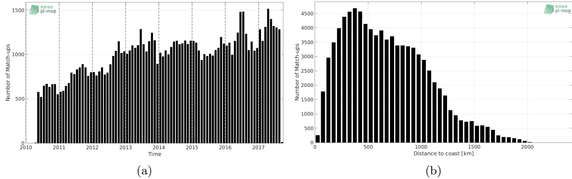
Figure 1: Number of match-ups between Argo and SMOS-L3-CATDS-CECOS-IFREMER-V2-1DAY-0.5DEG SSS as a function of time (a) and as function of the distance to coast (b) over the Atlantic Ocean Pi-MEP region and for the full satellite product period.
