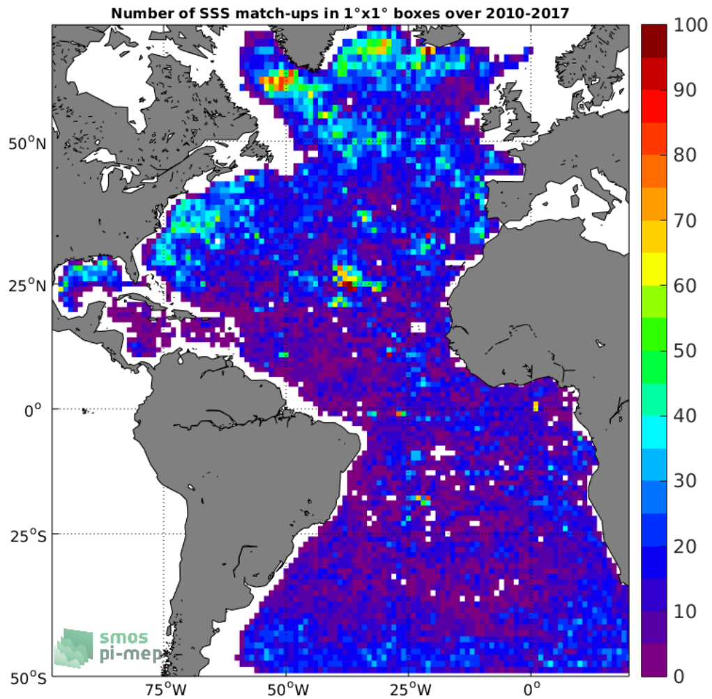
Figure 4: Number of SSS match-ups between Argo SSS and the SMOS-L3-CATDS-CECOS-IFREMER-V2-1DAY-0.5DEG SSS product for the Atlantic Ocean Pi-MEP region over 1°x1° boxes and for the full satellite product period.
