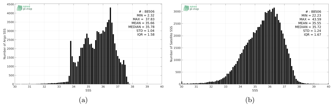
Figure 2: Histograms of SSS from Argo (a) and SMOS-L3-CATDS-CECOS-IFREMER-V2-1DAY-0.5DEG (b) considering all match-up pairs per bins of 0.1 over the Atlantic Ocean Pi-MEP region and for the full satellite product period.
