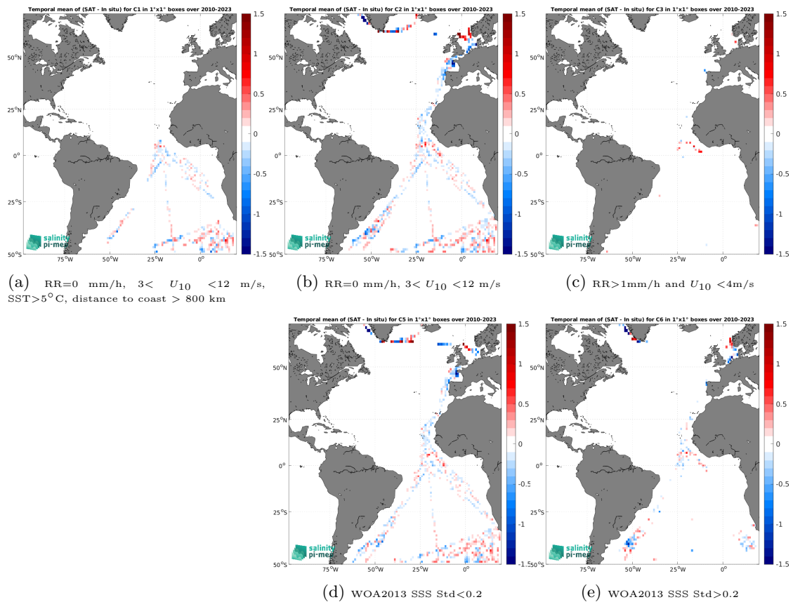
Figure 14: Temporal mean gridded over spatial boxes of size 1^\circ \times 1^\circ of \Delta SSS (SMOS SSS L3 v335 - Monthly - 25 km (CATDS-CPDC) - TSG (Polarstern)) for 5 different subdatasets corresponding to:RR=0 mm/h, 3 < U_{10} < 12 m/s, SST >5^\circ\text{C} , distance to coast > 800 km (a), RR=0 mm/h, 3 < U_{10} < 12 m/s (b), RR >1 mm/h and U_{10} < 4 m/s (c), WOA2013 SSS Std <0.2 (d), WOA2013 SSS Std >0.2 (e).
