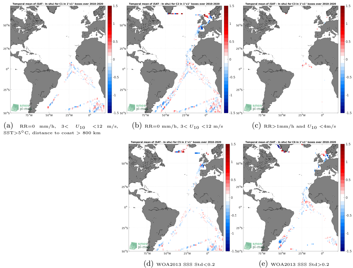
Figure 12: Temporal mean gridded over spatial boxes of size 1^\circ \times 1^\circ of \Delta SSS (SMOS SSS L3 v335 - Monthly - 25 km (CATDS-CPDC) - TSG (Polarstern)) for 5 different subdatasets corresponding to:RR=0 mm/h, 3 < U_{10} < 12 m/s, SST >5^\circ\text{C} , distance to coast > 800 km (a), RR=0 mm/h, 3 < U_{10} < 12 m/s (b), RR >1 mm/h and U_{10} < 4 m/s (c), WOA2013 SSS Std <0.2 (d), WOA2013 SSS Std >0.2 (e).
