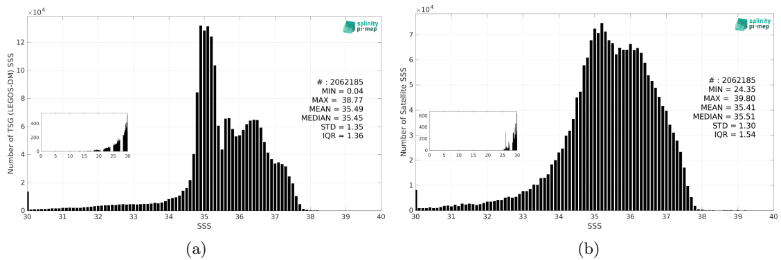
Figure 3: Histograms of SSS from TSG (LEGOS-DM) (a) and SMOS SSS L3 v335 - Monthly - 25 km (CATDS-CPDC) (b) considering all match-up pairs per bins of 0.1 over the Atlantic Ocean Pi-MEP region and for the full satellite product period.
