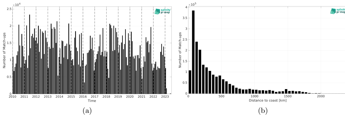
Figure 2: Number of match-ups between TSG (LEGOS-DM) and SMOS SSS L3 v335 - Monthly - 25 km (CATDS-CPDC) SSS as a function of time (a) and as function of the distance to coast (b) over the Atlantic Ocean Pi-MEP region and for the full satellite product period.
