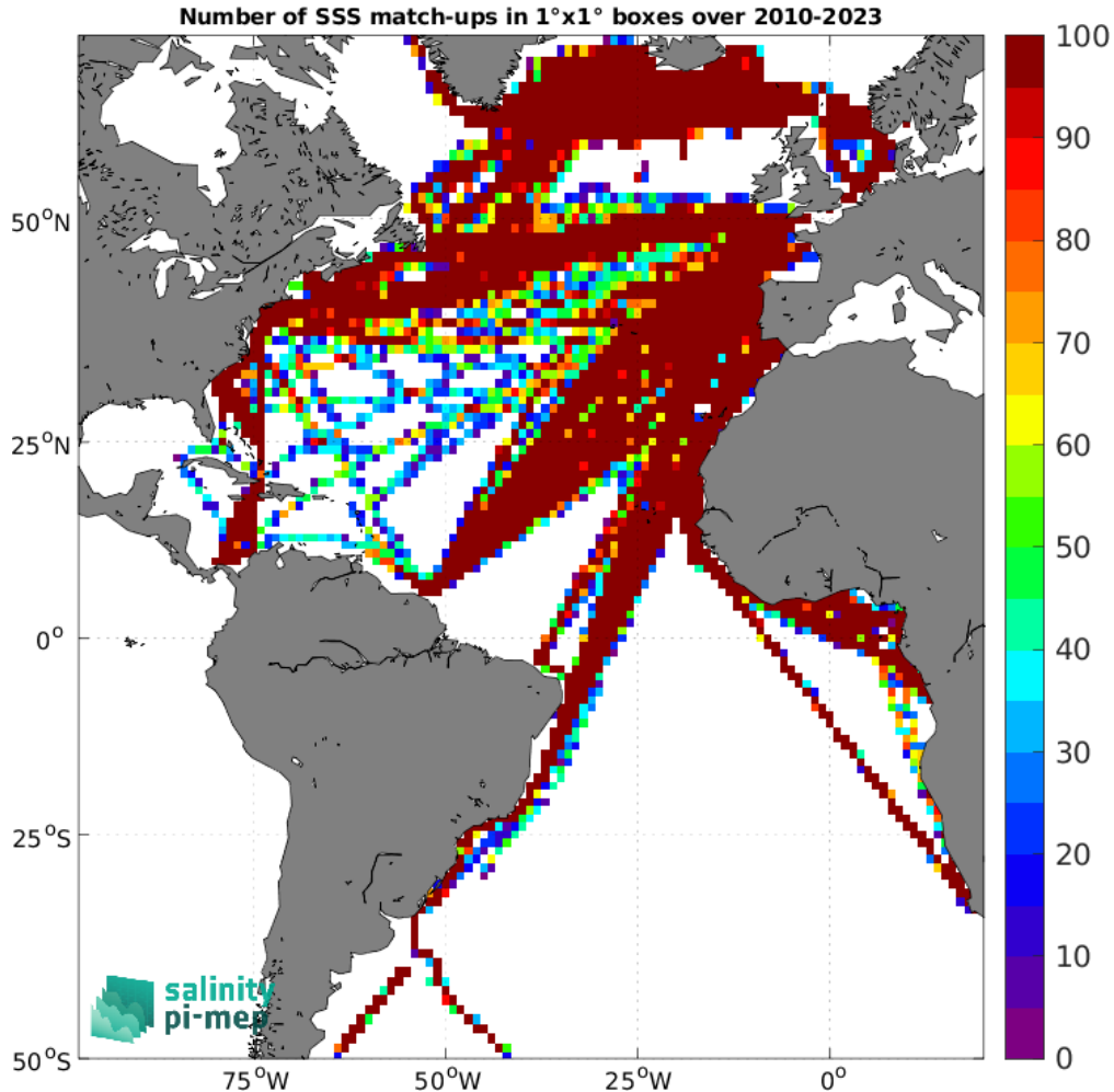
Figure 5: Number of SSS match-ups between TSG (LEGOS-DM) SSS and the SMOS SSS L3 v335 - Monthly - 25 km (CATDS-CPDC) SSS product for the Atlantic Ocean Pi-MEP region over 1^\circ \times 1^\circ boxes and for the full satellite product period.
