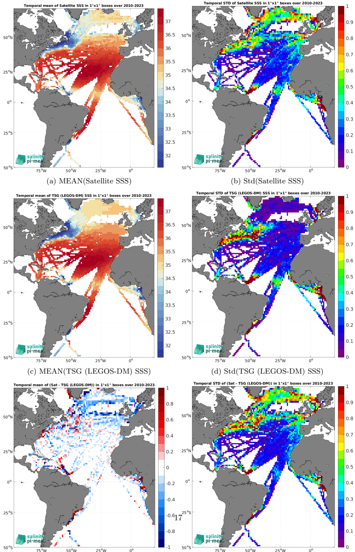
Figure 7: Temporal mean (left) and Std (right) of SSS from SMOS SSS L3 v335 - Monthly - 25 km (CATDS-CPDC) (top), TSG (LEGOS-DM) (middle), and of \Delta SSS (Satellite - TSG (LEGOS-DM)). Only match-up pairs are used to generate these maps.
