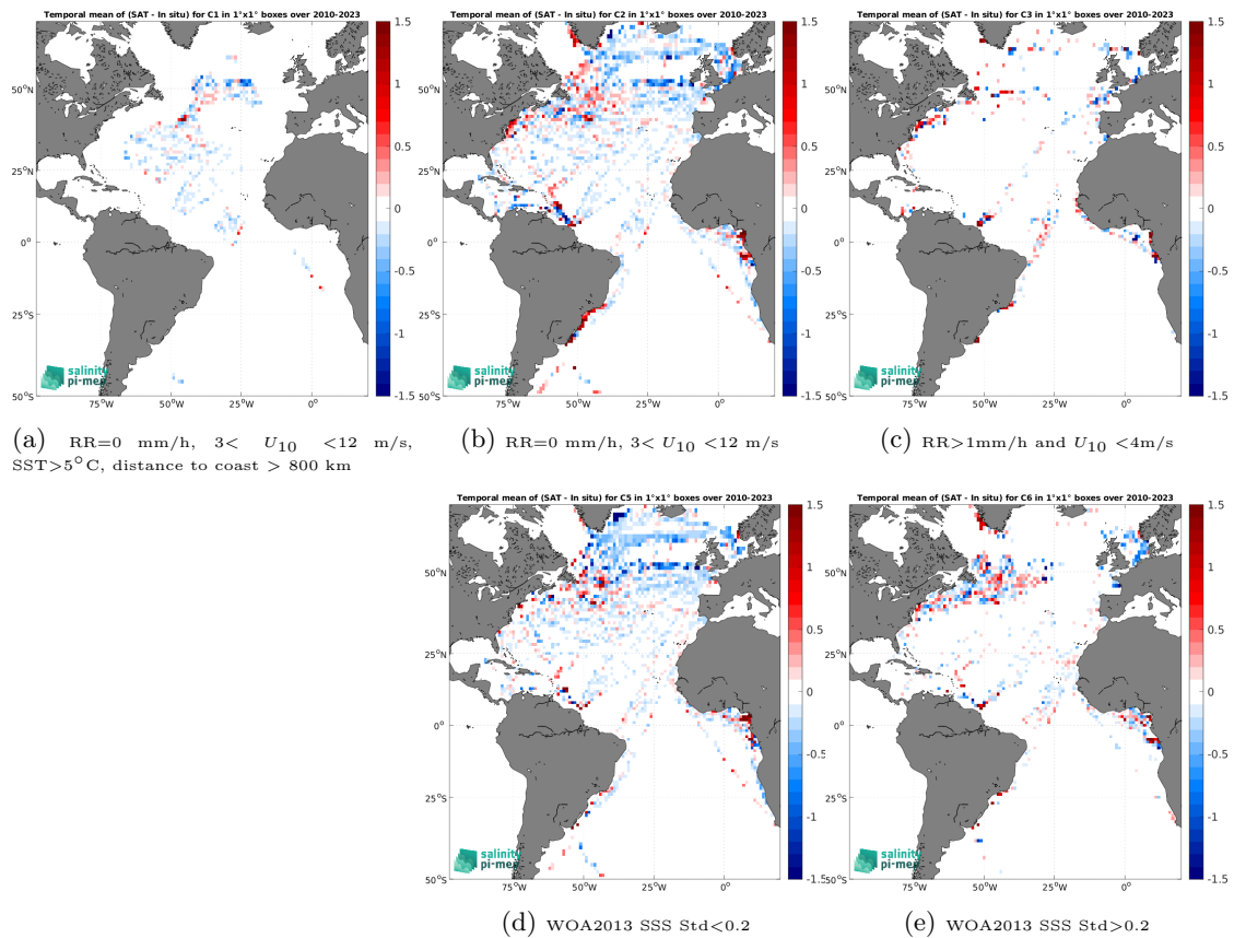
Figure 14: Temporal mean gridded over spatial boxes of size 1^\circ \times 1^\circ of \Delta\text{SSS} (SMOS SSS L3 v335 - Monthly - 25 km (CATDS-CPDC) - TSG (LEGOS-DM)) for 5 different subdatasets corresponding to:RR=0 mm/h, 3 < U_{10} < 12 m/s, SST>5°C, distance to coast > 800 km (a), RR=0 mm/h, 3 < U_{10} < 12 m/s (b), RR>1mm/h and U_{10} < 4 m/s (c), WOA2013 SSS Std<0.2 (d), WOA2013 SSS Std>0.2 (e).
