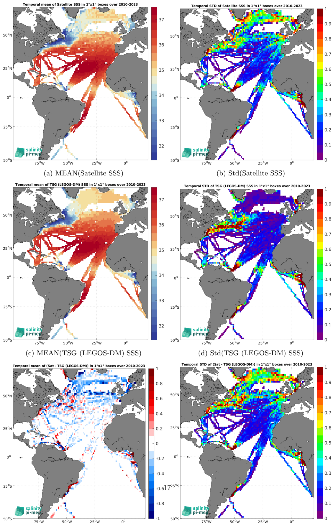
(e) MEAN( \Delta SSS) (Satellite - TSG (LEGOS-DM)) (f) Std( \Delta SSS) (Satellite - TSG (LEGOS-DM)) Figure 6: Temporal mean (left) and Std (right) of SSS from SMOS SSS L3 v335 - Monthly - 25 km (CATDS-CPDC) (top), TSG (LEGOS-DM) (middle), and of \Delta SSS (Satellite - TSG (LEGOS-DM)). Only match-up pairs are used to generate these maps.
