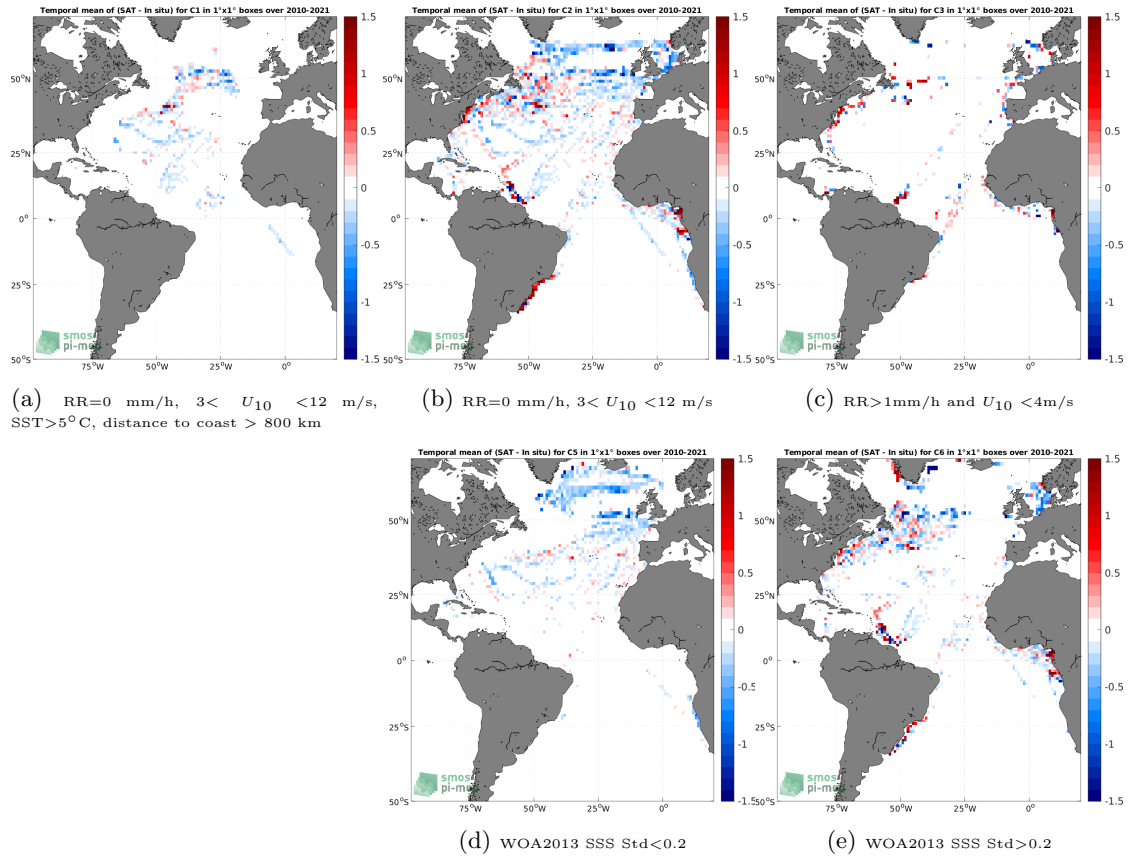
Figure 12: Temporal mean gridded over spatial boxes of size 1^\circ \times 1^\circ of \Delta SSS (SMOS SSS L3 v335 - Monthly - 25 km (CATDS-CPDC) - TSG (LEGOS-DM)) for 5 different subdatasets corresponding to:RR=0 mm/h, 3 < U_{10} < 12 m/s, SST >5^\circ\text{C} , distance to coast > 800 km (a), RR=0 mm/h, 3 < U_{10} < 12 m/s (b), RR >1 mm/h and U_{10} < 4 m/s (c), WOA2013 SSS Std <0.2 (d), WOA2013 SSS Std >0.2 (e).
