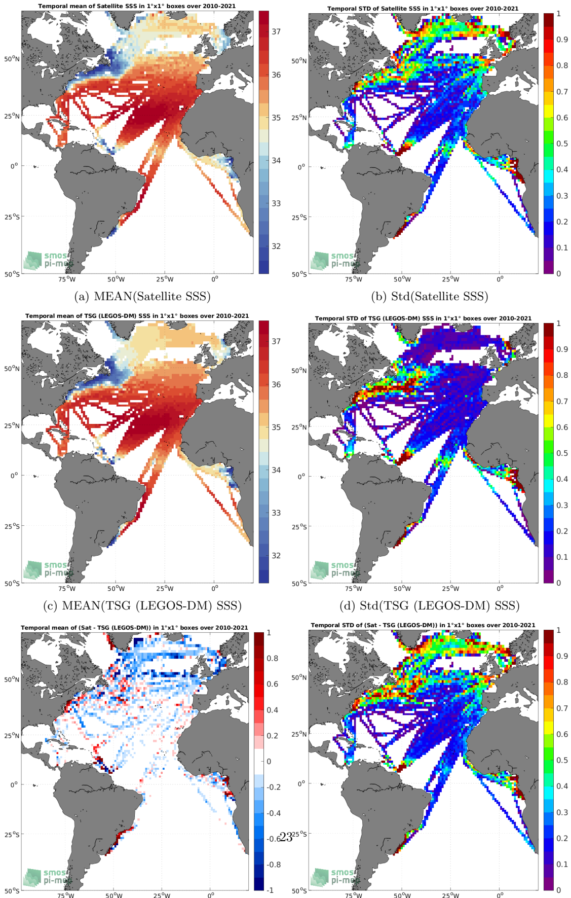
Figure 6: Temporal mean (left) and Std (right) of SSS from SMOS SSS L3 v335 - Monthly - 25 km (CATDS-CPDC) (top), TSG (LEGOS-DM) (middle), and of \Delta SSS (Satellite - TSG (LEGOS-DM)). Only match-up pairs are used to generate these maps.
