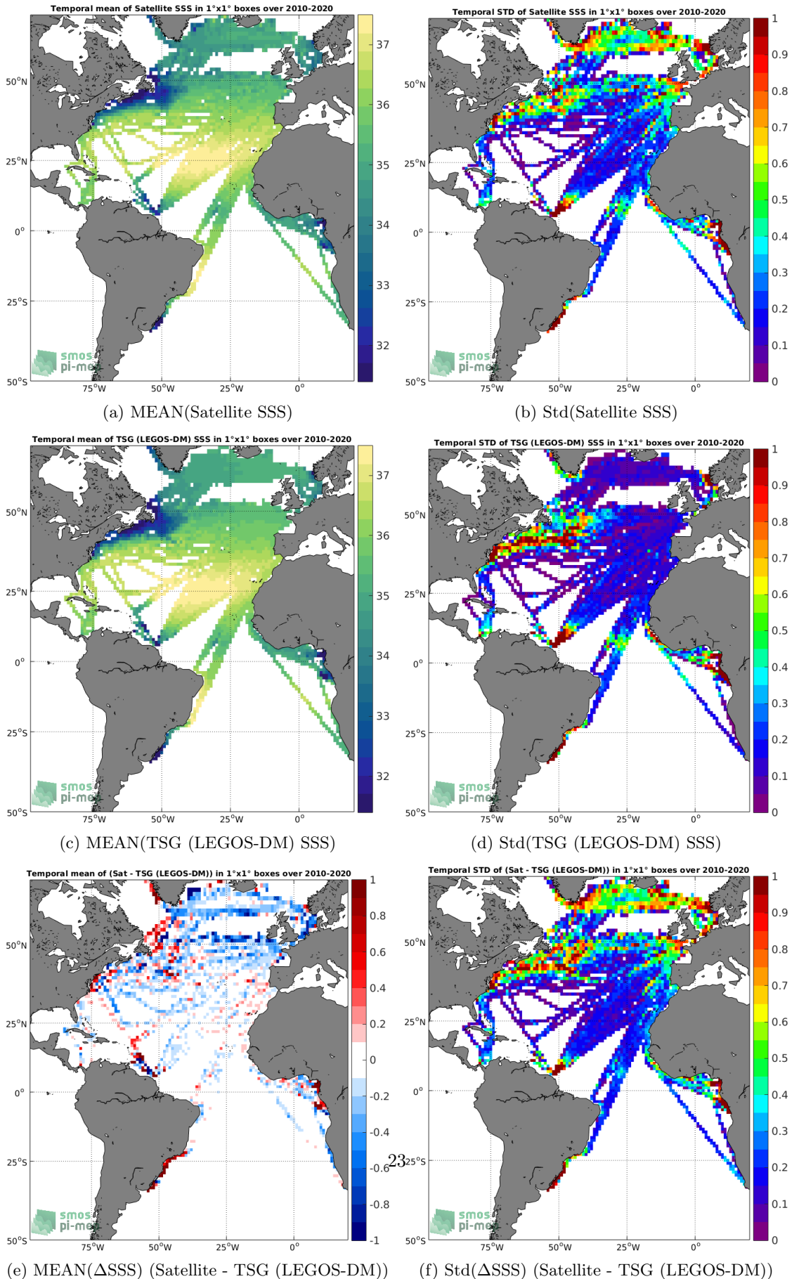
Figure 6: Temporal mean (left) and Std (right) of SSS from SMOS SSS L3 v335 - Monthly - 25 km (CATDS-CPDC) (top), TSG (LEGOS-DM) (middle), and of \Delta SSS (Satellite - TSG (LEGOS-DM)). Only match-up pairs are used to generate these maps.
