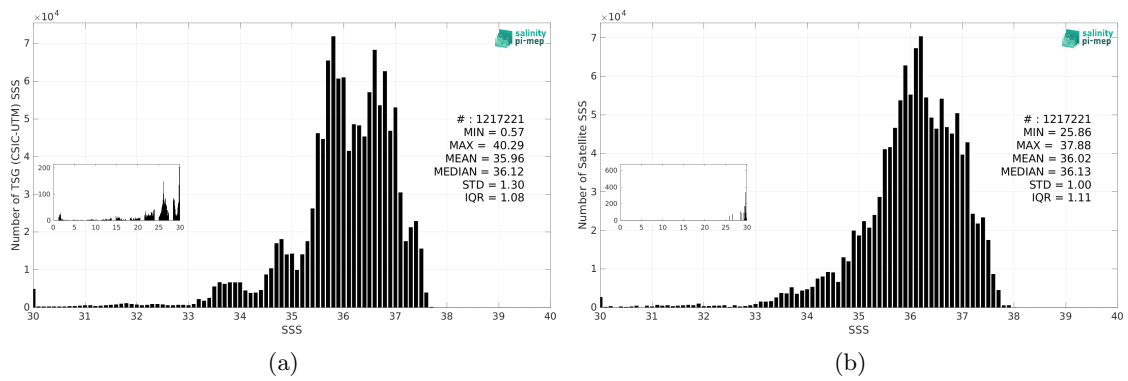
Figure 3: Histograms of SSS from TSG (CSIC-UTM) (a) and SMOS SSS L3 v335 - Monthly - 25 km (CATDS-CPDC) (b) considering all match-up pairs per bins of 0.1 over the Atlantic Ocean Pi-MEP region and for the full satellite product period.
