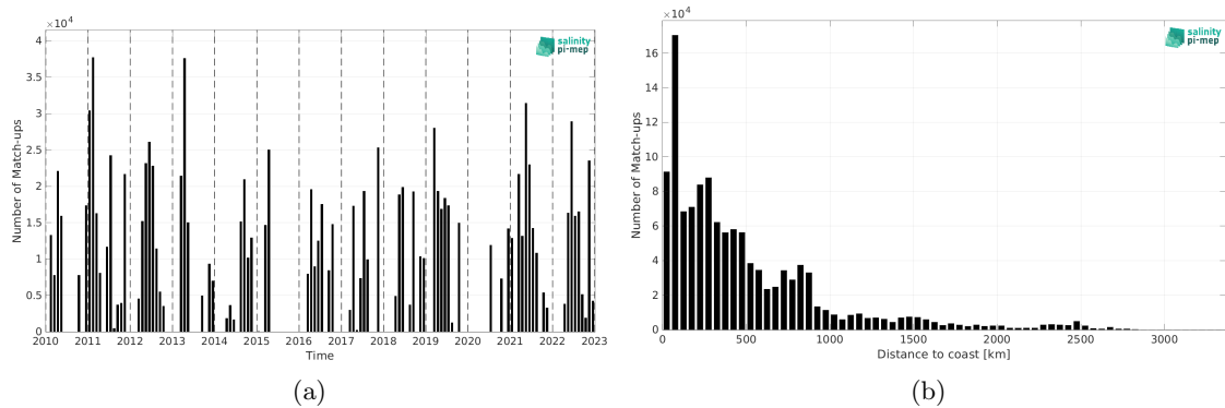
Figure 2: Number of match-ups between TSG (CSIC-UTM) and SMOS SSS L3 v335 - Monthly - 25 km (CATDS-CPDC) SSS as a function of time (a) and as function of the distance to coast (b) over the Atlantic Ocean Pi-MEP region and for the full satellite product period.
