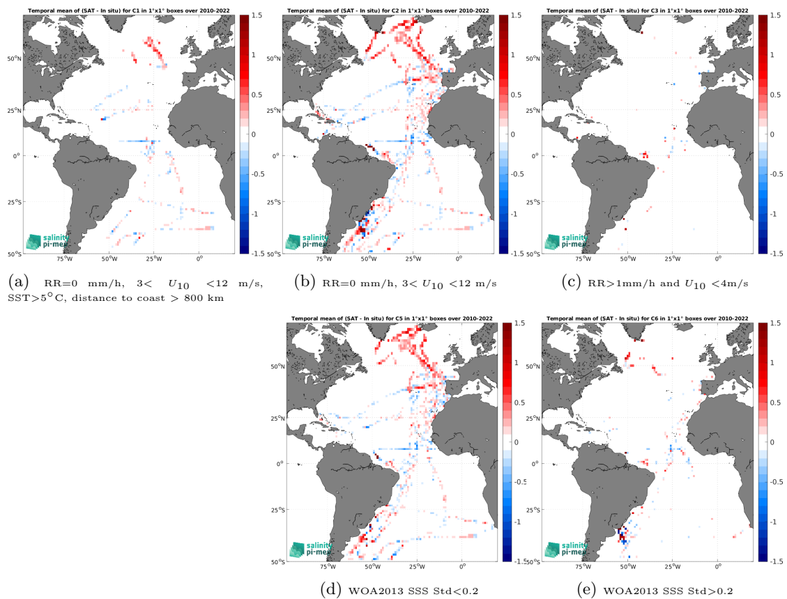
Figure 14: Temporal mean gridded over spatial boxes of size 1^\circ \times 1^\circ of \Delta\text{SSS} (SMOS SSS L3 v335 - Monthly - 25 km (CATDS-CPDC) - TSG (CSIC-UTM)) for 5 different subdatasets corresponding to:RR=0 mm/h, 3 < U_{10} < 12 m/s, SST>5°C, distance to coast > 800 km (a), RR=0 mm/h, 3 < U_{10} < 12 m/s (b), RR>1mm/h and U_{10} < 4 m/s (c), WOA2013 SSS Std<0.2 (d), WOA2013 SSS Std>0.2 (e).
