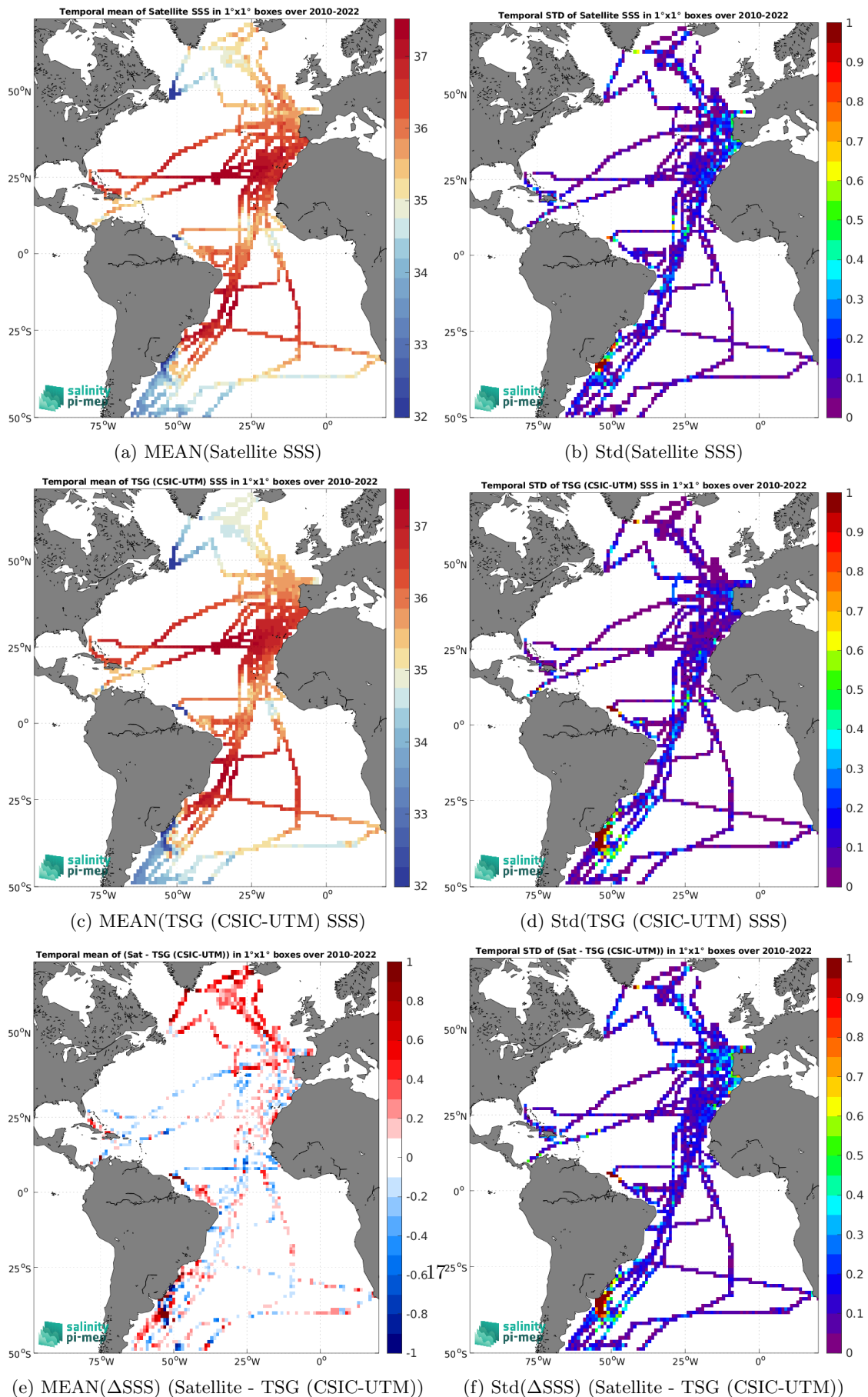
Figure 7: Temporal mean (left) and Std (right) of SSS from SMOS SSS L3 v335 - Monthly - 25 km (CATDS-CPDC) (top), TSG (CSIC-UTM) (middle), and of \Delta SSS (Satellite - TSG (CSIC-UTM)). Only match-up pairs are used to generate these maps.
