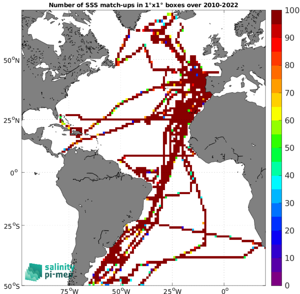
Figure 5: Number of SSS match-ups between TSG (CSIC-UTM) SSS and the SMOS SSS L3 v335 - Monthly - 25 km (CATDS-CPDC) SSS product for the Atlantic Ocean Pi-MEP region over 1^\circ \times 1^\circ boxes and for the full satellite product period.
