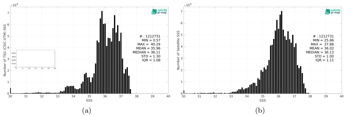
Figure 2: Histograms of SSS from TSG (CSIC-UTM) (a) and SMOS SSS L3 v335 - Monthly - 25 km (CATDS-CPDC) (b) considering all match-up pairs per bins of 0.1 over the Atlantic Ocean Pi-MEP region and for the full satellite product period.
