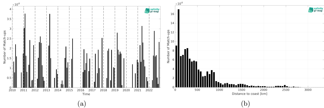
Figure 1: Number of match-ups between TSG (CSIC-UTM) and SMOS SSS L3 v335 - Monthly - 25 km (CATDS-CPDC) SSS as a function of time (a) and as function of the distance to coast (b) over the Atlantic Ocean Pi-MEP region and for the full satellite product period.
