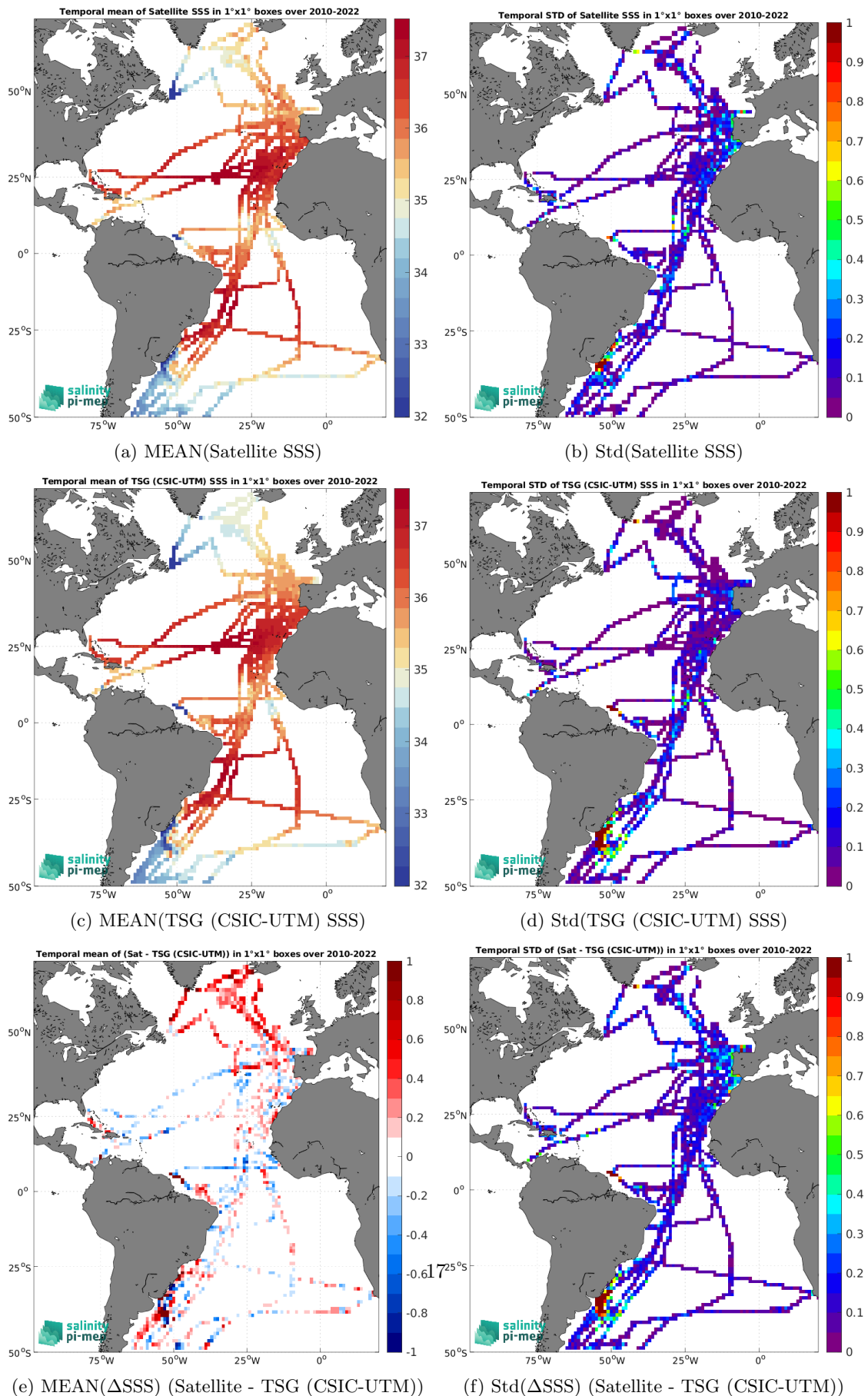
Figure 6: Temporal mean (left) and Std (right) of SSS from SMOS SSS L3 v335 - Monthly - 25 km (CATDS-CPDC) (top), TSG (CSIC-UTM) (middle), and of \Delta SSS (Satellite - TSG (CSIC-UTM)). Only match-up pairs are used to generate these maps.
