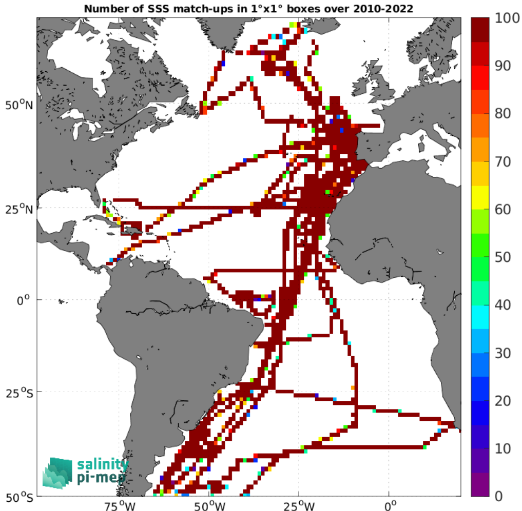
Figure 4: Number of SSS match-ups between TSG (CSIC-UTM) SSS and the SMOS SSS L3 v335 - Monthly - 25 km (CATDS-CPDC) SSS product for the Atlantic Ocean Pi-MEP region over 1^\circ \times 1^\circ boxes and for the full satellite product period.
