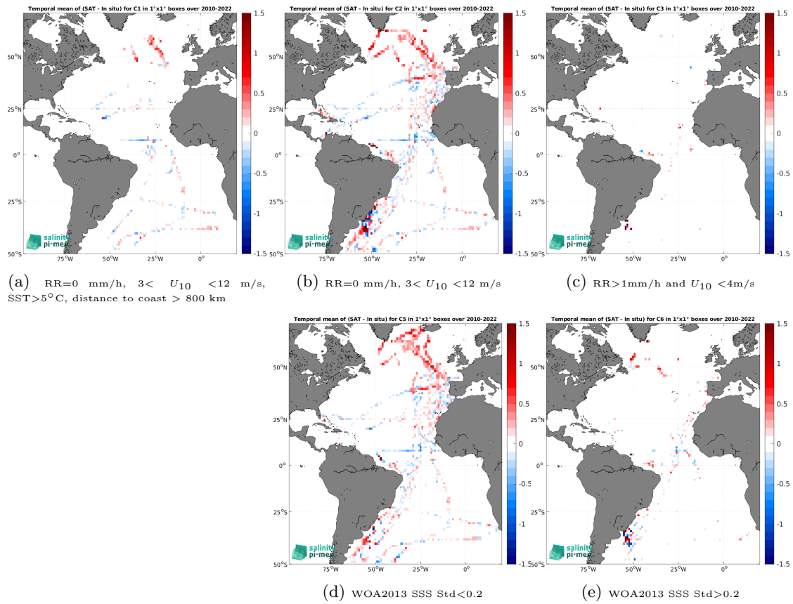
Figure 12: Temporal mean gridded over spatial boxes of size 1^\circ \times 1^\circ of \Delta SSS (SMOS SSS L3 v335 - Monthly - 25 km (CATDS-CPDC) - TSG (CSIC-UTM)) for 5 different subdatasets corresponding to:RR=0 mm/h, 3 < U_{10} < 12 m/s, SST >5^\circ\text{C} , distance to coast > 800 km (a), RR=0 mm/h, 3 < U_{10} < 12 m/s (b), RR >1 mm/h and U_{10} < 4 m/s (c), WOA2013 SSS Std <0.2 (d), WOA2013 SSS Std >0.2 (e).
