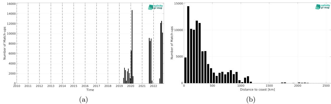
Figure 2: Number of match-ups between Saildrone and SMOS SSS L3 v335 - Monthly - 25 km (CATDS-CPDC) SSS as a function of time (a) and as function of the distance to coast (b) over the Atlantic Ocean Pi-MEP region and for the full satellite product period.
