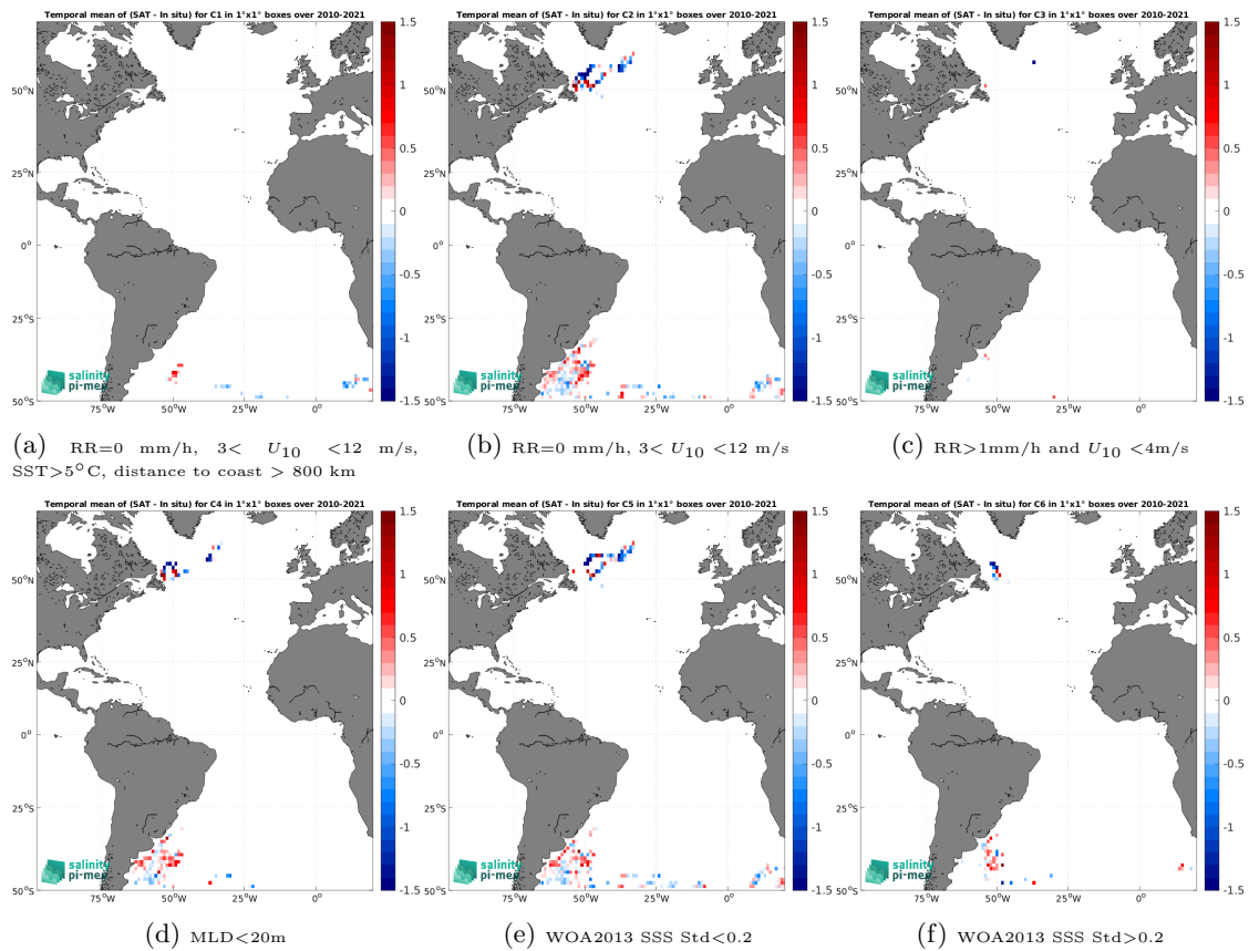
Figure 14: Temporal mean gridded over spatial boxes of size 1^\circ \times 1^\circ of \Delta SSS (SMOS SSS L3 v335 - Monthly - 25 km (CATDS-CPDC) - Marine mammals) for 6 different subdatasets corresponding to:RR=0 mm/h, 3 < U_{10} < 12 m/s, SST>5°C, distance to coast > 800 km (a), RR=0 mm/h, 3 < U_{10} < 12 m/s (b), RR>1mm/h and U_{10} < 4 m/s (c),MLD<20m (d),WOA2013 SSS Std<0.2 (e),WOA2013 SSS Std>0.2 (f).
