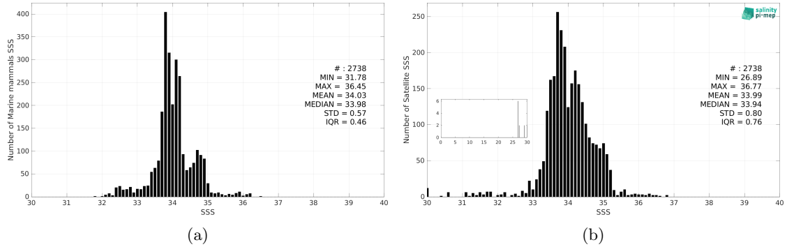
Figure 3: Histograms of SSS from Marine mammals (a) and SMOS SSS L3 v335 - Monthly - 25 km (CATDS-CPDC) (b) considering all match-up pairs per bins of 0.1 over the Atlantic Ocean Pi-MEP region and for the full satellite product period.
