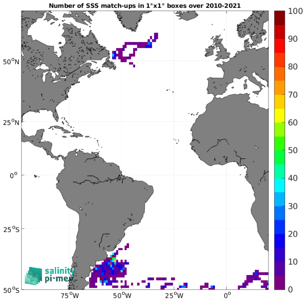
Figure 5: Number of SSS match-ups between Marine mammals SSS and the SMOS SSS L3 v335 - Monthly - 25 km (CATDS-CPDC) SSS product for the Atlantic Ocean Pi-MEP region over 1^\circ \times 1^\circ boxes and for the full satellite product period.
