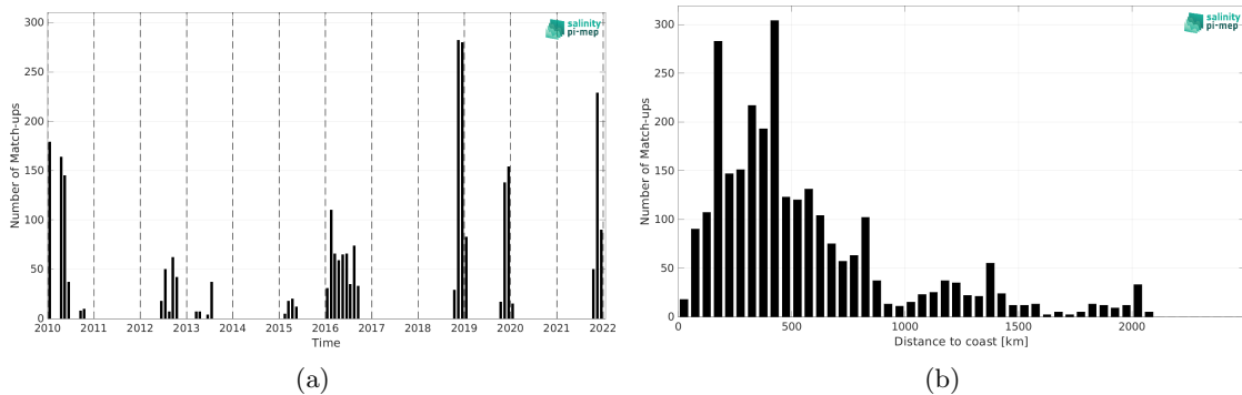
Figure 2: Number of match-ups between Marine mammals and SMOS SSS L3 v335 - Monthly - 25 km (CATDS-CPDC) SSS as a function of time (a) and as function of the distance to coast (b) over the Atlantic Ocean Pi-MEP region and for the full satellite product period.
