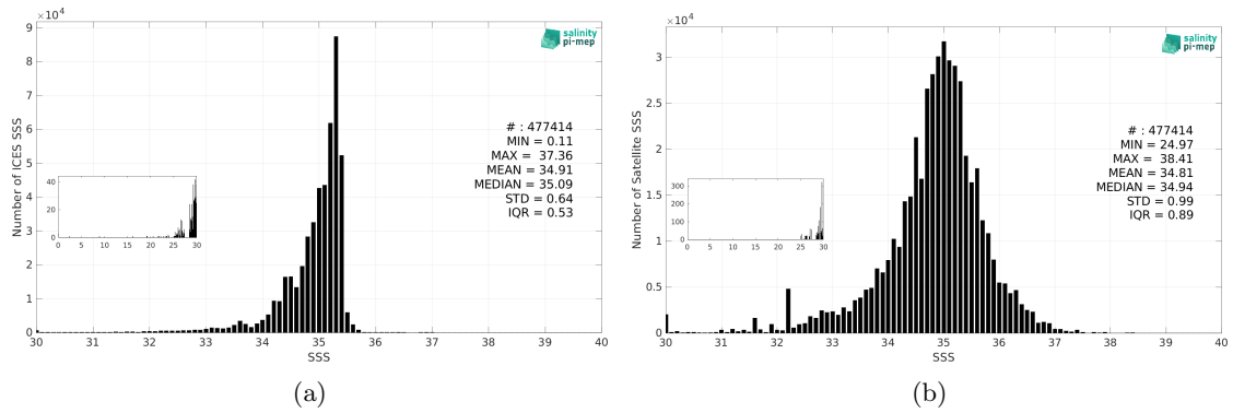
Figure 3: Histograms of SSS from ICES (a) and SMOS SSS L3 v335 - Monthly - 25 km (CATDS-CPDC) (b) considering all match-up pairs per bins of 0.1 over the Atlantic Ocean Pi-MEP region and for the full satellite product period.
