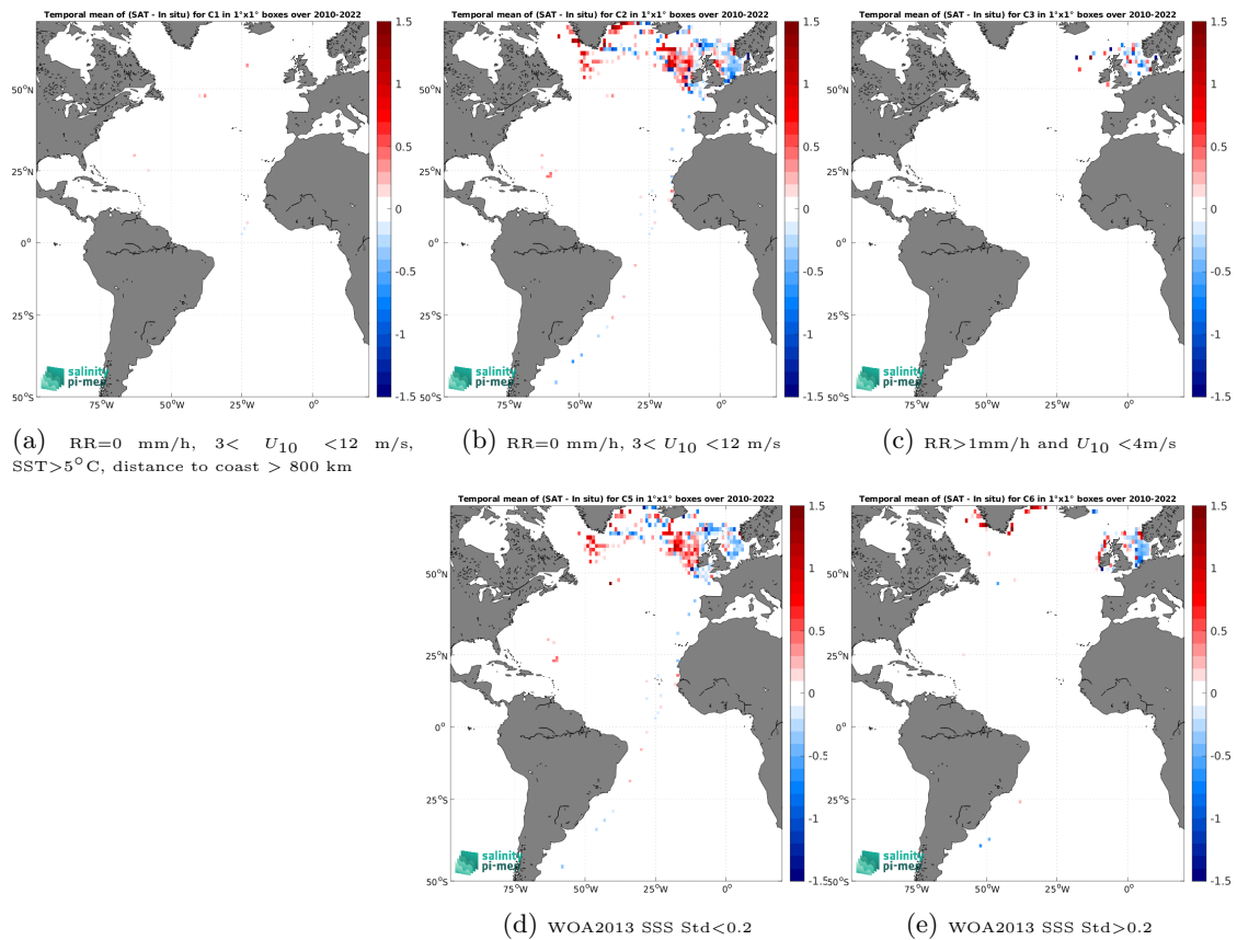
Figure 14: Temporal mean gridded over spatial boxes of size 1^\circ \times 1^\circ of \Delta\text{SSS} (SMOS SSS L3 v335 - Monthly - 25 km (CATDS-CPDC) - ICES) for 5 different subdatasets corresponding to:RR=0 mm/h, 3 < U_{10} < 12 m/s, SST>5°C, distance to coast > 800 km (a), RR=0 mm/h, 3 < U_{10} < 12 m/s (b), RR>1mm/h and U_{10} < 4 m/s (c), WOA2013 SSS Std<0.2 (d), WOA2013 SSS Std>0.2 (e).
