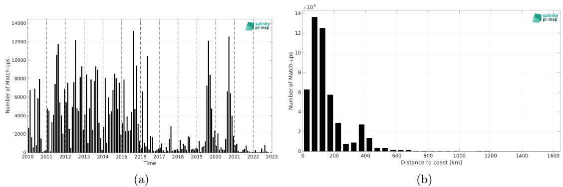
Figure 2: Number of match-ups between ICES and SMOS SSS L3 v335 - Monthly - 25 km (CATDS-CPDC) SSS as a function of time (a) and as function of the distance to coast (b) over the Atlantic Ocean Pi-MEP region and for the full satellite product period.
