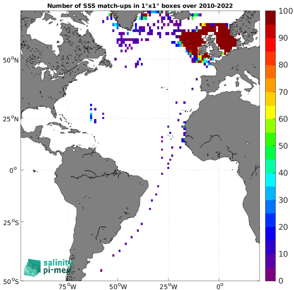
Figure 5: Number of SSS match-ups between ICES SSS and the SMOS SSS L3 v335 - Monthly - 25 km (CATDS-CPDC) SSS product for the Atlantic Ocean Pi-MEP region over 1^\circ \times 1^\circ boxes and for the full satellite product period.
