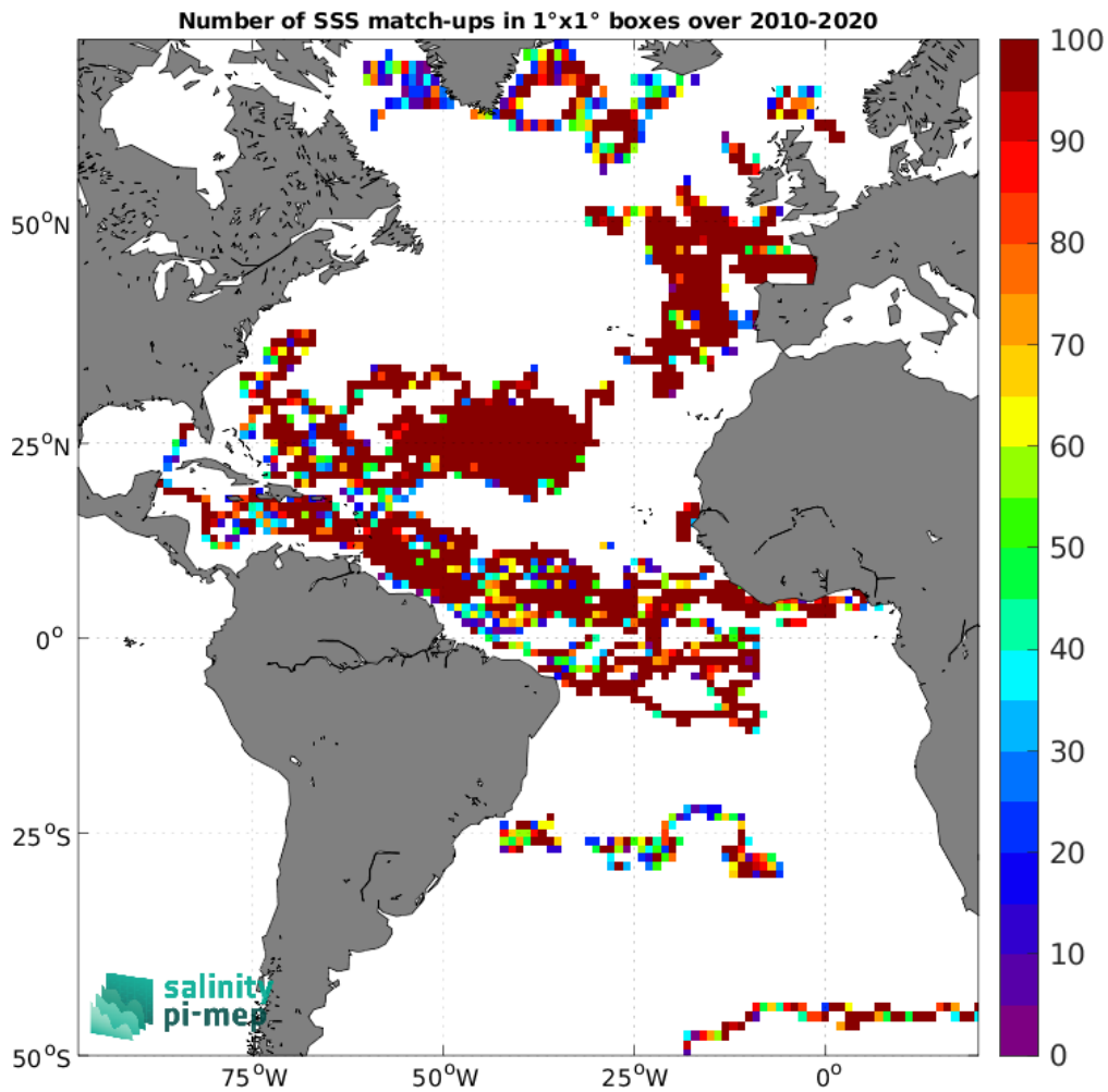
Figure 3: Number of SSS match-ups between Surface drifters SSS and the SMOS SSS L3 v335 - Monthly - 25 km (CATDS-CPDC) SSS product for the Atlantic Ocean Pi-MEP region over 1°×1° boxes and for the full satellite product period.
