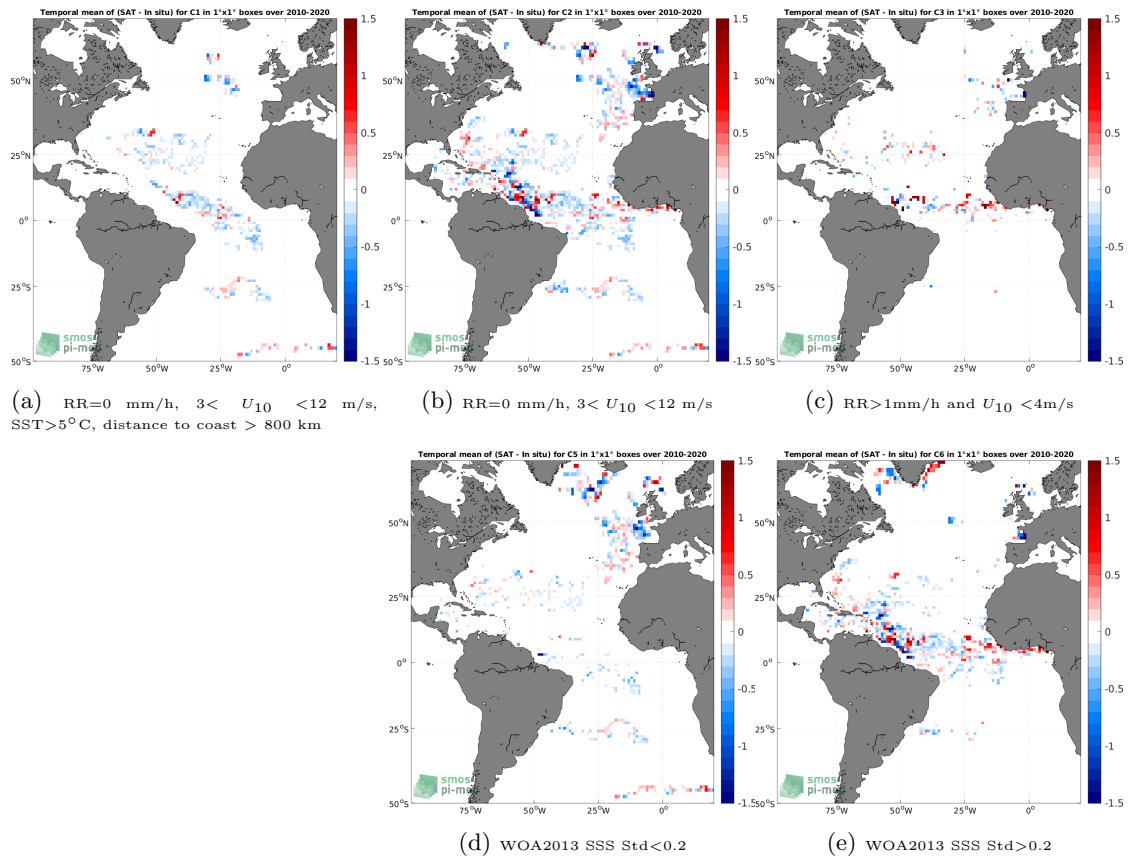
Figure 11: Temporal mean gridded over spatial boxes of size 1^\circ \times 1^\circ of \Delta SSS (SMOS SSS L3 v335 - Monthly - 25 km (CATDS-CPDC) - Surface drifters) for 5 different subdatasets corresponding to:RR=0 mm/h, 3 < U_{10} < 12 m/s, SST >5^\circ\text{C} , distance to coast > 800 km (a), RR=0 mm/h, 3 < U_{10} < 12 m/s (b), RR >1 mm/h and U_{10} < 4 m/s (c), WOA2013 SSS Std <0.2 (d), WOA2013 SSS Std >0.2 (e).
