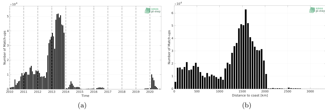
Figure 1: Number of match-ups between Surface drifters and SMOS SSS L3 v335 - Monthly - 25 km (CATDS-CPDC) SSS as a function of time (a) and as function of the distance to coast (b) over the Atlantic Ocean Pi-MEP region and for the full satellite product period.
