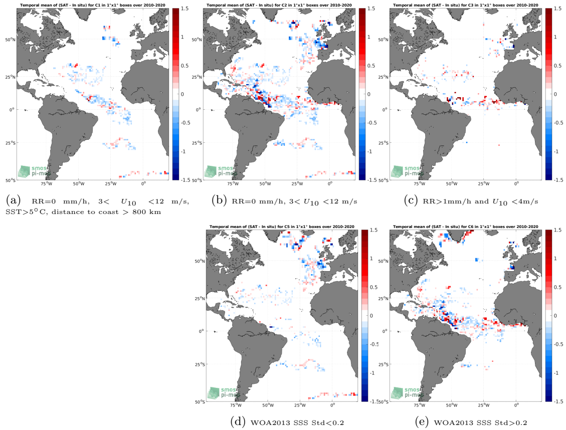
Figure 11: Temporal mean gridded over spatial boxes of size 1^\circ \times 1^\circ of \Delta\text{SSS} (SMOS SSS L3 v335 - Monthly - 25 km (CATDS-CPDC) - Surface drifters) for 5 different subdatasets corresponding to:RR=0 mm/h, 3 < U_{10} < 12 m/s, SST >5^\circ\text{C} , distance to coast > 800 km (a), RR=0 mm/h, 3 < U_{10} < 12 m/s (b), RR >1 mm/h and U_{10} < 4 m/s (c), WOA2013 SSS Std <0.2 (d), WOA2013 SSS Std >0.2 (e).
