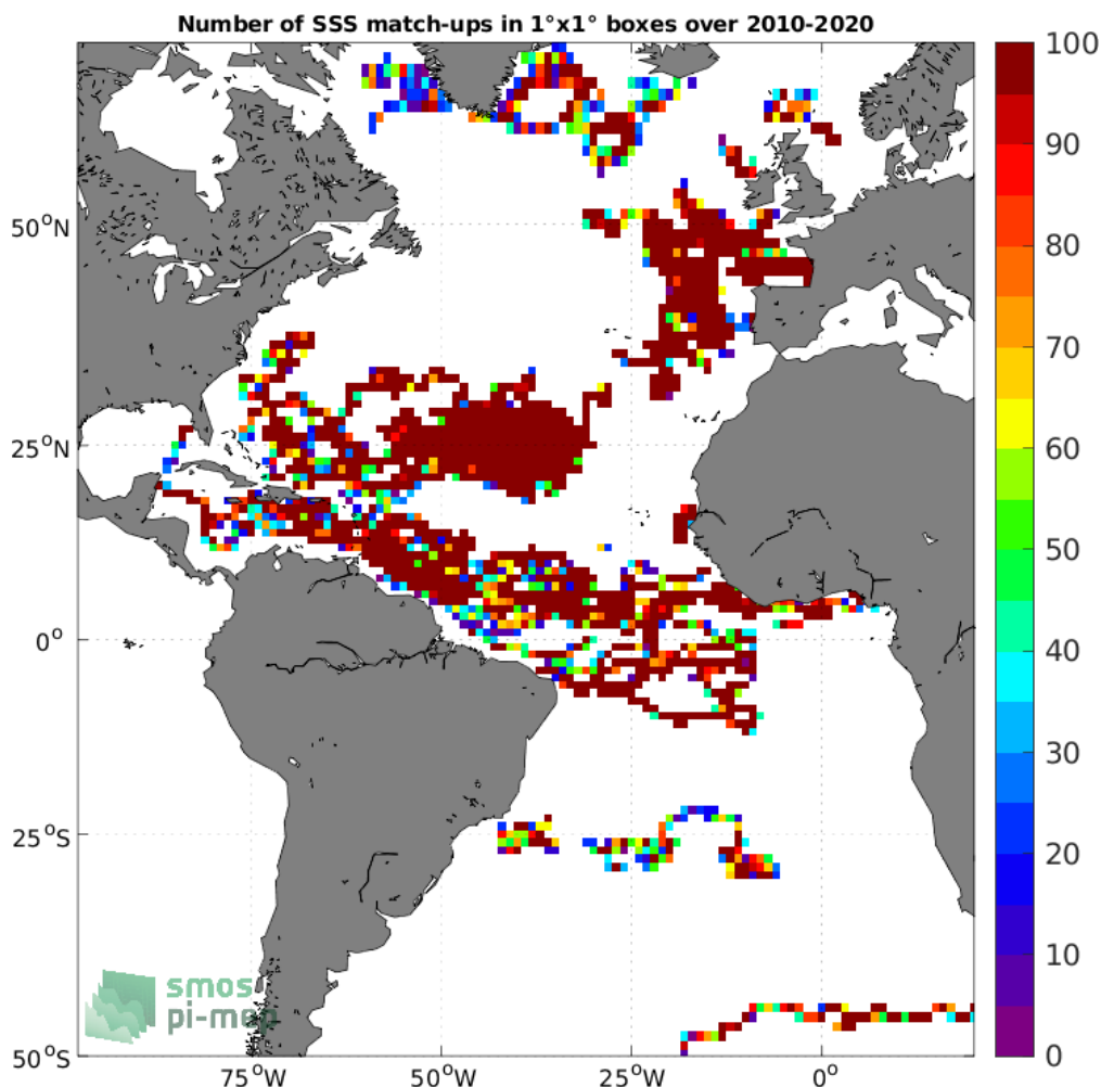
Figure 3: Number of SSS match-ups between Surface drifters SSS and the SMOS SSS L3 v335 - Monthly - 25 km (CATDS-CPDC) SSS product for the Atlantic Ocean Pi-MEP region over 1^\circ \times 1^\circ boxes and for the full satellite product period.
