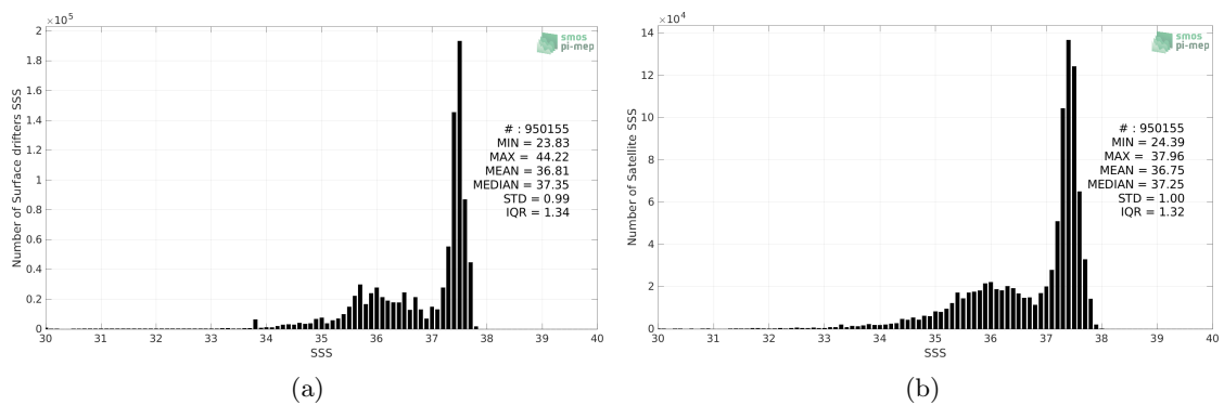
Figure 2: Histograms of SSS from Surface drifters (a) and SMOS SSS L3 v335 - Monthly - 25 km (CATDS-CPDC) (b) considering all match-up pairs per bins of 0.1 over the Atlantic Ocean Pi-MEP region and for the full satellite product period.
