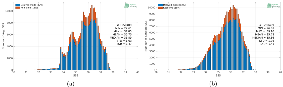
Figure 2: Histograms of SSS from Argo (a) and SMOS SSS L3 v335 - Monthly - 25 km (CATDS-CPDC) (b) considering all match-up pairs per bins of 0.1 over the Atlantic Ocean Pi-MEP region and for the full satellite product period.
