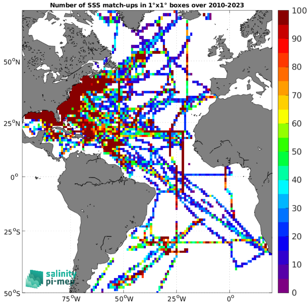
Figure 4: Number of SSS match-ups between TSG (SAMOS) SSS and the SMOS SSS L3 v335 - 10 Days - 25 km (CATDS-CPDC) SSS product for the Atlantic Ocean Pi-MEP region over 1^\circ \times 1^\circ boxes and for the full satellite product period.
