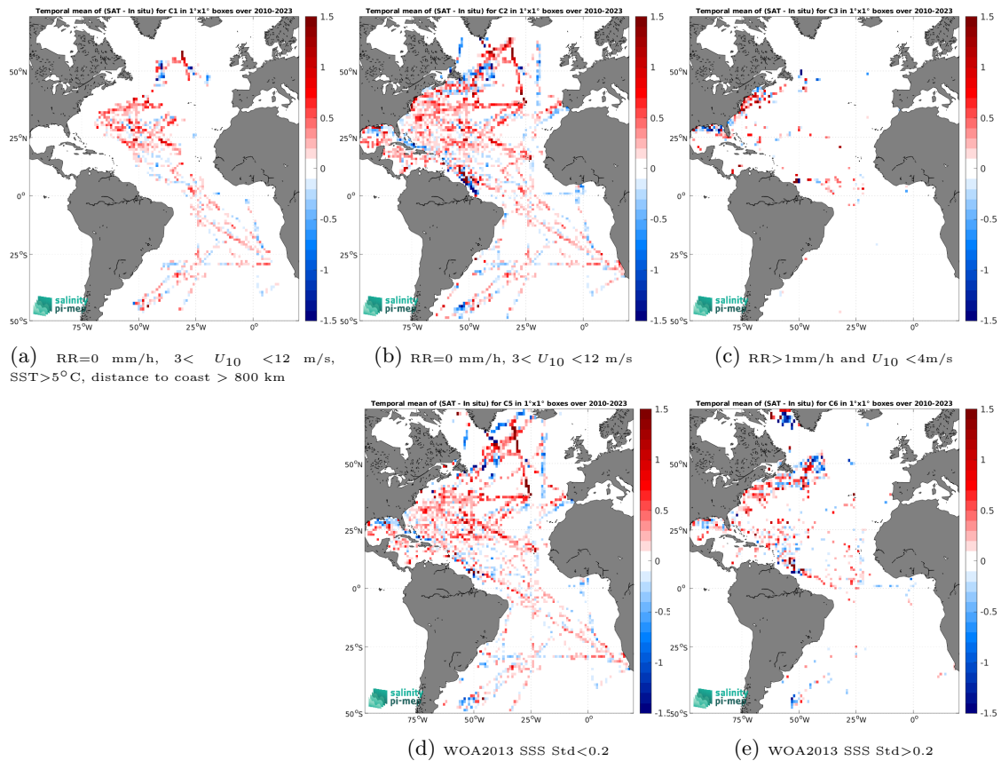
Figure 12: Temporal mean gridded over spatial boxes of size 1^\circ \times 1^\circ of \Delta\text{SSS} (SMOS SSS L3 v335 - 10 Days - 25 km (CATDS-CPDC) - TSG (SAMOS)) for 5 different subdatasets corresponding to:RR=0 mm/h, 3 < U_{10} < 12 m/s, SST >5^\circ\text{C} , distance to coast > 800 km (a), RR=0 mm/h, 3 < U_{10} < 12 m/s (b), RR >1 mm/h and U_{10} < 4 m/s (c), WOA2013 SSS Std <0.2 (d), WOA2013 SSS Std >0.2 (e).
