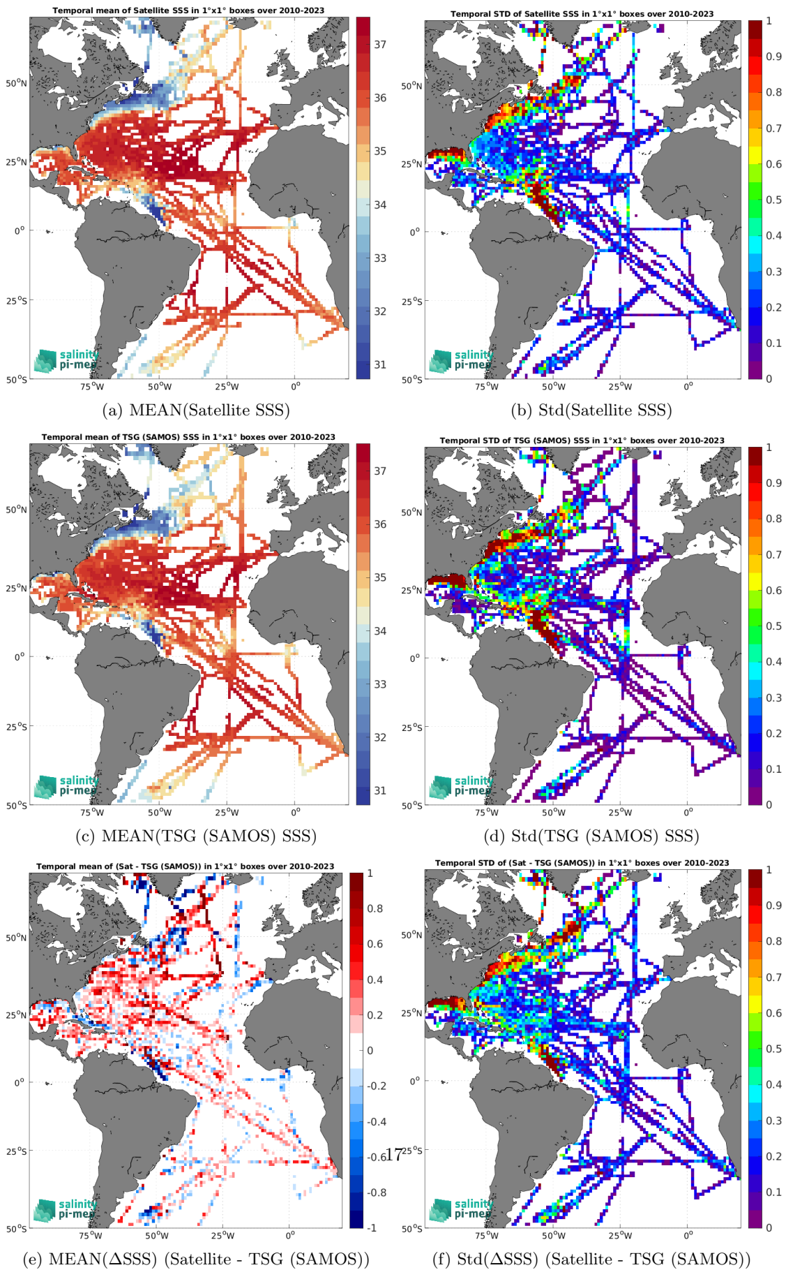
Figure 6: Temporal mean (left) and Std (right) of SSS from SMOS SSS L3 v335 - 10 Days - 25 km (CATDS-CPDC) (top), TSG (SAMOS) (middle), and of \Delta SSS (Satellite - TSG (SAMOS)). Only match-up pairs are used to generate these maps.
