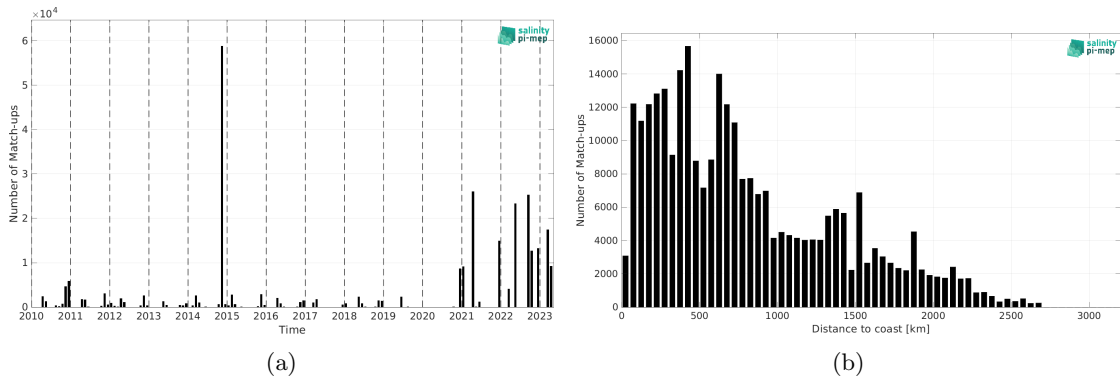
Figure 2: Number of match-ups between TSG (Polarstern) and SMOS SSS L3 v335 - 10 Days - 25 km (CATDS-CPDC) SSS as a function of time (a) and as function of the distance to coast (b) over the Atlantic Ocean Pi-MEP region and for the full satellite product period.
