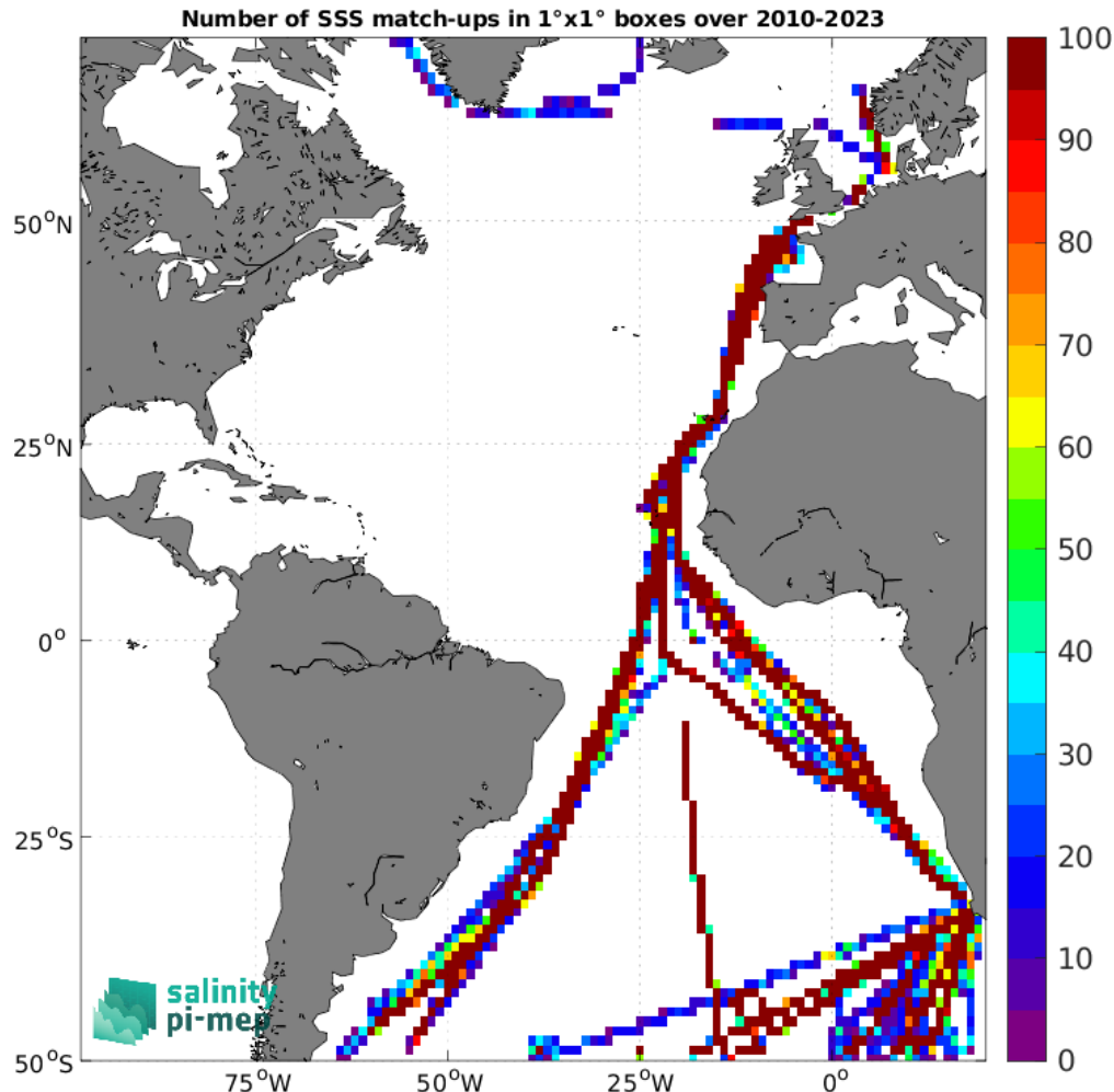
Figure 5: Number of SSS match-ups between TSG (Polarstern) SSS and the SMOS SSS L3 v335 - 10 Days - 25 km (CATDS-CPDC) SSS product for the Atlantic Ocean Pi-MEP region over 1^\circ \times 1^\circ boxes and for the full satellite product period.
