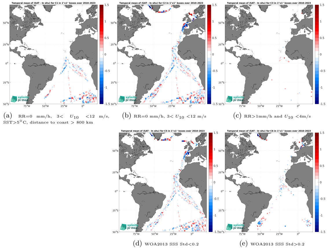
Figure 14: Temporal mean gridded over spatial boxes of size 1^\circ \times 1^\circ of \Delta\text{SSS} (SMOS SSS L3 v335 - 10 Days - 25 km (CATDS-CPDC) - TSG (Polarstern)) for 5 different subdatasets corresponding to:RR=0 mm/h, 3 < U_{10} < 12 m/s, SST>5°C, distance to coast > 800 km (a), RR=0 mm/h, 3 < U_{10} < 12 m/s (b), RR>1mm/h and U_{10} < 4 m/s (c), WOA2013 SSS Std<0.2 (d), WOA2013 SSS Std>0.2 (e).
