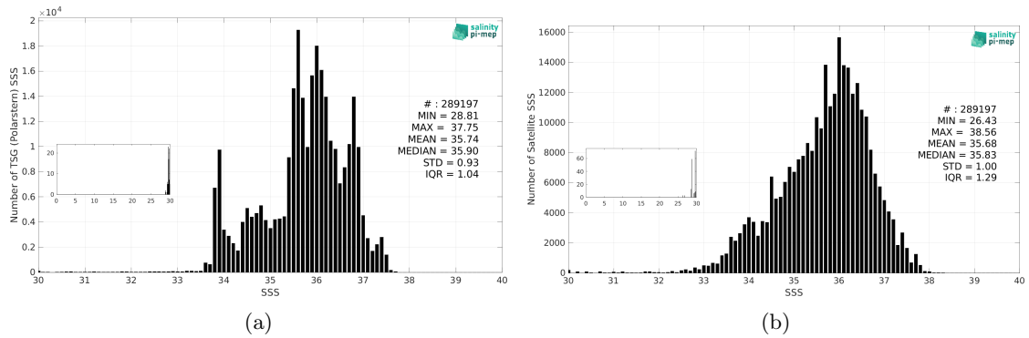
Figure 3: Histograms of SSS from TSG (Polarstern) (a) and SMOS SSS L3 v335 - 10 Days - 25 km (CATDS-CPDC) (b) considering all match-up pairs per bins of 0.1 over the Atlantic Ocean Pi-MEP region and for the full satellite product period.
