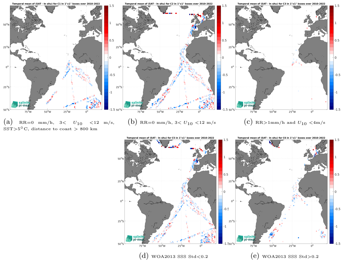
Figure 12: Temporal mean gridded over spatial boxes of size 1^\circ \times 1^\circ of \Delta\text{SSS} (SMOS SSS L3 v335 - 10 Days - 25 km (CATDS-CPDC) - TSG (Polarstern)) for 5 different subdatasets corresponding to:RR=0 mm/h, 3 < U_{10} < 12 m/s, SST >5^\circ\text{C} , distance to coast > 800 km (a), RR=0 mm/h, 3 < U_{10} < 12 m/s (b), RR >1 mm/h and U_{10} < 4 m/s (c), WOA2013 SSS Std <0.2 (d), WOA2013 SSS Std >0.2 (e).
