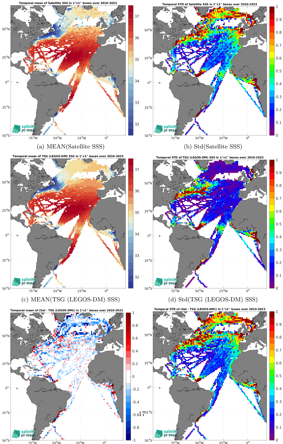
Figure 7: Temporal mean (left) and Std (right) of SSS from SMOS SSS L3 v335 - 10 Days - 25 km (CATDS-CPDC) (top), TSG (LEGOS-DM) (middle), and of \Delta SSS (Satellite - TSG (LEGOS-DM)). Only match-up pairs are used to generate these maps.
