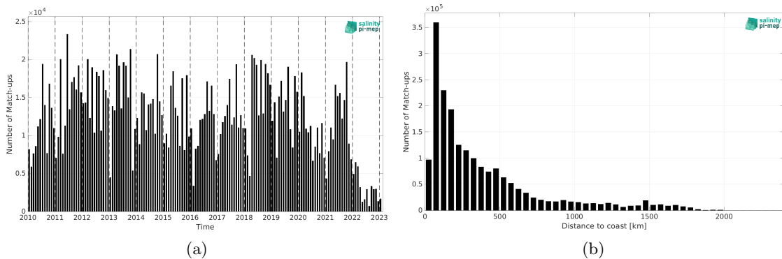
Figure 1: Number of match-ups between TSG (LEGOS-DM) and SMOS SSS L3 v335 - 10 Days - 25 km (CATDS-CPDC) SSS as a function of time (a) and as function of the distance to coast (b) over the Atlantic Ocean Pi-MEP region and for the full satellite product period.
