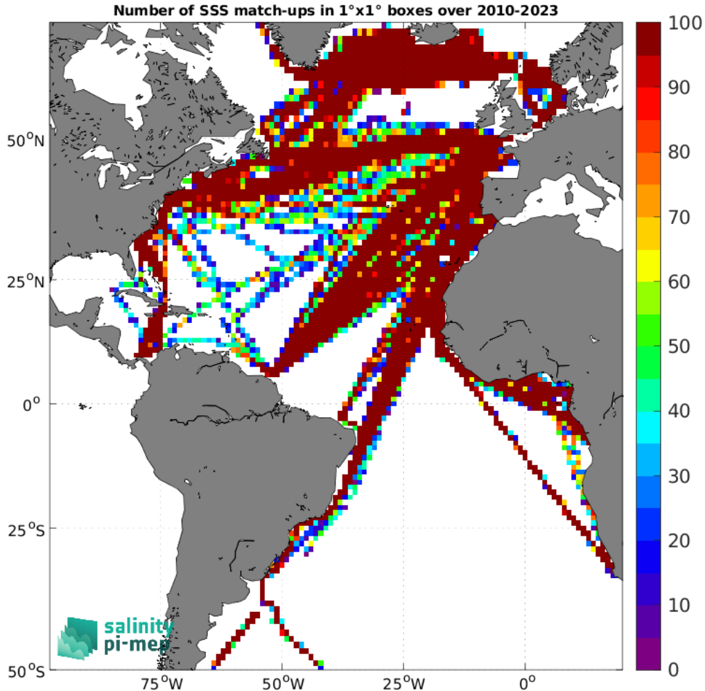
Figure 4: Number of SSS match-ups between TSG (LEGOS-DM) SSS and the SMOS SSS L3 v335 - 10 Days - 25 km (CATDS-CPDC) SSS product for the Atlantic Ocean Pi-MEP region over 1^\circ \times 1^\circ boxes and for the full satellite product period.
