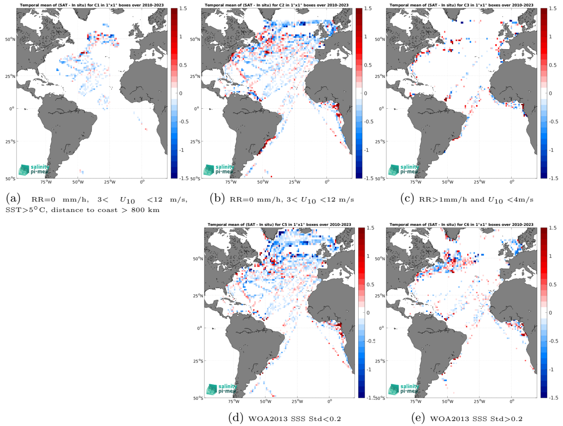
Figure 12: Temporal mean gridded over spatial boxes of size 1^\circ \times 1^\circ of \Delta SSS (SMOS SSS L3 v335 - 10 Days - 25 km (CATDS-CPDC) - TSG (LEGOS-DM)) for 5 different subdatasets corresponding to:RR=0 mm/h, 3 < U_{10} < 12 m/s, SST >5^\circ\text{C} , distance to coast > 800 km (a), RR=0 mm/h, 3 < U_{10} < 12 m/s (b), RR >1 mm/h and U_{10} < 4 m/s (c), WOA2013 SSS Std <0.2 (d), WOA2013 SSS Std >0.2 (e).
