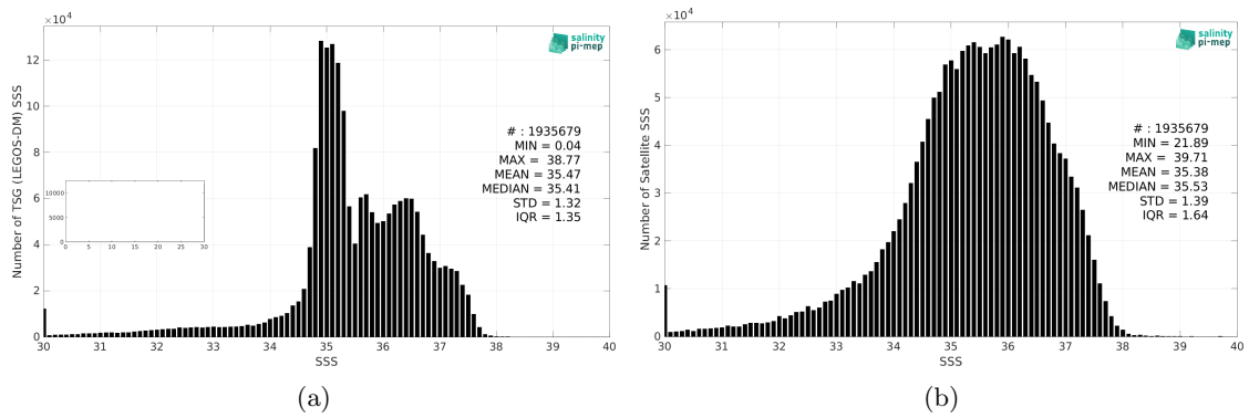
Figure 2: Histograms of SSS from TSG (LEGOS-DM) (a) and SMOS SSS L3 v335 - 10 Days - 25 km (CATDS-CPDC) (b) considering all match-up pairs per bins of 0.1 over the Atlantic Ocean Pi-MEP region and for the full satellite product period.
