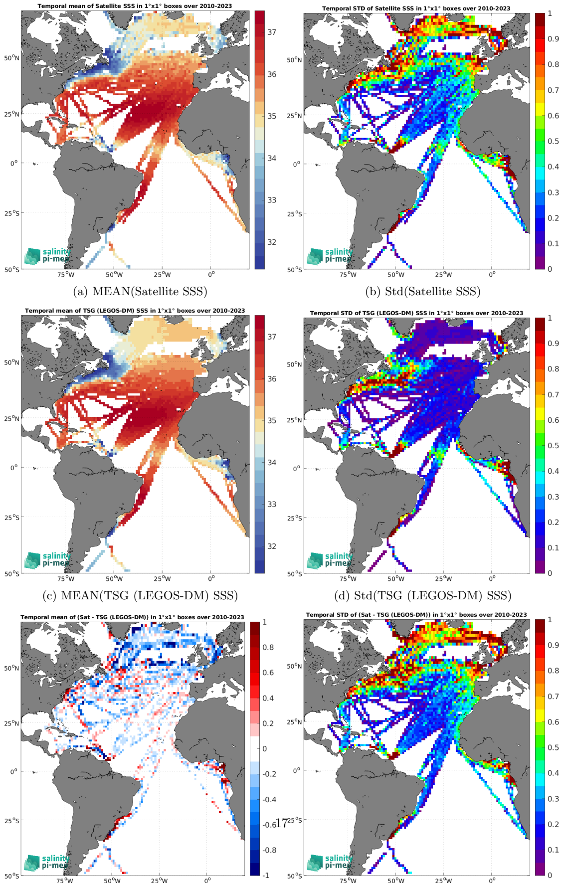
(e) MEAN( \Delta SSS) (Satellite - TSG (LEGOS-DM)) (f) Std( \Delta SSS) (Satellite - TSG (LEGOS-DM)) Figure 6: Temporal mean (left) and Std (right) of SSS from SMOS SSS L3 v335 - 10 Days - 25 km (CATDS-CPDC) (top), TSG (LEGOS-DM) (middle), and of \Delta SSS (Satellite - TSG (LEGOS-DM)). Only match-up pairs are used to generate these maps.
