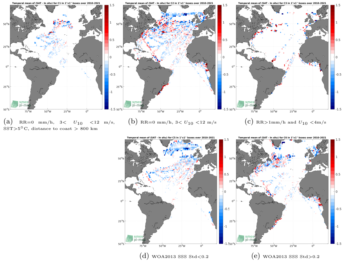
Figure 12: Temporal mean gridded over spatial boxes of size 1^\circ \times 1^\circ of \Delta SSS (SMOS SSS L3 v335 - 10 Days - 25 km (CATDS-CPDC) - TSG (LEGOS-DM)) for 5 different subdatasets corresponding to:RR=0 mm/h, 3 < U_{10} < 12 m/s, SST >5^\circ\text{C} , distance to coast > 800 km (a), RR=0 mm/h, 3 < U_{10} < 12 m/s (b), RR >1 mm/h and U_{10} < 4 m/s (c), WOA2013 SSS Std <0.2 (d), WOA2013 SSS Std >0.2 (e).
